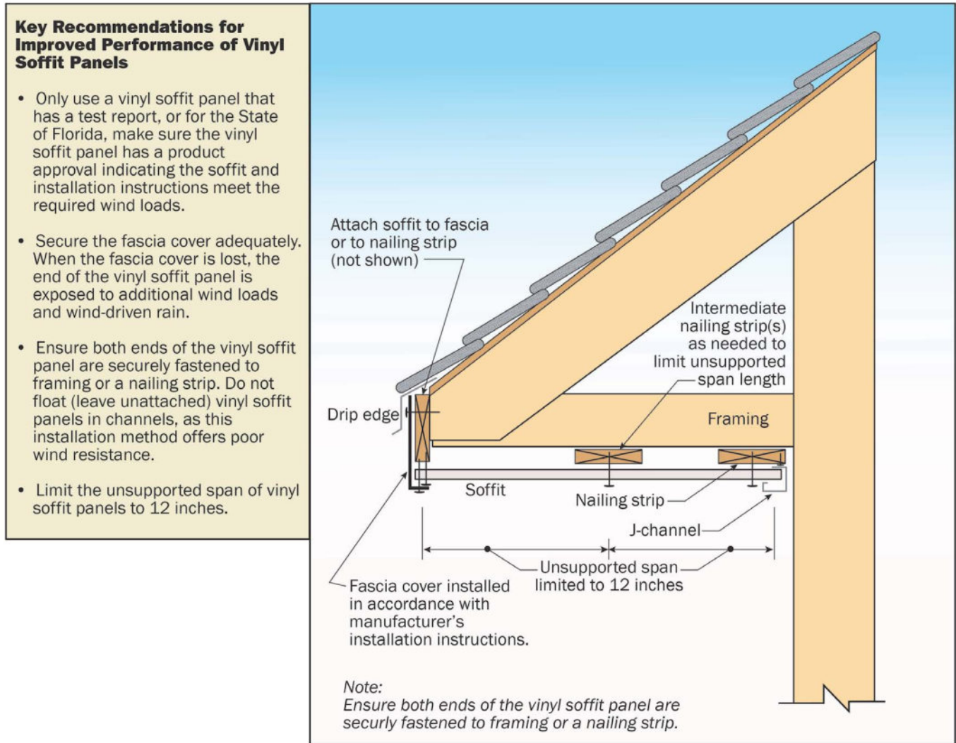
Vinyl Soffit Panel Installation
