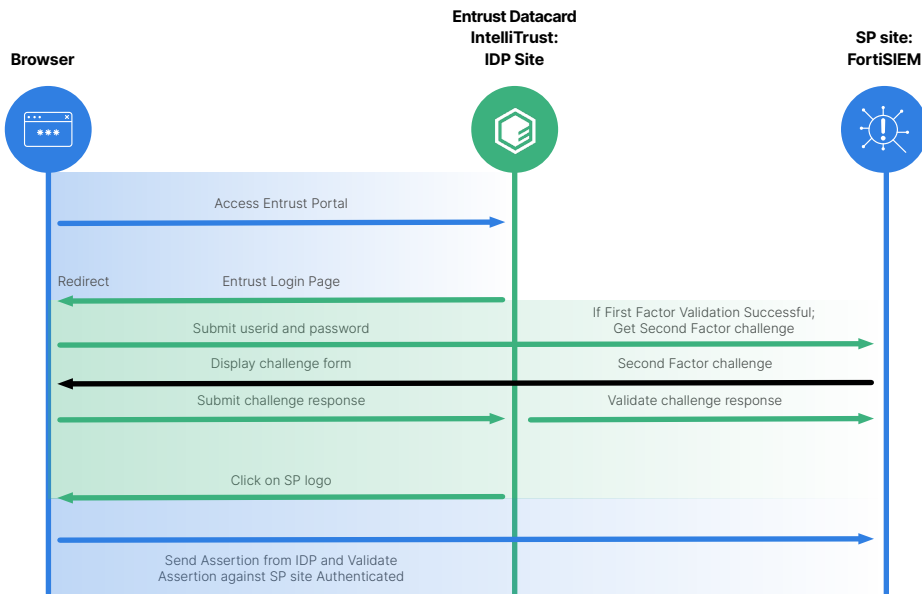
Entrust IDaaS and FortiSIEM integration
