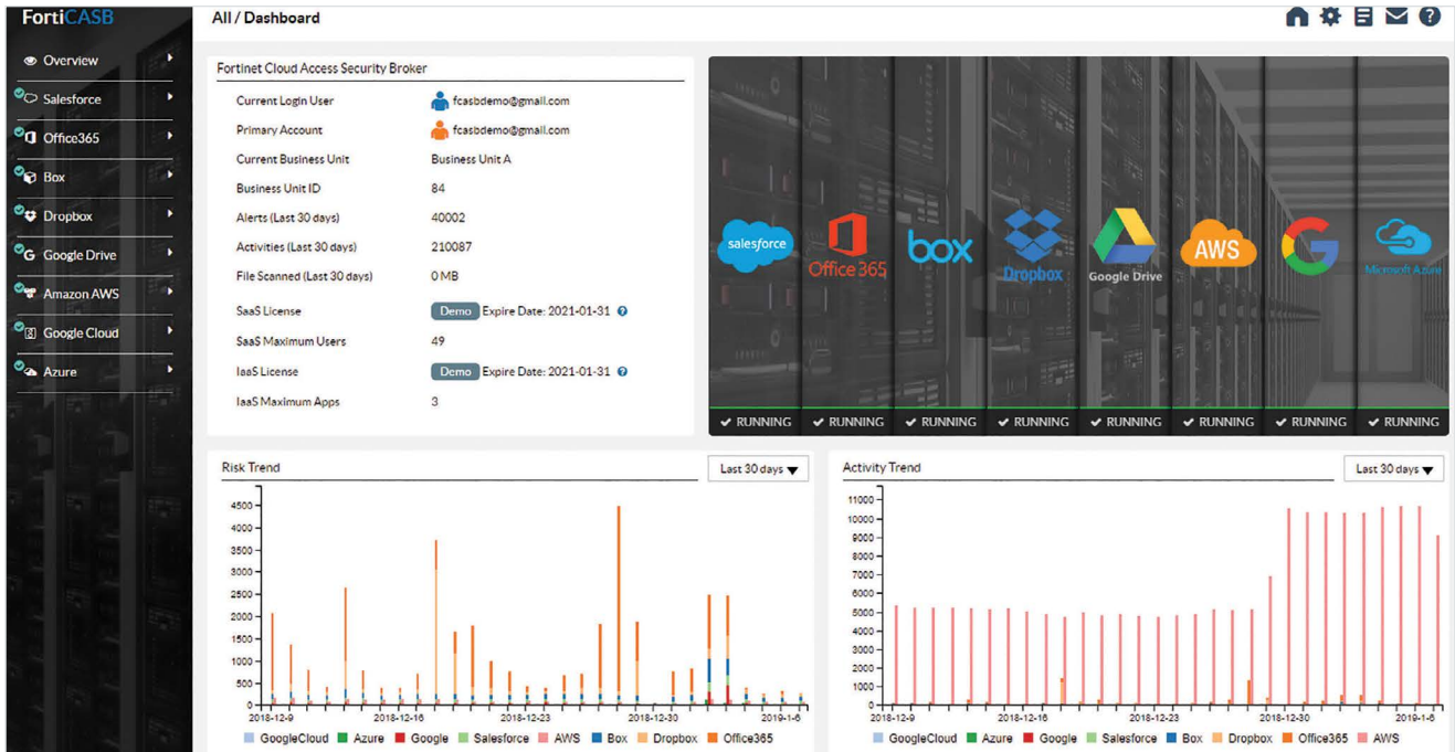
FIGURE 2: FortiCASB overview dashboard—centralized control and management.
