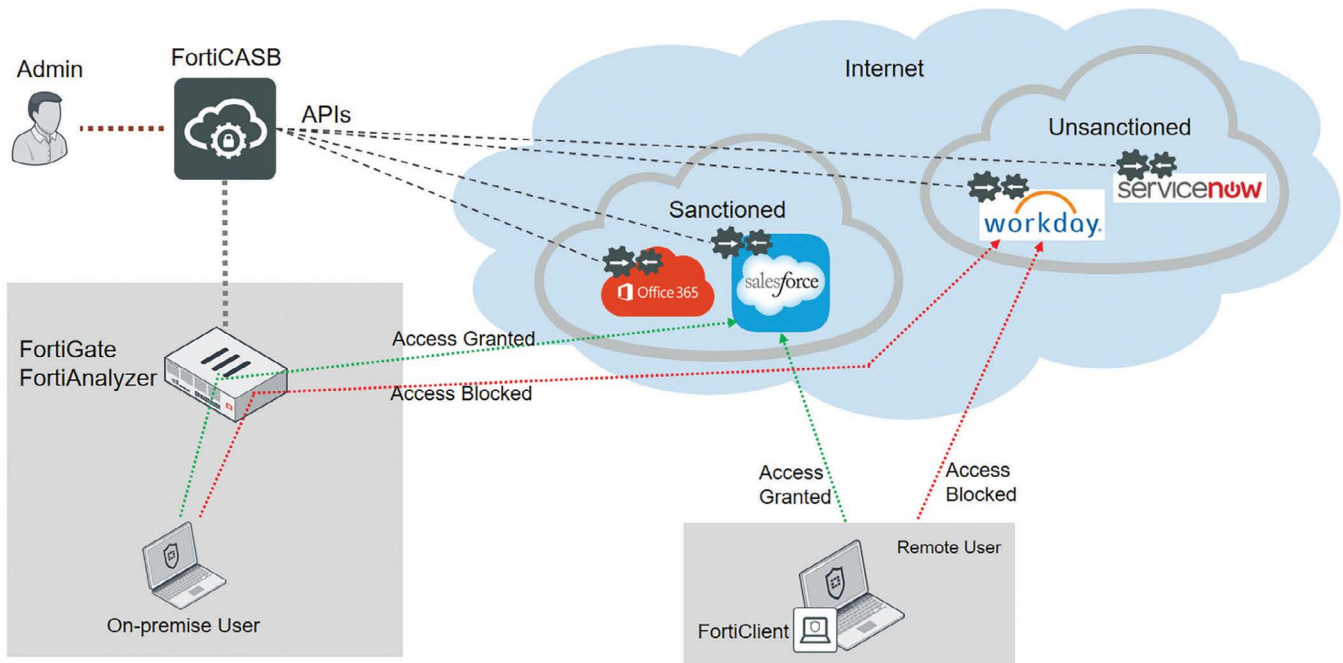
FIGURE 3: FortiCASB provides protection for on-premises and remote access to SaaS applications through its integration with FortiClient.
