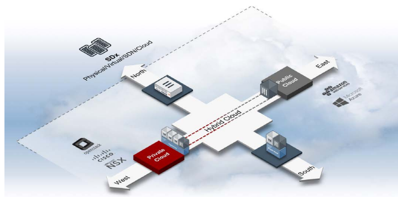
Figure 1: Cloud Security.
