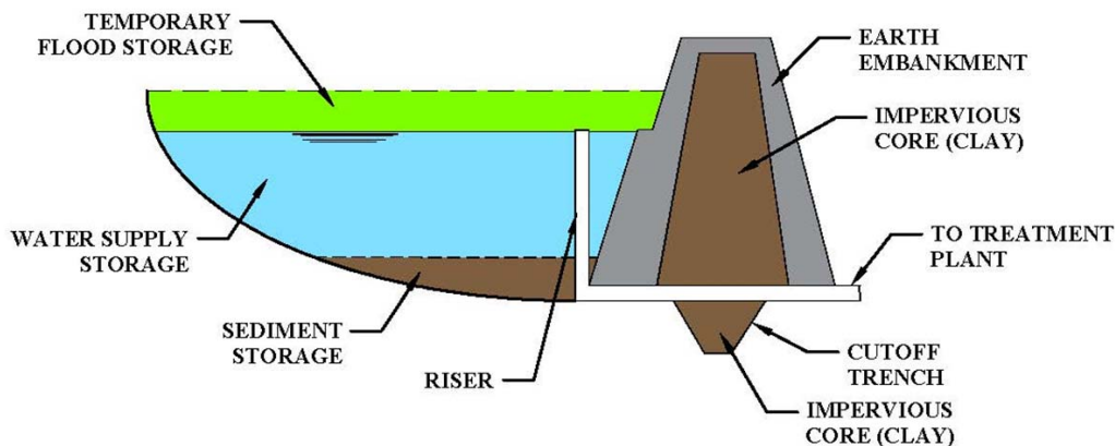
ILLUSTRATION OF WATER SUPPLY EMBANKMENT
