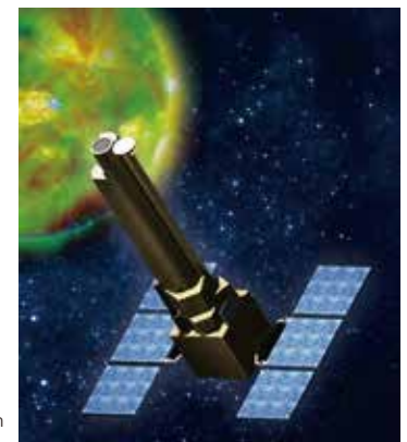
▶ Solar-C satellite in orbit (artist' s illustration) with solar image in EUV. credit: NAOJ/JAXA/NASA.
