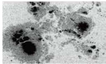
The Sun from the ground and from the space
