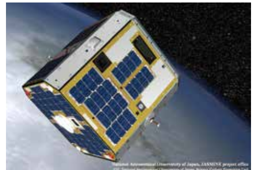
▲Artist's impression of JASMINE (the Small- JASMINE satellite : the small science-satellite with 30 cm primary mirror diameter) observing the Milky Way.
