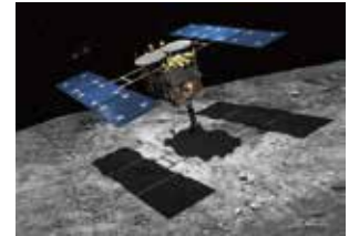
Asteroid explorer "Hayabusa-2" (JAXA/Ikeshita).
