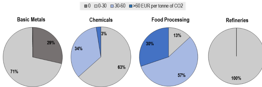
Figure 7. Proportion of CO 2 emissions from fossil fuel energy use in industry at different marginal price intervals in 2021
