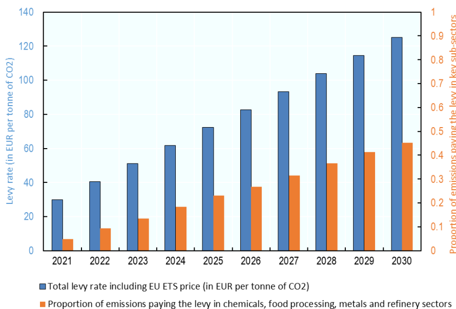
Figure 6. Total levy rate and estimated proportion of emissions paying the levy in the four key sub-sectors, 2021-2030
