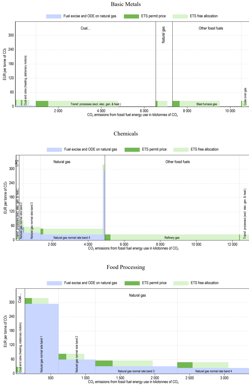
Figure 8. Effective carbon rates on CO 2 emissions from fossil fuel energy use in key sectors, 2021
