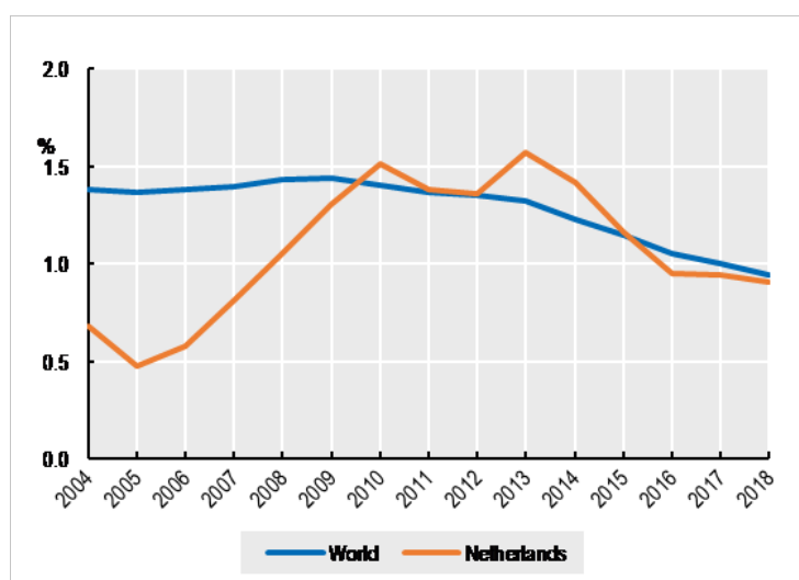
Figure 9. Netherlands-based patents in five emerging low-carbon technologies as a share of total patents in all technologies
