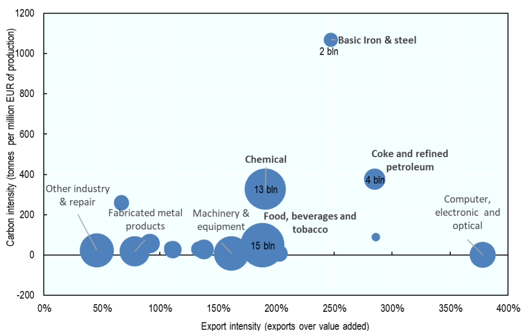
Figure 4. Carbon intensity and export intensity of manufacturing sectors in the Netherlands in 2015
