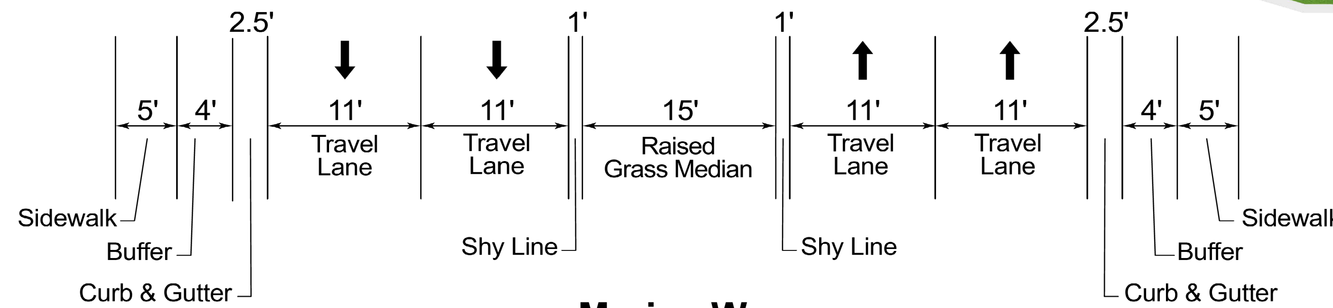
Marina Way Station 109+85 to Station 115+92
