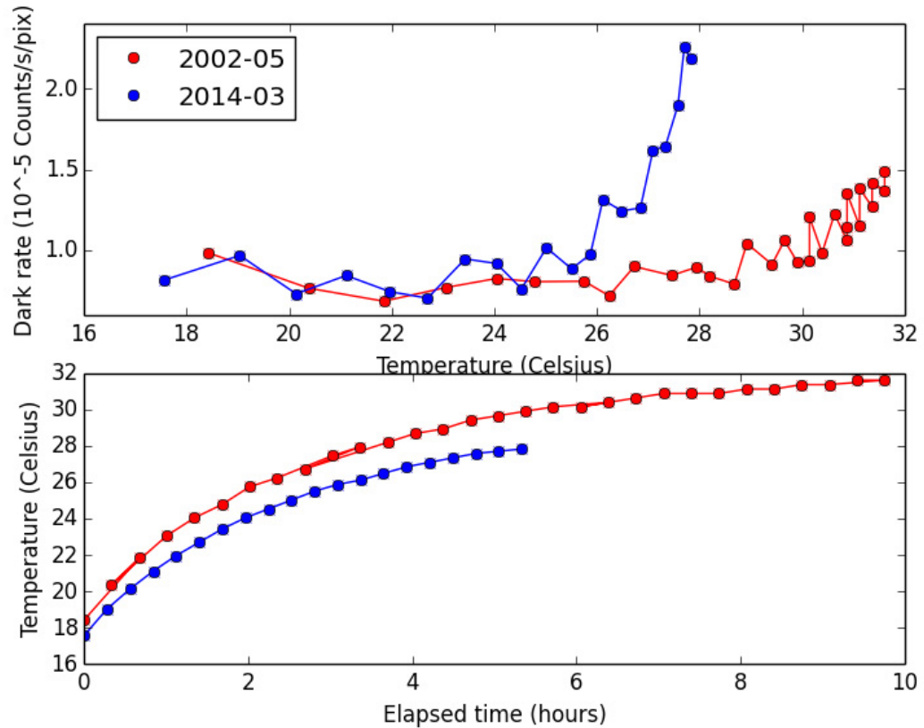
Figure 4.14: SBC Dark Rate and Operating Temperature
