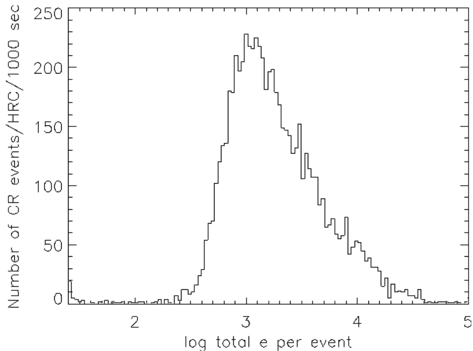
Figure 4.9: Electron deposition of cosmic rays on HRC.
