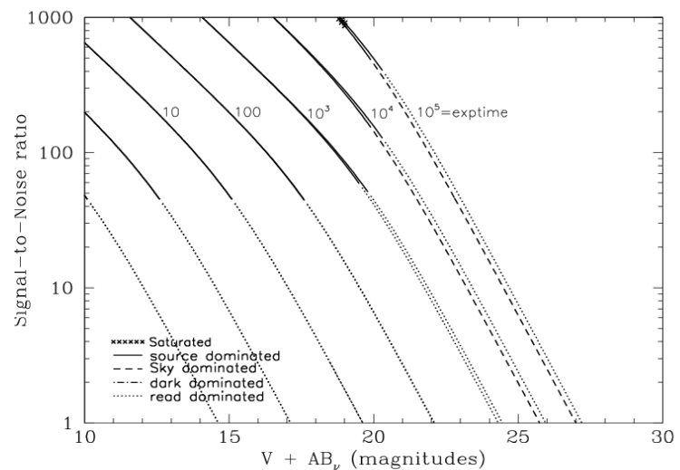
Figure 10.63: Extended source S/N vs. V+AB v for the HRC/F502N filter. Top curves are for low sky and bottom curves are for average sky for a 1 arcsec 2 area.
