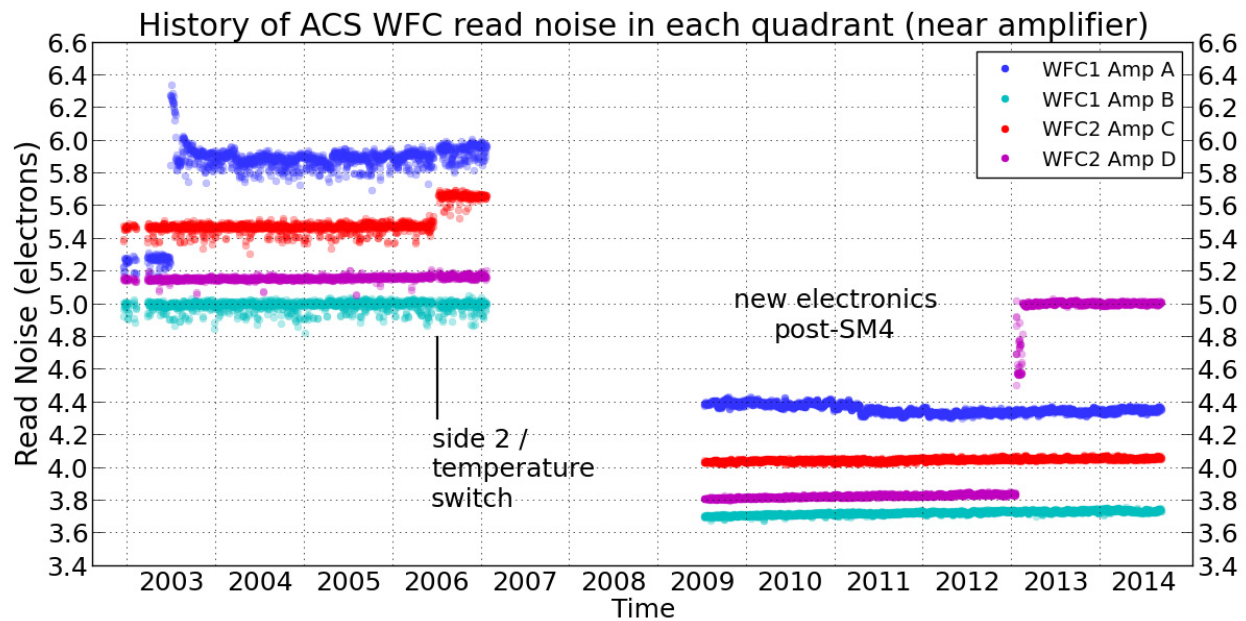
Figure 4.4: History of ACS/WF read noise
