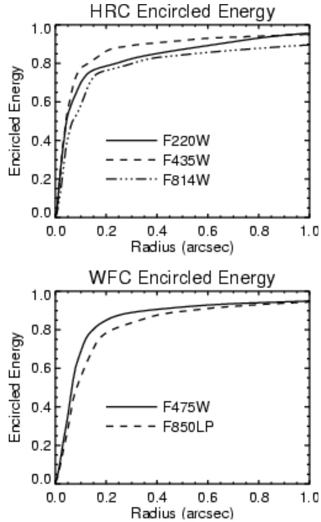
Figure 5.13: Encircled energy for the CCD channels.
