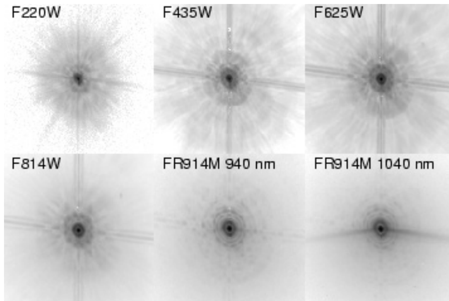
Figure 5.18: ACS HRC PSFs (3.25" x 3.25").
