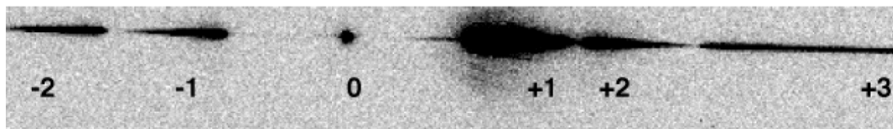
Figure 6.17: Fully dispersed spectrum for white dwarf GD153 with WFC/G800L.
