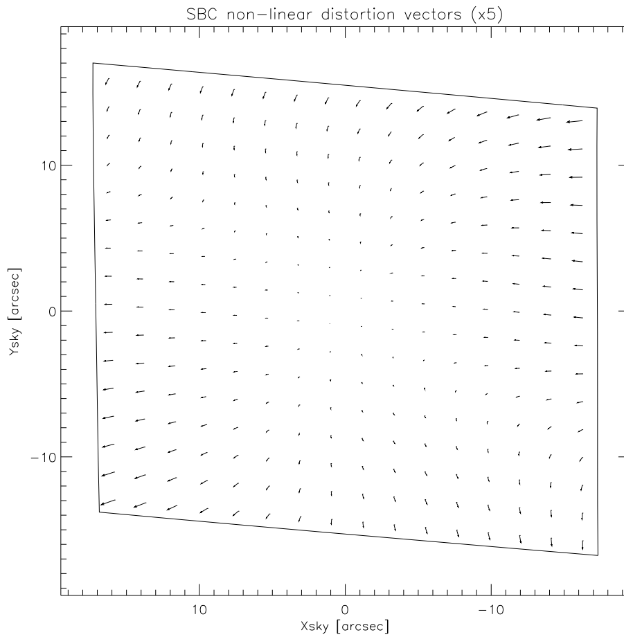
Figure 10.131: The geometric distortion map for the ACS/SBC
