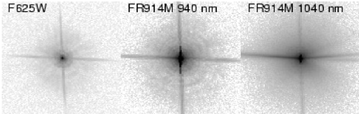
Figure 5.17: ACS WFC PSFs (10" x 10"). FR914M images are saturated.
