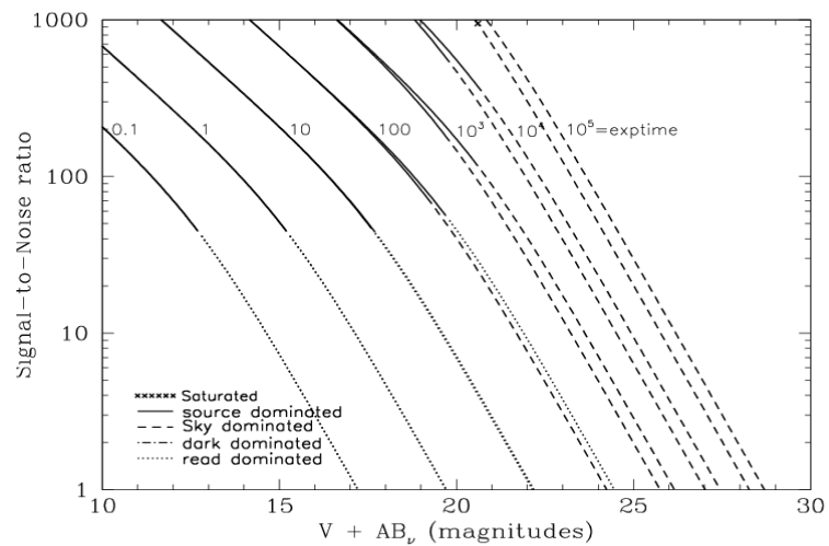
Figure 10.90: Extended source S/N vs. V+AB_v for the HRC/F850LP filter. Top curves are for low sky and bottom curves are for average sky for a 1 arcsec 2 area.
