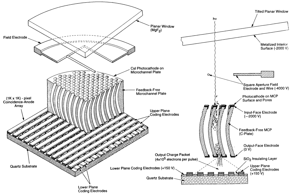
Figure 4.10: Design of the SBC MAMA.
