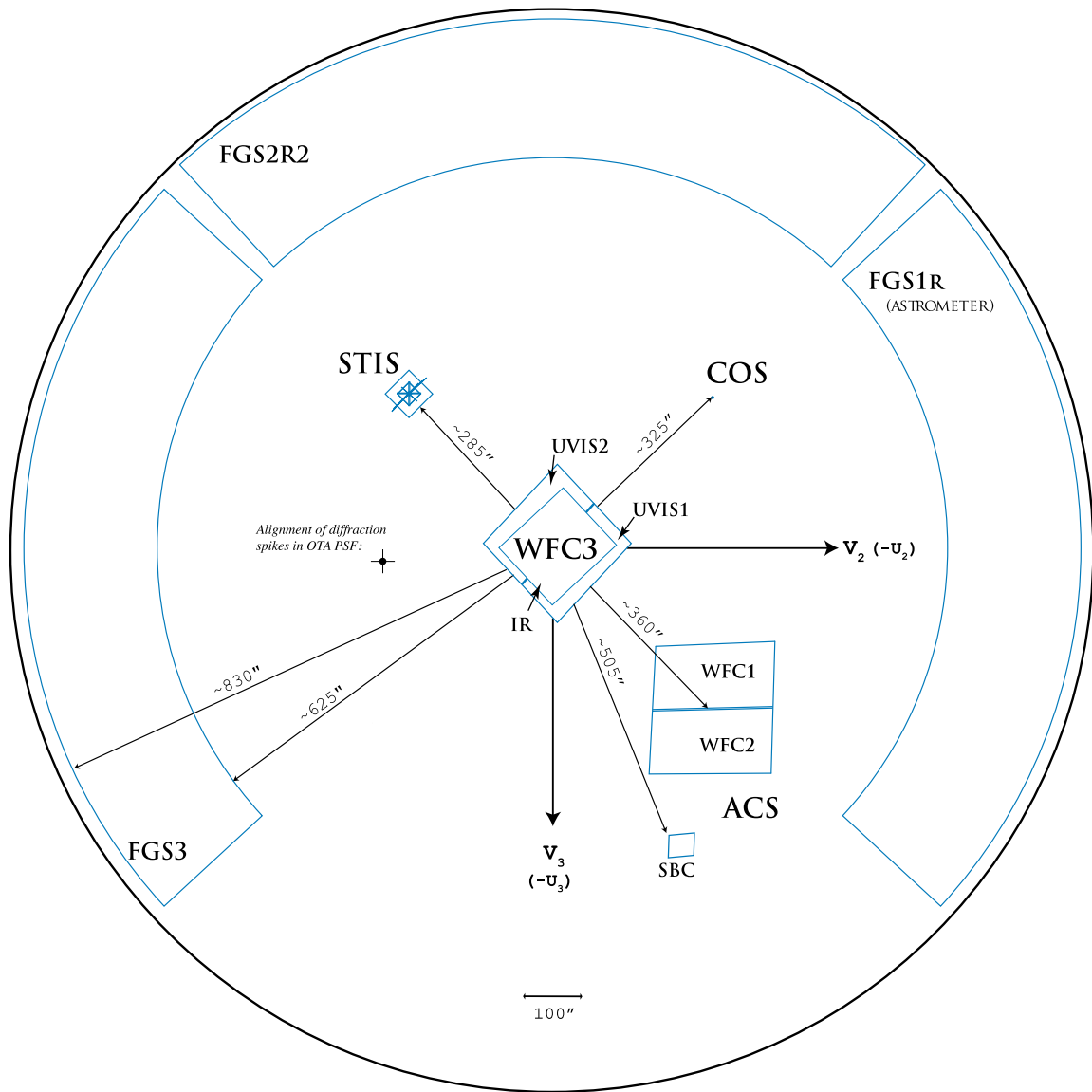
Figure 3.1: The HST field of view with the locations of the SI and the FGS apertures in the (U2,U3) focal plane.
