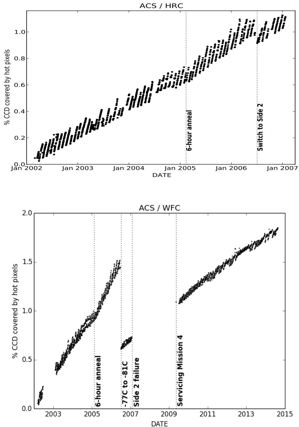
Figure 4.5: Hot Pixel Growth Rate for HRC and WFC
