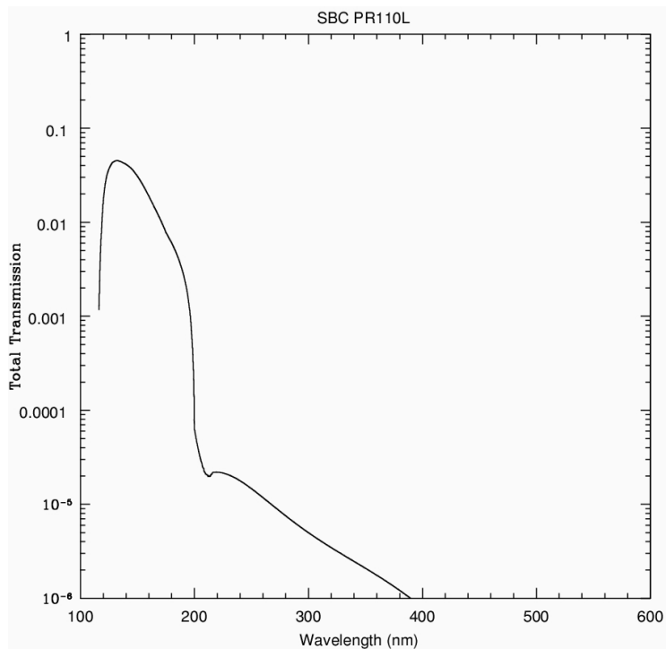
Figure 4.11: Total transmission curve for ACS SBC plus the PR110L prism.
