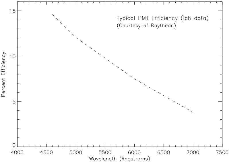
Figure 2.12: PMT Efficiency
