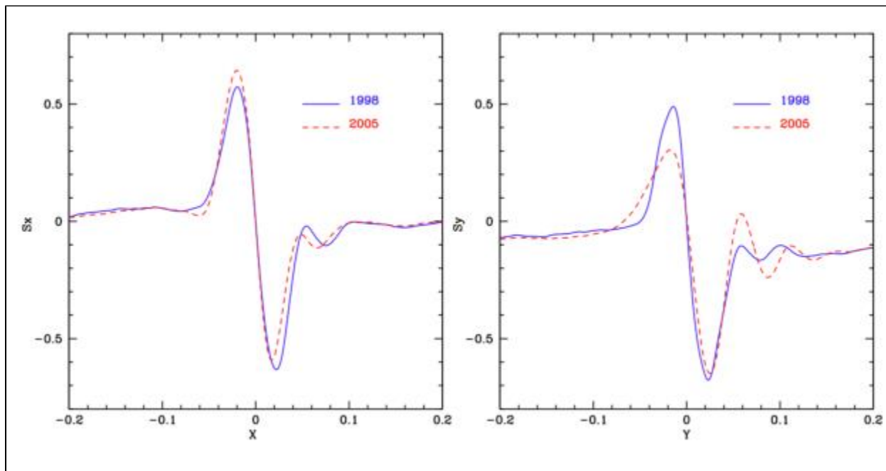
Figure 2.7: FGS1r S-curves
