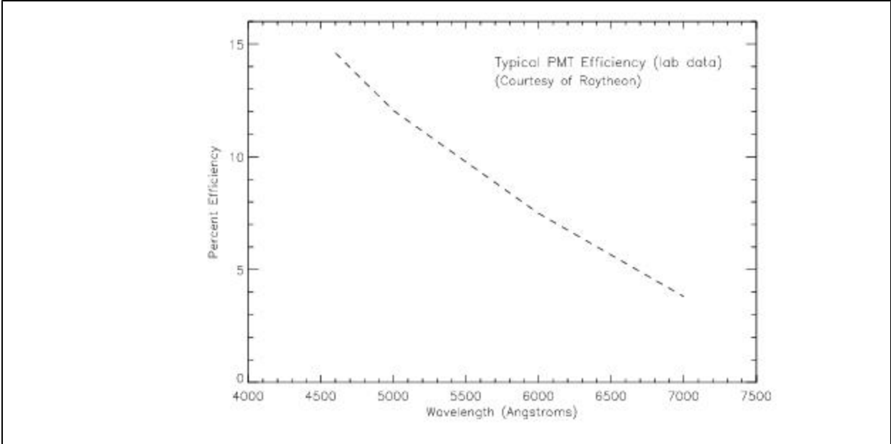
Figure 2.12: PMT Efficiency
