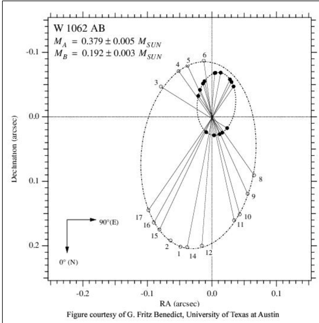
Figure 3.4 shows the orbits of the components of Wolf 1062 about the system's barycenter. This has been determined from both Transfer mode observations, which yield the relative orbit, and Position mode observations, which map the orbit of the primary relative to reference stars distributed about the FGS FOV (in effect establishing the inertial reference frame). Note that the Position mode data also yield the system's parallax and proper motion.
