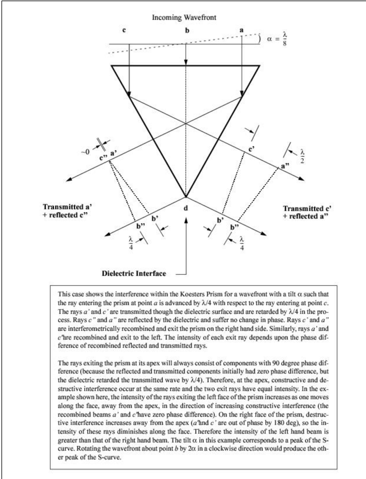
Figure 2.3: The Koesters Prism: Constructive and Destructive Interference.
