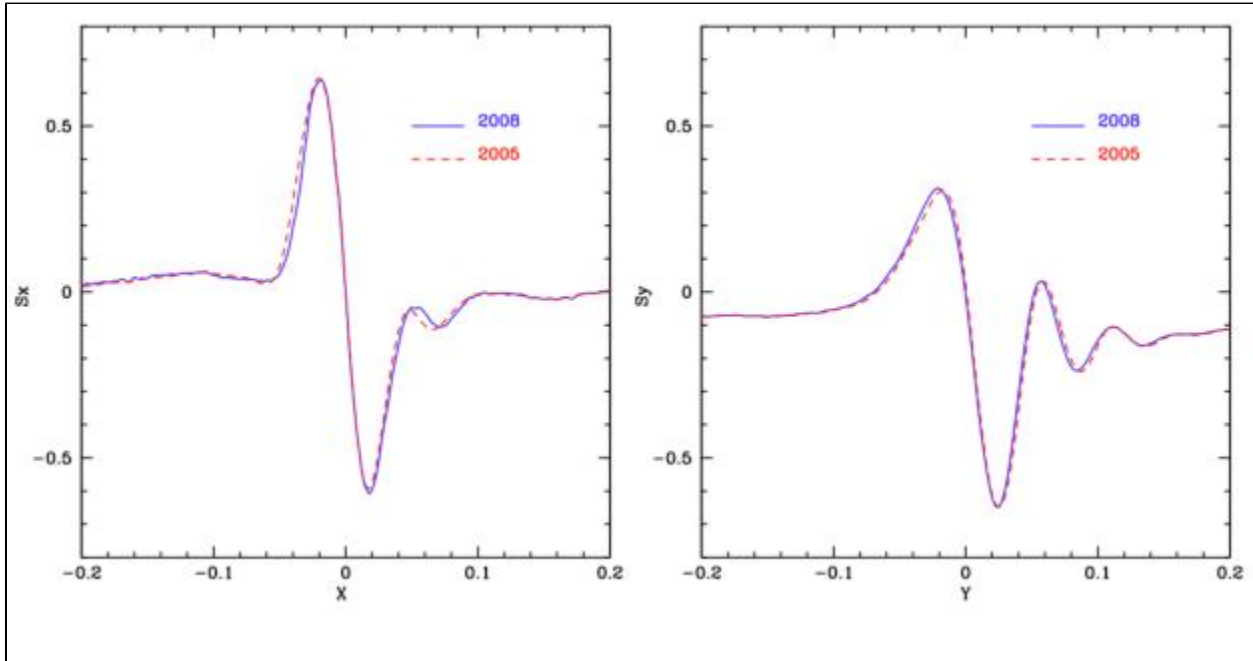
Figure 2.8:FGS1r S-curves 2005
