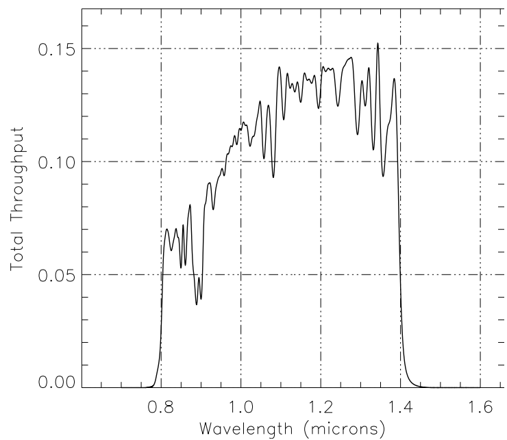
Figure A.6: NIC1, F110W Throughput
