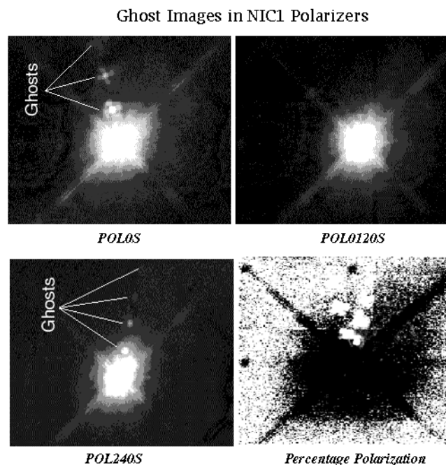
Figure 5.6: Ghost Images in NIC1 Polarizers.
