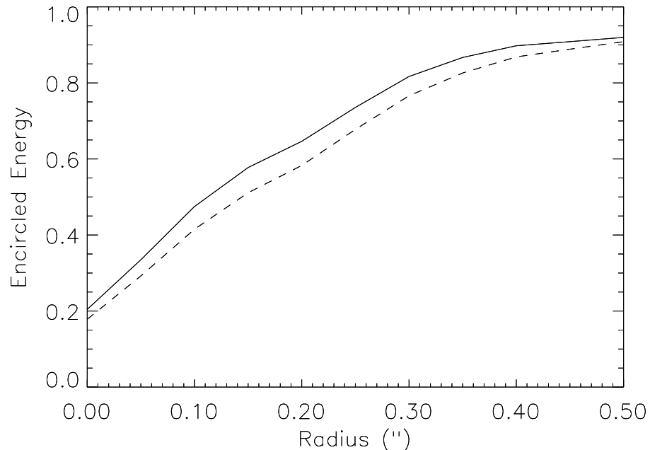
Figure 4.13: NIC3 encircled energy at 1.6 microns at optimum focus (PAM= -12 mm, solid line) and at the best achievable focus (PAM= -9.5 mm, dashed line) with the HST secondary mirror at nominal position.
