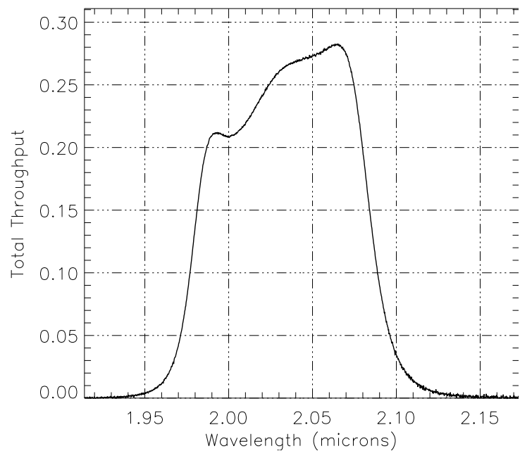
Figure A.26: NIC2, F204M Throughput
