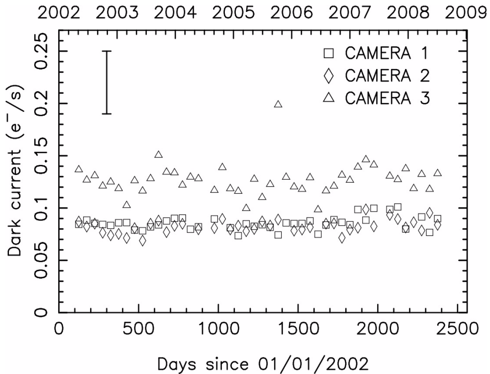
Figure 7.4: Results from the NICMOS dark current monitoring program following the installation of the NCS. Shown are the monthly (bi-monthly since January 2003) linear dark current measurements for all three NICMOS cameras. Note that the linear dark current is stable within the measurement errors (a typical error bar for Camera 3 is shown in the upper left corner, the other cameras have errors about half of this).
