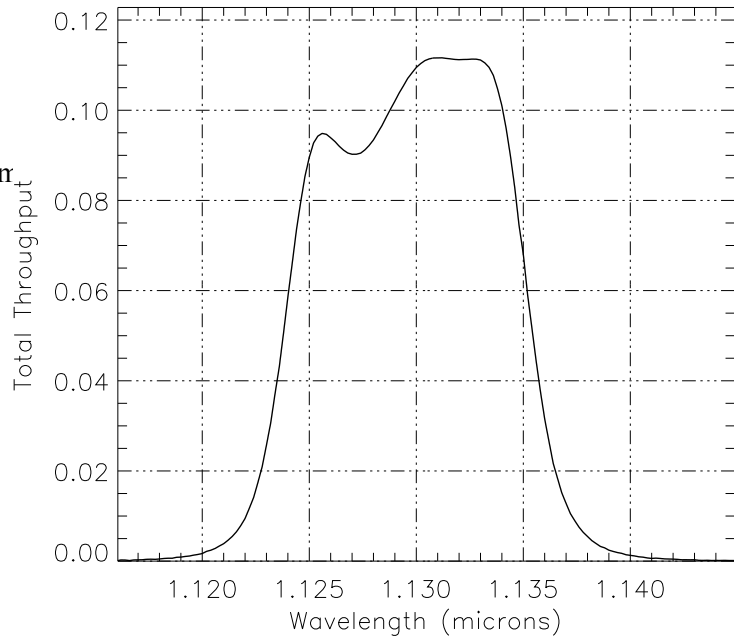
Figure A.7: NIC1, F113N Throughput
