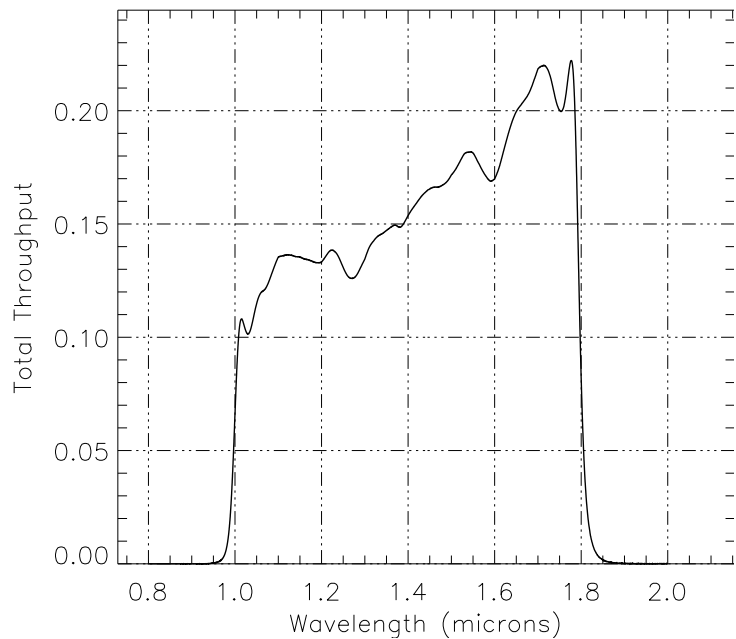
Figure A.8: NIC1, F140W Throughput
