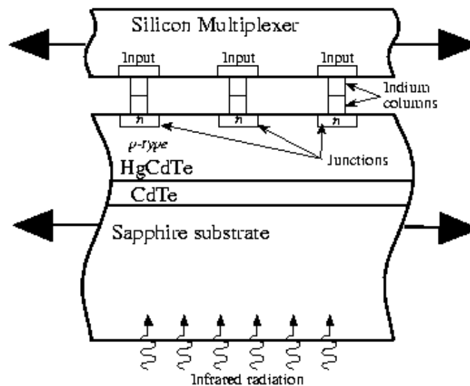
Figure 7.1: Cross-section of a NICMOS3-type detector (not to scale). Adapted from McLean, Ian S. "Electronic imaging in astronomy. Detectors and instrumentation", 1997.
