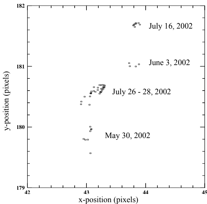
Figure 5.3: Coronagraphic hole location (detector coordinates) during Cycle 11.
