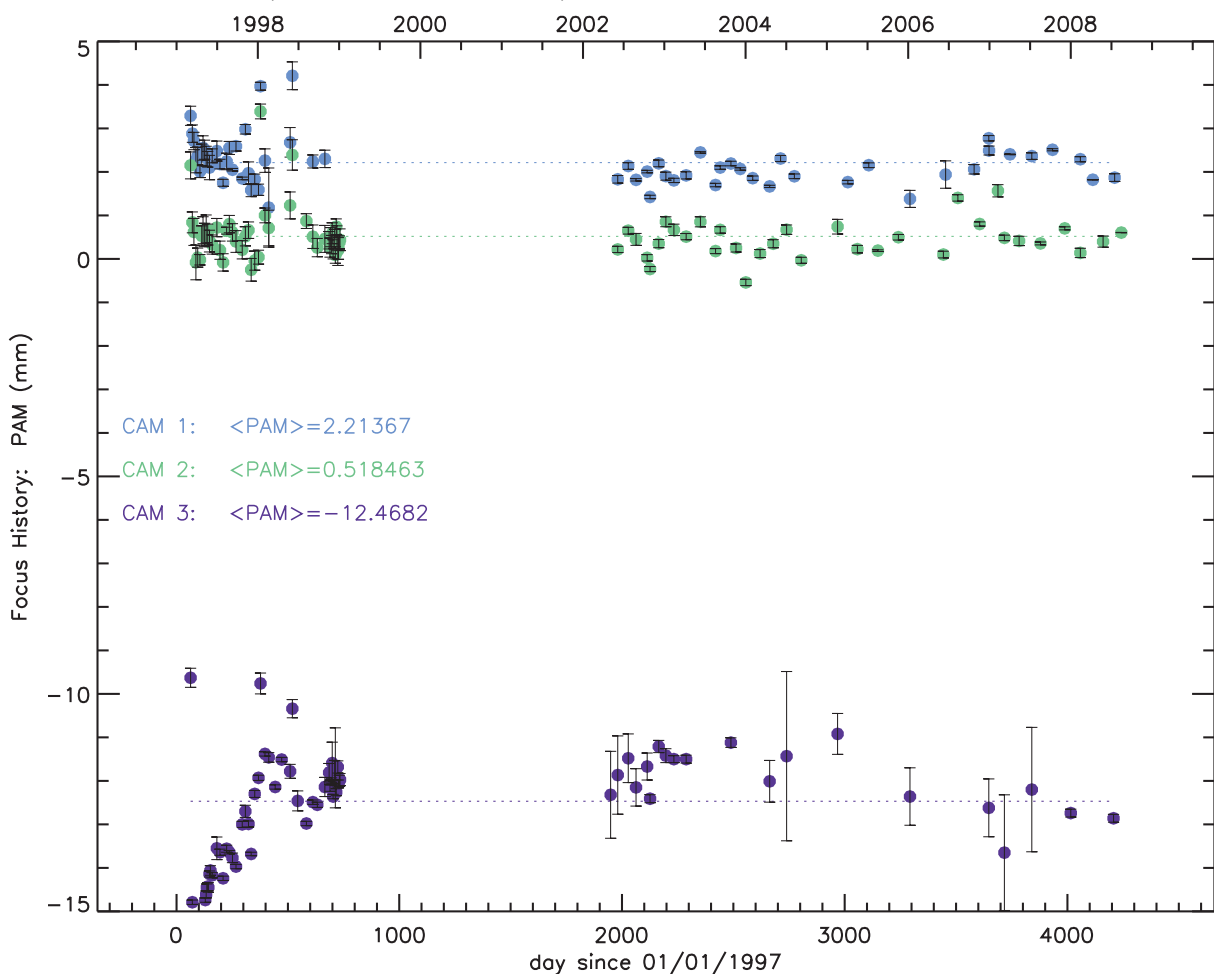
Figure 4.6: NICMOS Focus History as of 4 July 2007 (focus at the detector center).
