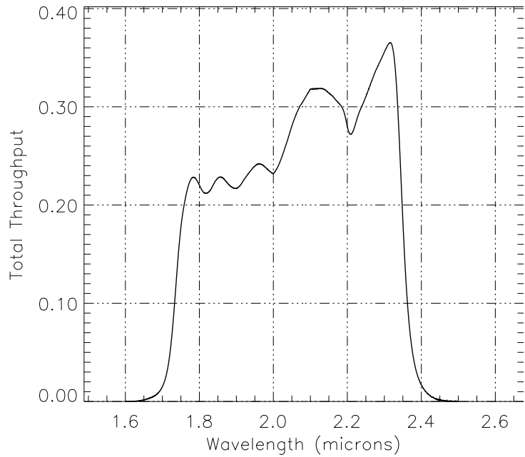
Figure A.27: NIC2, F205W Throughput
