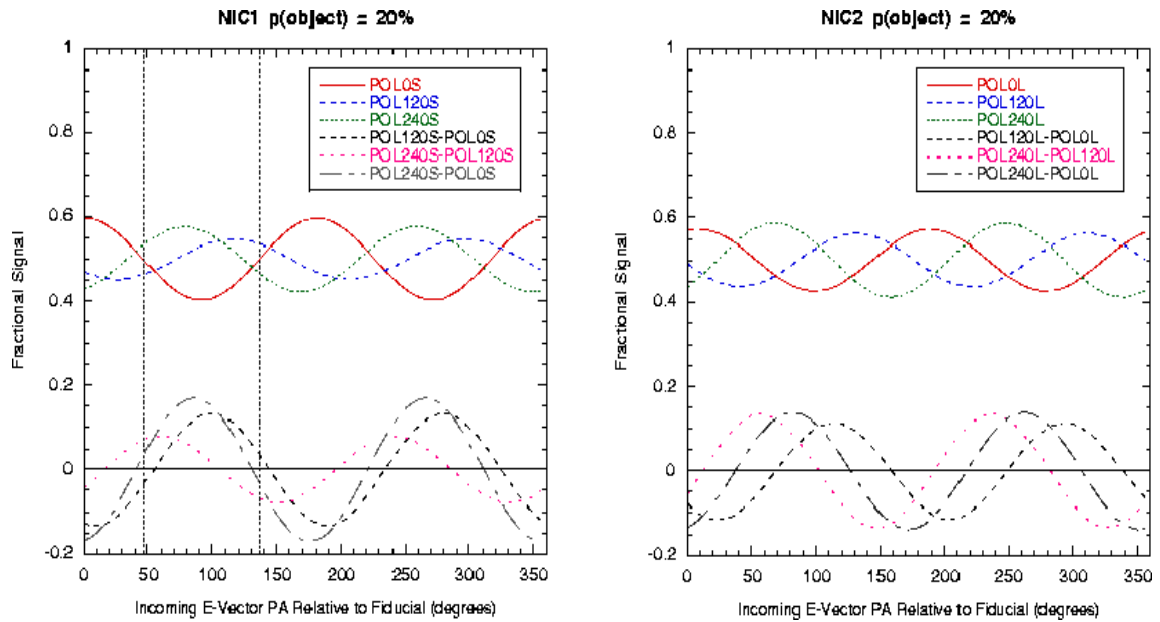
Figure 5.7: Fractional signal measured in each NICMOS polarizer as a function of incident electric position angle. Refer to http://www.ecf.hq.org/nicmos/sardinia/node14.html#2206 "Imaging Polarimetry with NICMOS" for more details.
