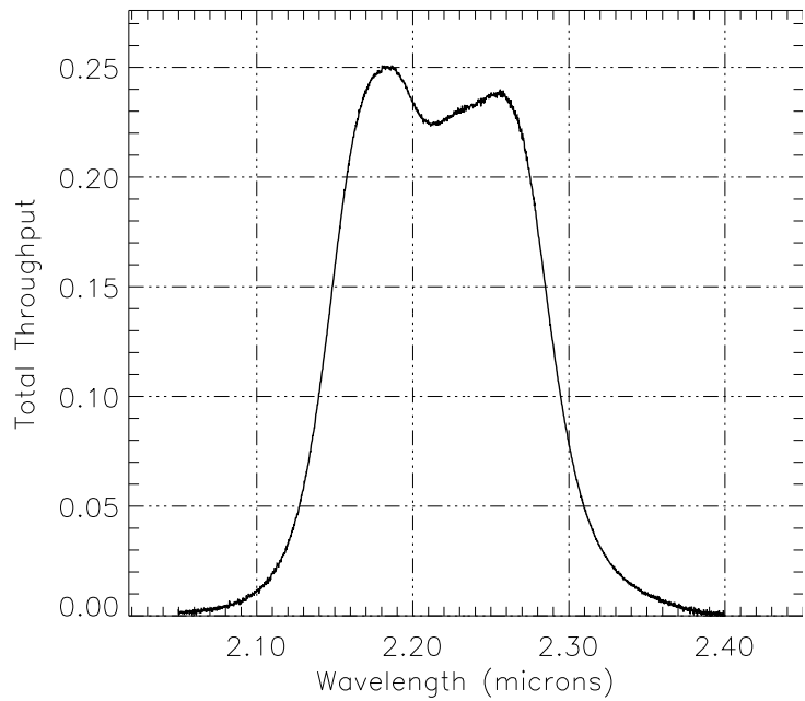
Figure A.49: NIC3, F222M Throughput
