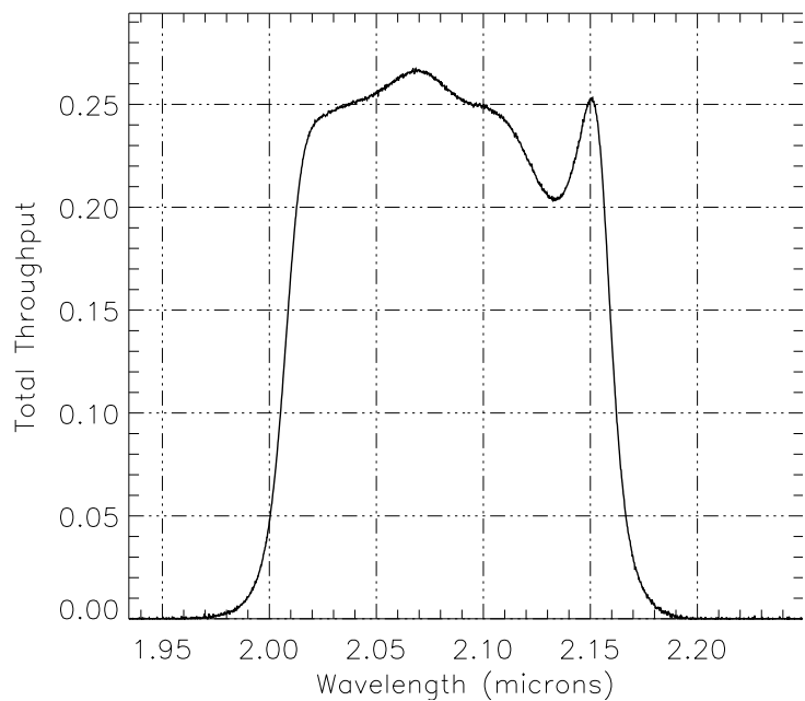
Figure A.28: NIC2, F207M Throughput
