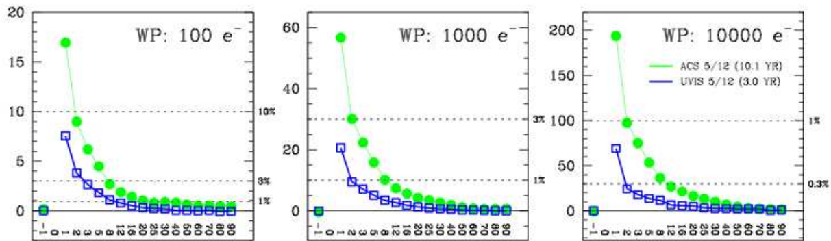
Observed charge trailing 100, 1000, and 10000 e^- hot pixels in WFC3 (blue) and ACS (green) images from May 2012.
