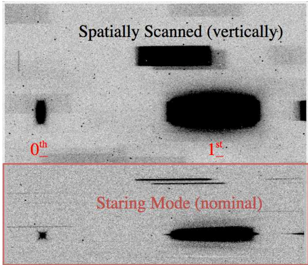
A spatially-scanned IR spectrum, labeled with its 0th and +1st order light, and compared to a nominal staring-mode slitless spectrum of the same field (red outlined inset) (WFC3 ISR 2012-08). The images are 512 columns wide, of the detector's 1024. The scan was 40 pixels high (4.8 arcsec).
