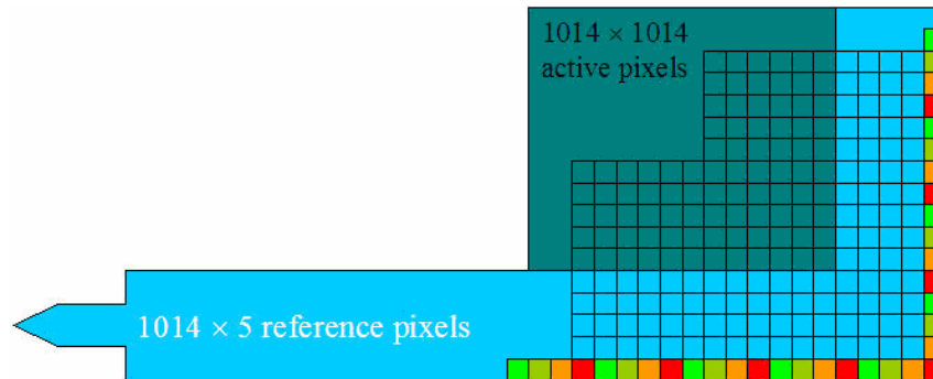
Figure 5.18: Schematic layout of the active pixels (dark shading) and of the reference pixels at a corner of the WFC3/IR detector. The color coding represents different values of the reference pixel capacitance.
