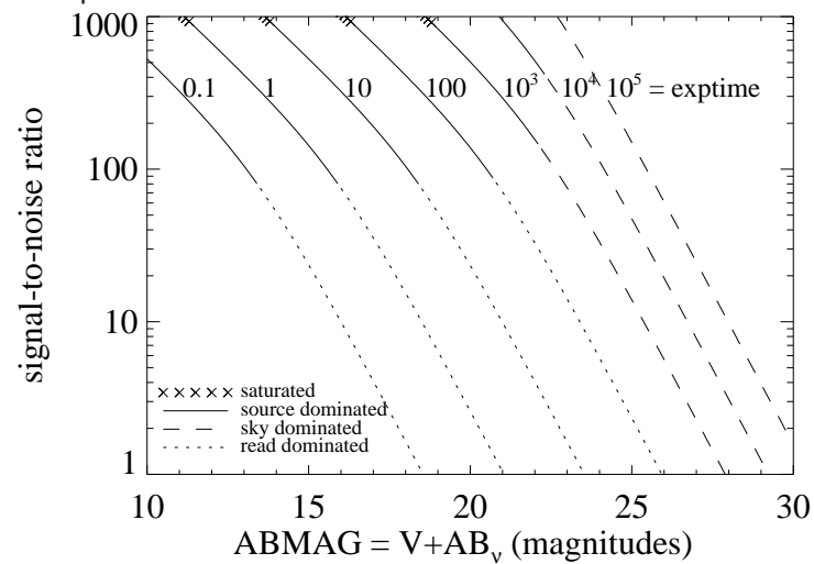
Figure A.57: Extended source S/N vs. V+AB_V for the F475X filter, assuming high sky backgrounds and a source uniformly filling a 1 \text{ arcsec}^2 aperture.
