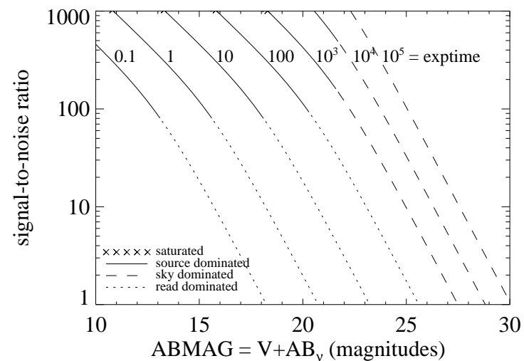
Figure A.72: Extended source S/N vs. V+AB_v for the F600LP filter, assuming high sky backgrounds and a source uniformly filling a 1 \text{ arcsec}^2 aperture.
