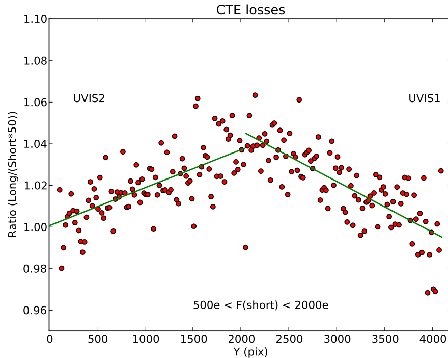
Figure 5.12: Normalized ratio of stellar fluxes measured in a long exposure of NGC 1850 to fluxes measured in a short exposure, shown as a function of Y position on the detector. The ratio deviates from 1 because of the relatively greater CTE losses in the shorter (fainter) exposure.
