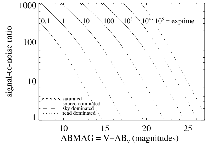
Figure A.87: Extended source S/N vs. V+AB_v for the F645N filter, assuming high sky backgrounds and a source uniformly filling a 1 \text{ arcsec}^2 aperture.
