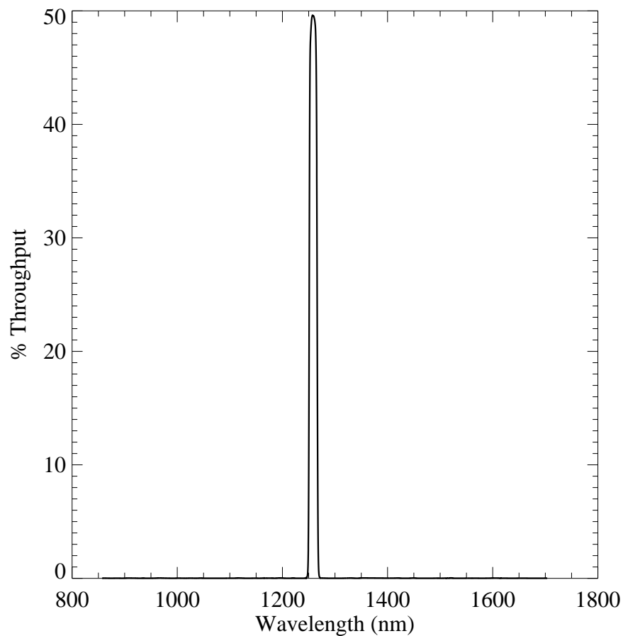
Figure A.199: Integrated system throughput for F126N.
