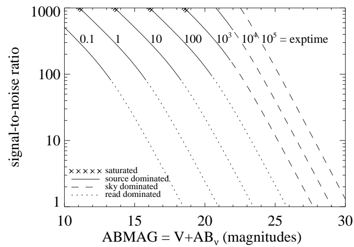
Figure A.75: Extended source S/N vs. V+AB_V for the F606W filter, assuming high sky backgrounds and a source uniformly filling a 1 \text{ arcsec}^2 aperture.
