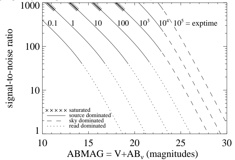
Figure A.224: Point source S/N vs. V+AB_V for the F160W filter, assuming high sky backgrounds and a 3 \times 3 pixel aperture.
