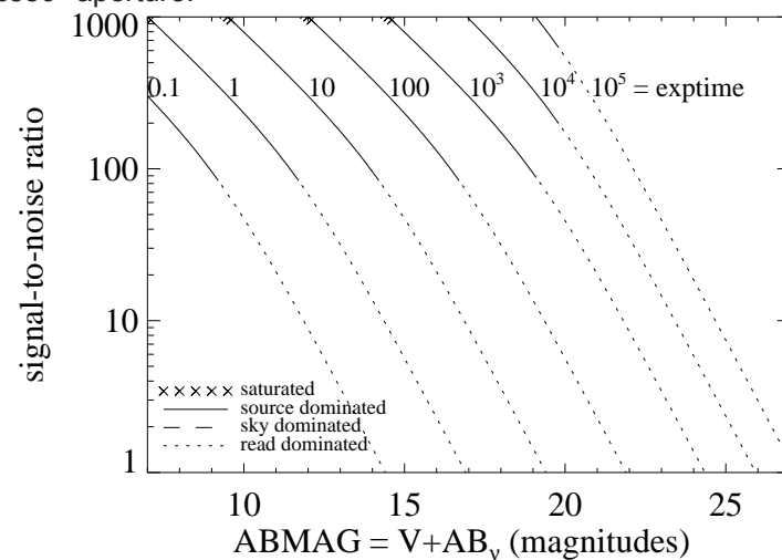
Figure A.162: Extended source S/N vs. V+AB_V for the FQ634N filter, assuming high sky backgrounds and a source uniformly filling a 1 arcsec 2 aperture.
