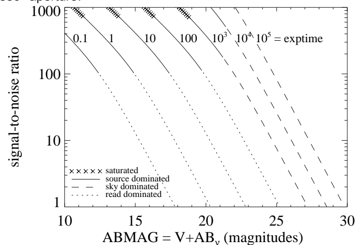
Figure A.189: Extended source S/N vs. V+AB_V for the F098M filter, assuming high sky backgrounds and a source uniformly filling a 1 \text{ arcsec}^2 aperture.
