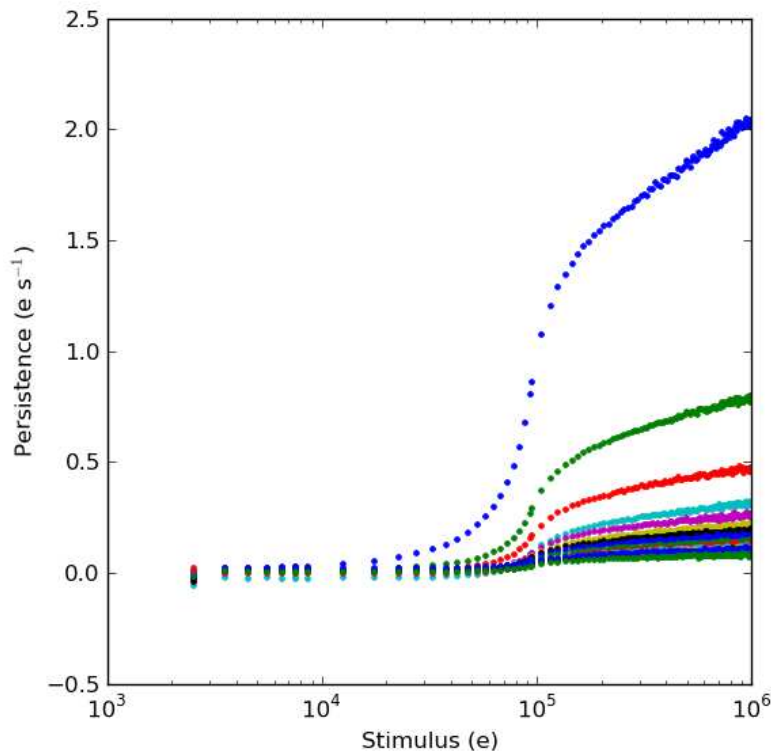
Figure 5.25: Persistence as a function of fluence ("stimulus" provided by exposure to Omega Cen) observed over the detector in a subsequent series of darks (color coded)
