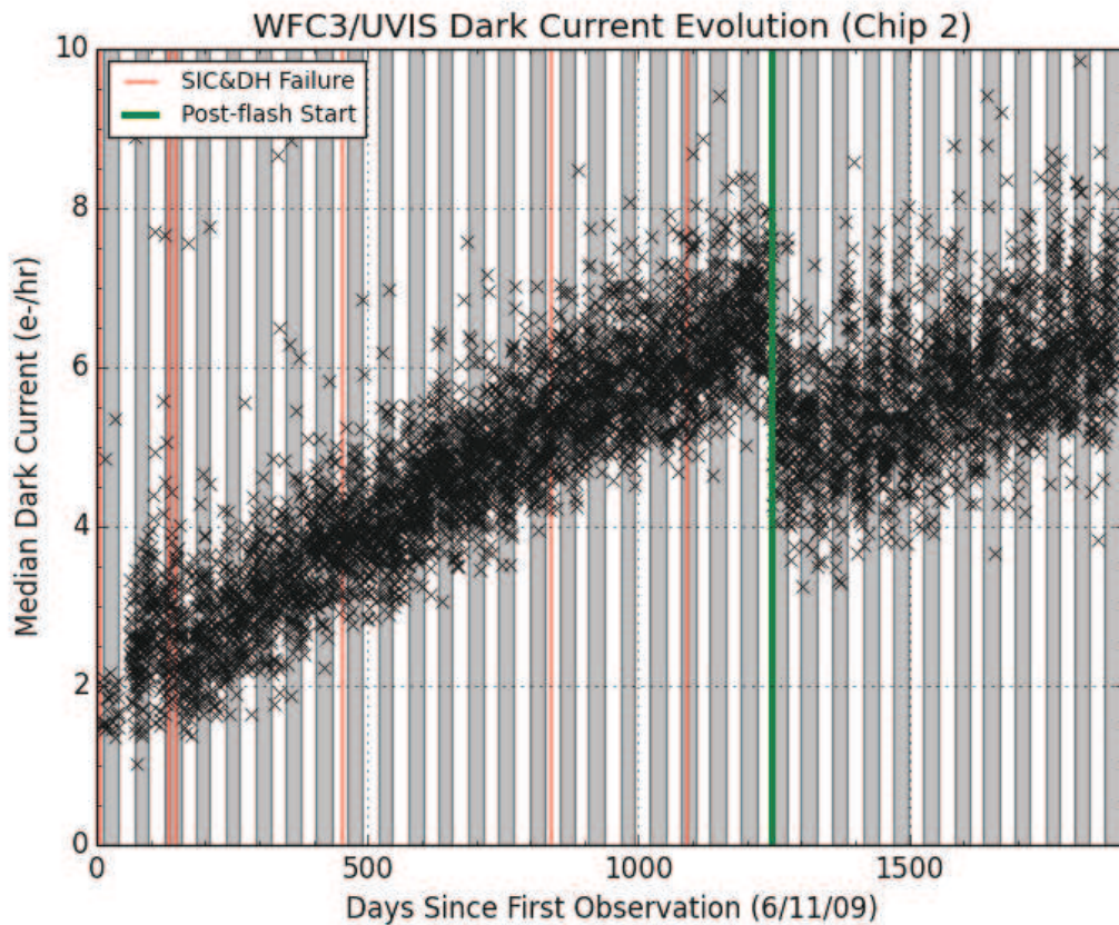
Figure 5.7: Median dark current of the WFC3/UVIS detector measured on orbit from June 2009 to Aug 2014. The use of post-flash accounts for the discontinuity in Nov 2012.
