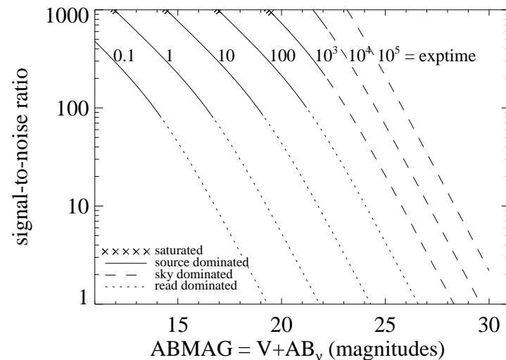
Figure A.27: Extended source S/N vs. V+AB_v for the F350LP filter, assuming high sky backgrounds and a source uniformly filling a 1 \text{ arcsec}^2 aperture.
