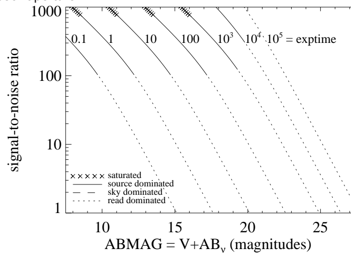
Figure A.213: Extended source S/N vs. V+AB_v for the F132N filter, assuming high sky backgrounds and a source uniformly filling a 1 \text{ arcsec}^2 aperture.
