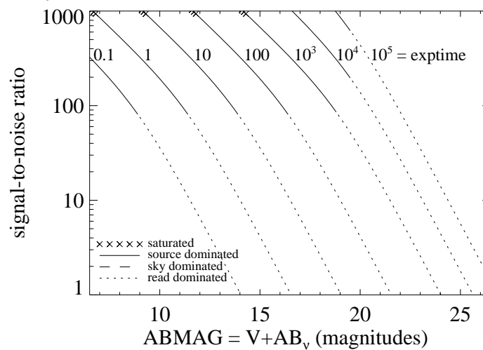
Figure A.144: Extended source S/N vs. V+AB_v for the FQ436N filter, assuming high sky backgrounds and a source uniformly filling a 1 \text{ arcsec}^2 aperture.
