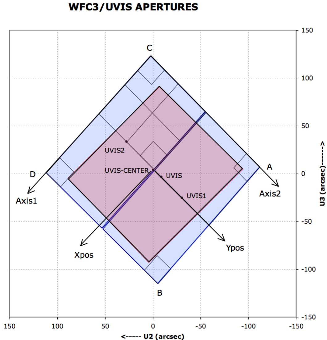
Figure 6.1: UVIS Aperture Diagram
