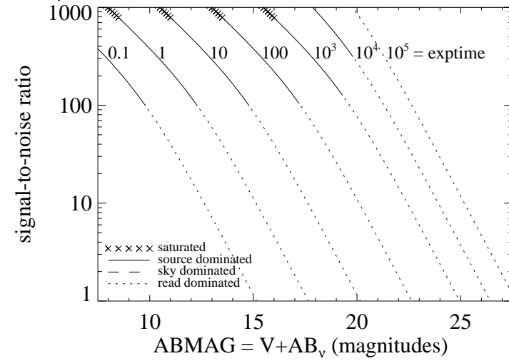
Figure A.207: Extended source S/N vs. V+AB_v for the F128N filter, assuming high sky backgrounds and a source uniformly filling a 1 \text{ arcsec}^2 aperture.
