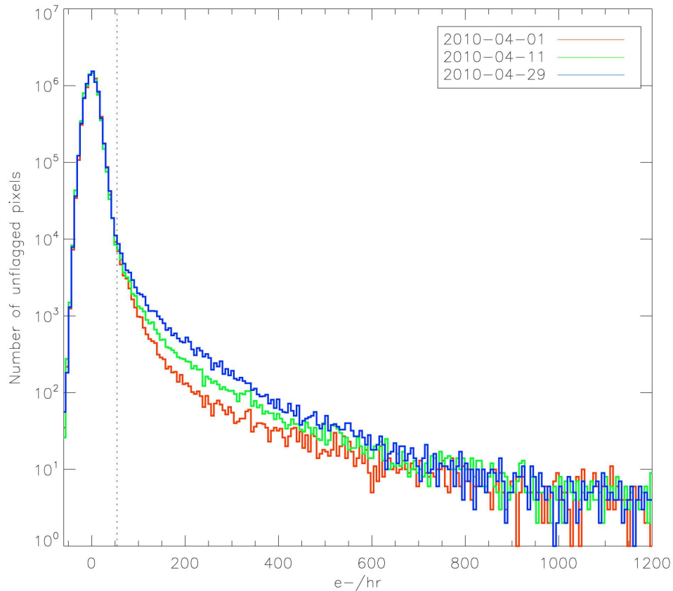
Figure 5.8: Dark histograms illustrate the increase in the number of hot pixels (>54 e - /hr) between anneal procedures. The April 1, April 11, and April 29 curves (red, green, and blue, respectively) are from one day after an anneal procedure, about mid-way between anneals, and about one day prior to an anneal procedure.
