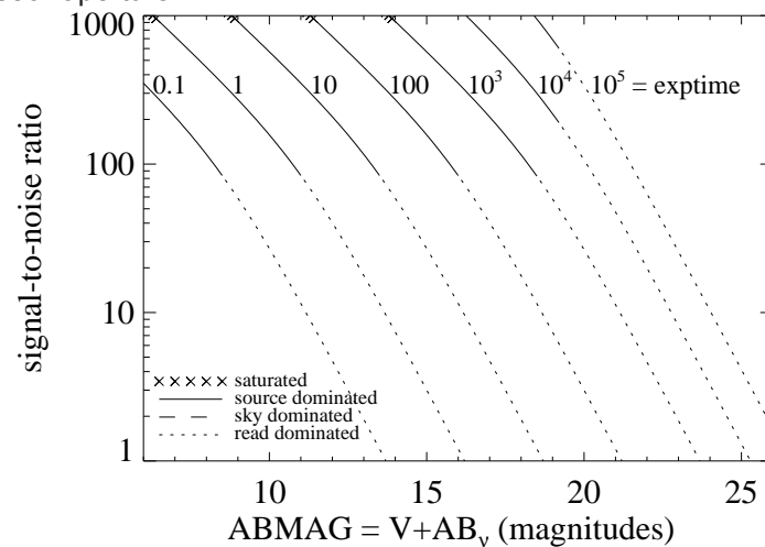
Figure A.147: Extended source S/N vs. V+AB_V for the FQ437N filter, assuming high sky backgrounds and a source uniformly filling a 1 arcsec 2 aperture.
