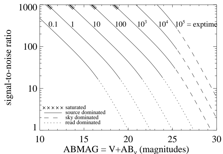
Figure A.56: Point source S/N vs. V+AB_V for the F475X filter, assuming high sky backgrounds and a 5 \times 5 pixel aperture.
