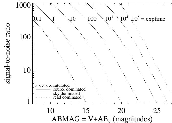
Figure A.93: Extended source S/N vs. V+AB_v for the F657N filter, assuming high sky backgrounds and a source uniformly filling a 1 \text{ arcsec}^2 aperture.
