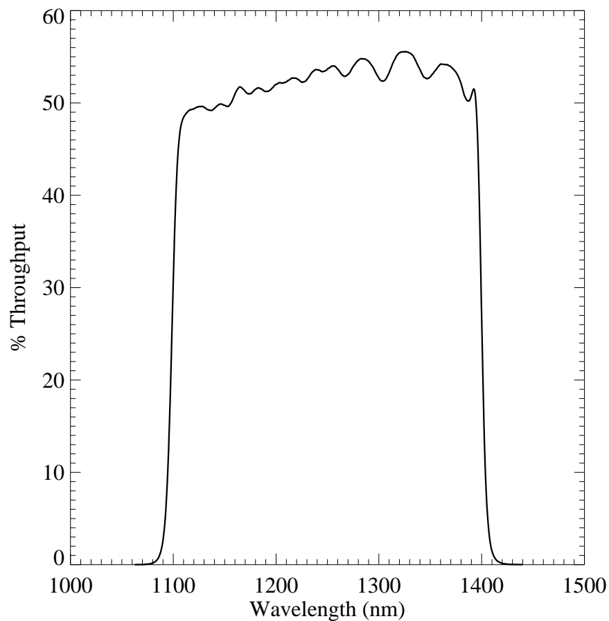
Figure A.196: Integrated system throughput for F125W.
