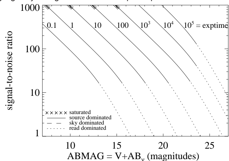
Figure A.92: Point source S/N vs. V+AB_v for the F657N filter, assuming high sky backgrounds and a 5 \times 5 pixel aperture.
