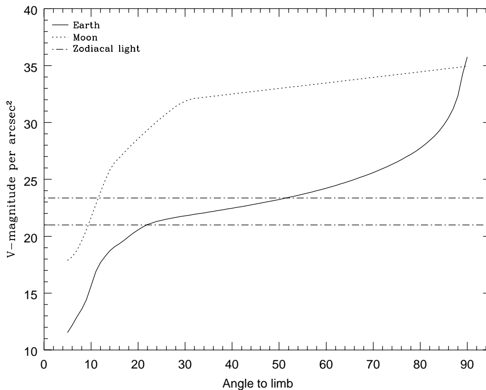
Figure 9.2: Background contributions in V magnitude per arcsec 2 due to the zodiacal light, Moon, and sunlit Earth, as a function of angle between the target and the limb of the Earth or Moon. The two zodiacal light lines show the extremes of possible values.
