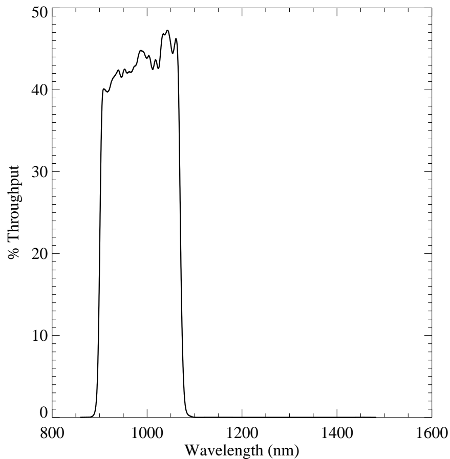
Figure A.187: Integrated system throughput for F098M.
