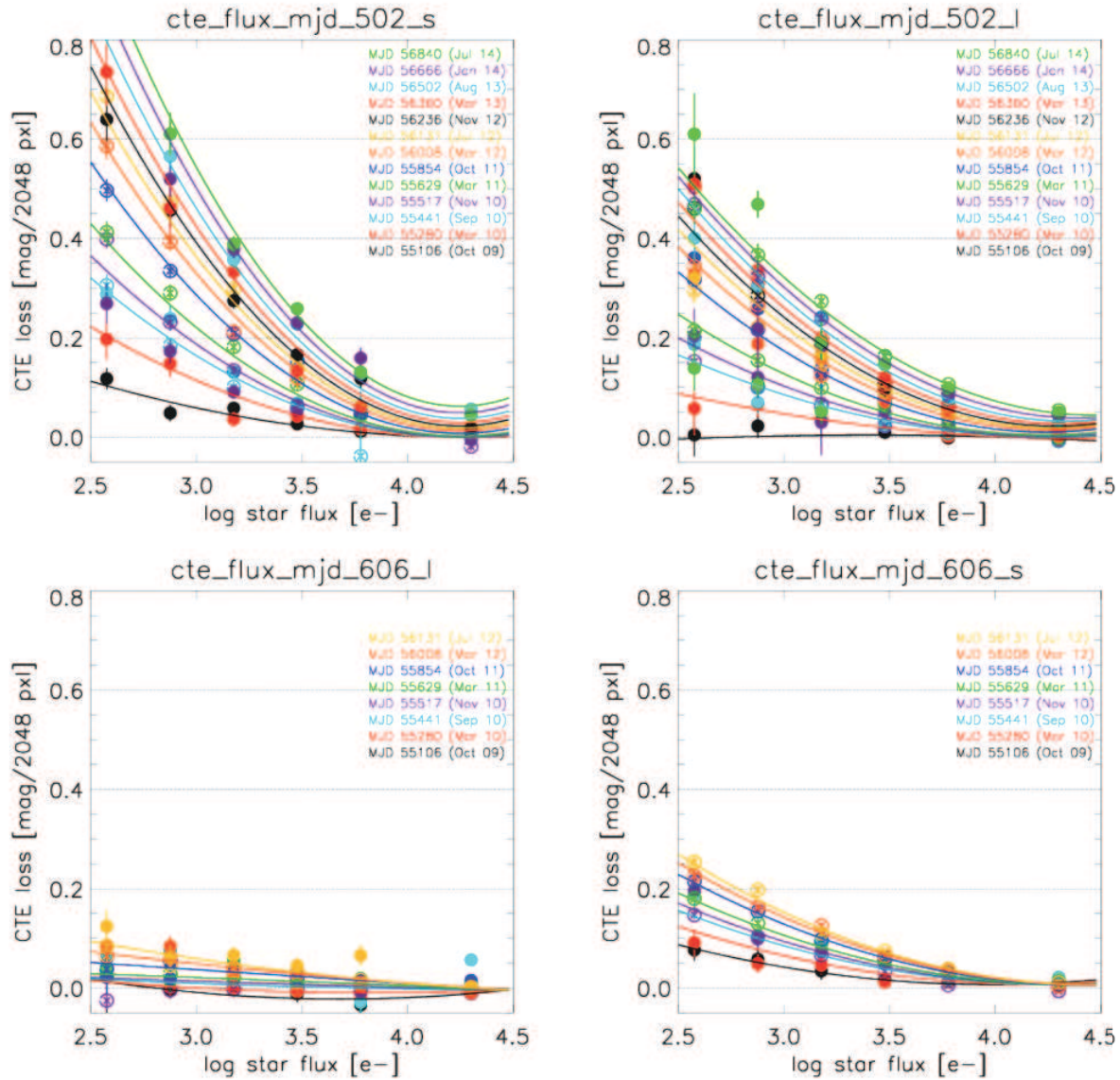
Figure 6.18: CTE Losses as a Function of Star Flux, Observation Date, and Image Background
