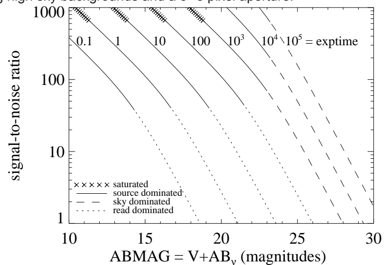
Figure A.188: Point source S/N vs. V+AB_V for the F098M filter, assuming high sky backgrounds and a 3 \times 3 pixel aperture.
