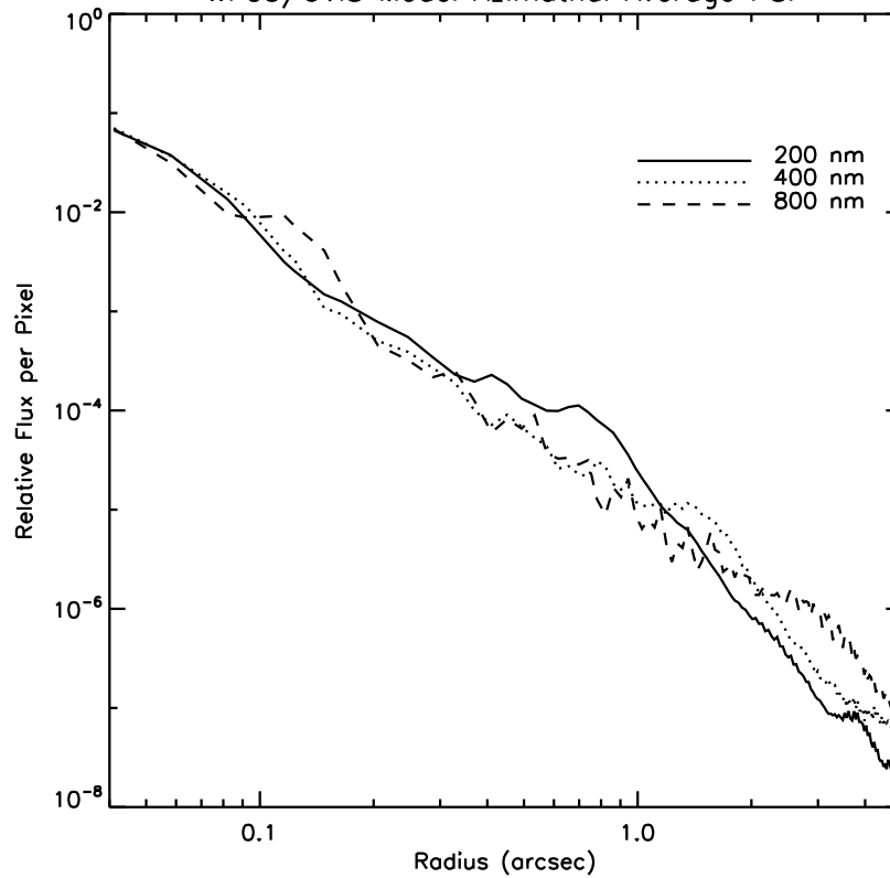
Figure 6.10: Azimuthally averaged mean WFC3/UVIS PSF. WFC3/UVIS Model Azimuthal Average PSF
