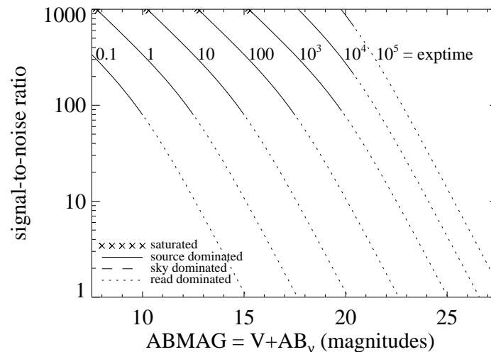
Figure A.99: Extended source S/N vs. V+AB_v for the F665N filter, assuming high sky backgrounds and a source uniformly filling a 1 arcsec 2 aperture.
