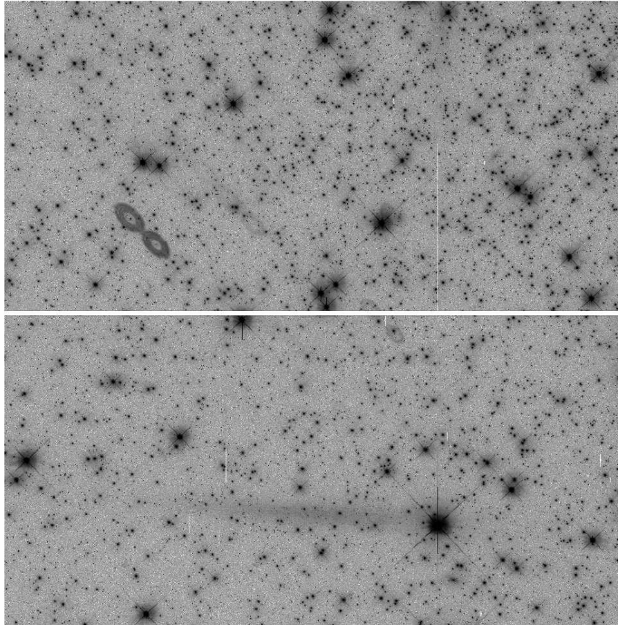
Figure 6.9: UVIS figure-eight window ghosts. An F606W exposure of 47 Tuc (iabj01z7q_fit, display log stretched and saturated) shows figure-8 ghosts well removed along a diagonal from the bright stars in the lower right quadrant that produce them.
