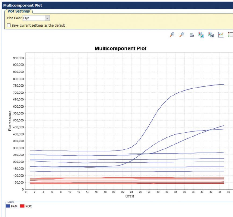
Appendix Figure 1. Amplification and multicomponent plots.
