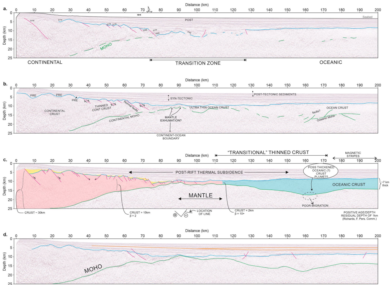
Figure 3. Digitized examples of the different group interpretations. (a) continent-ocean transition (COT) interpretation (group—JJ), with the extent of the transition zone marked by an arrowed section. The Moho is partially interpreted, as is the top of the Basement. (b) continent-ocean boundaries (COB) interpretation (group—KQ). This interpretation includes the continental and oceanic crust, including a section of ultra-thinned ocean crust in between, but also explicitly locates the COB. The Moho is partially interpreted at a distance of 110–160 km. (c) COT interpretation (group—JQ). The interpretation uses annotation to show the extent of “transitional” thinned crust; the thickness of the continental crust and the oceanic crust and associated \beta —stretching factors, as well as other features. (d) The one interpretation (group—JL) that could not be categorized. The interpretation shows the Moho, Top Basement, Faults and sediment fill; but with no identification of oceanic or continental crust, a boundary or a transition zone.
