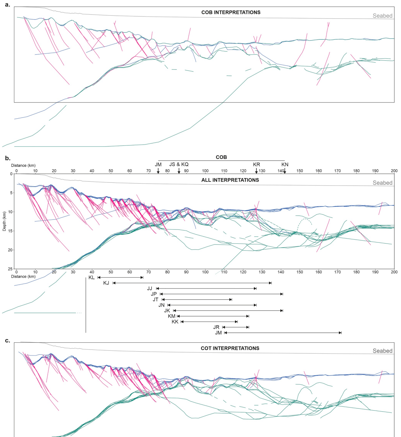
Figure 4. Digitized and stacked group interpretations. (a) The five continent-ocean boundaries (COB) interpretations stacked. (b) All 17 group interpretations stacked. The position of the COB as identified by the five groups is annotated above the stacked interpretations, and the extent of the continent-ocean transition (COT) zone for the 11 COT group interpretations is shown below the stacked interpretations. (c) The 11 COT interpretations stacked. In each subfigure the Moho is green, Top Basement is blue and Faults are magenta.
