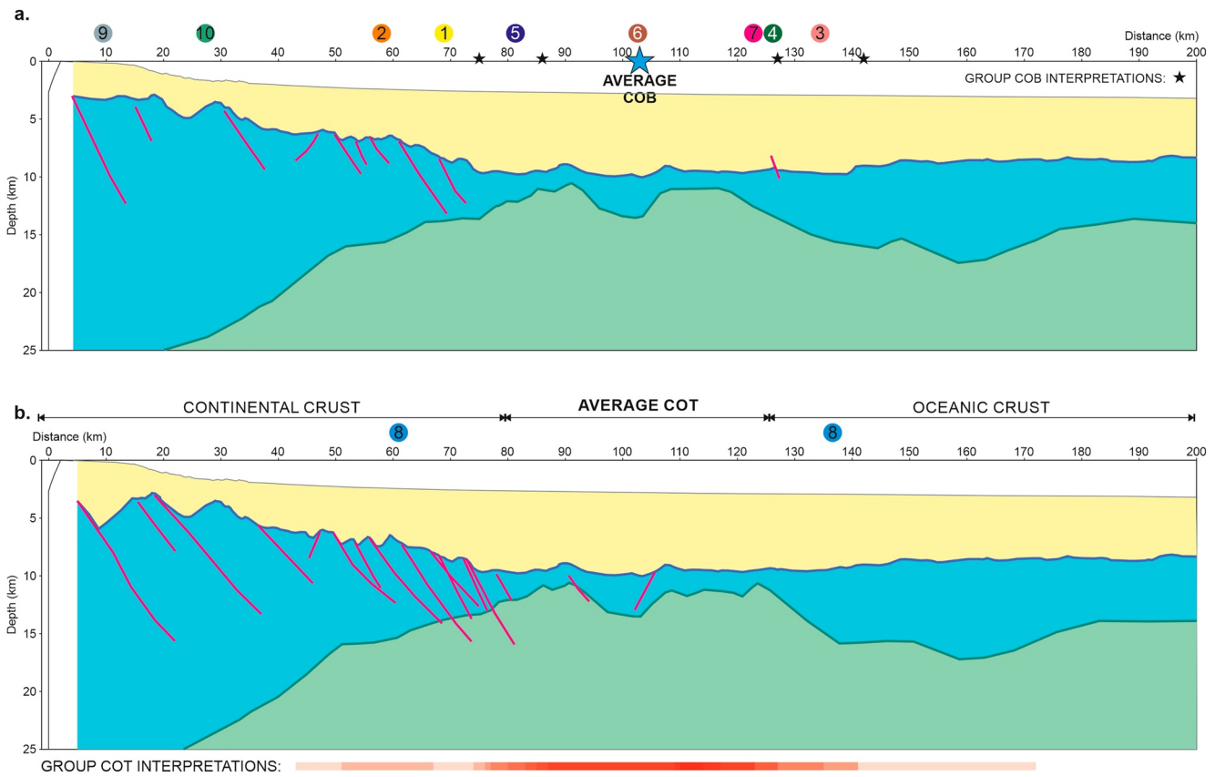
Figure 7. Modal interpretations calculated from all groups for abrupt continent-ocean boundaries (COB) and diffuse continent-ocean transition (COT) models, including the sedimentary units (yellow), the basement (blue) and the upper mantle (green). (a) Modal interpretation calculated from the five COB model interpretations. The position of the average COB is shown with a blue star, individual COB position interpretations are marked with smaller black stars (see also Figure 4b). (b) Modal interpretation calculated from the 11 COT model interpretations (calculated as the average start and average end of the COT interpretations). The extent and position of group interpretations of the COT zone are represented below the section as an intensity color bar, the higher the color intensity (red) the more groups interpreted a transition zone in that portion of the seismic section (see Figure 4b for individual group transition zone extents). Interpretation colors follow previous figures: Moho—green, Top Basement—blue, Faults—magenta. The colored numbers represent the placement of COB and COT interpretations across the East Indian Margin from the published studies outlined in Eagles et al. (2015) and summarized in Figure 1.
