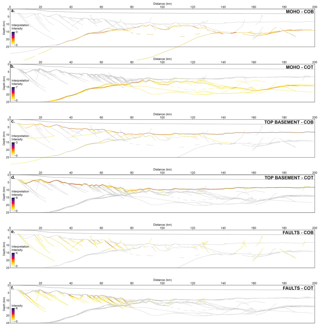
Figure 5. Heat maps of the three elements (Moho, Top Basement, and Faults) that the groups were requested to interpret, split by abrupt continent-ocean boundaries (COB) and diffuse continent-ocean transition (COT) model types. Moho heat maps of the COB (a) and COT (b) interpretations. Top Basement heat maps of the COB (c) and COT (d) interpretations. Fault heat maps of the COB (e) and COT (f) interpretations. In all images, the heat map intensity color bar is scaled to the maximum number of overlapping interpretations in the set for the element of interest. In each instance the other elements interpreted as well as the seabed are shown in pale gray.
