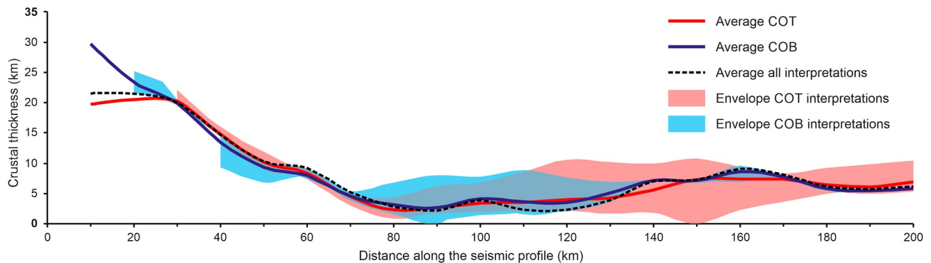
Figure 6. Average crustal thickness interpreted across the section showing the average for all interpretations (dashed line), the average for the diffuse continent-ocean transition (red line) and abrupt continent-ocean boundaries interpretations (blue line) separately, and the envelopes of the range in thickness interpreted. The lack of envelope interpretations at a certain distance along the profile indicates that no more than one interpretation was available. Crustal thicknesses were calculated every 10 km along the seismic section for each interpretation.
