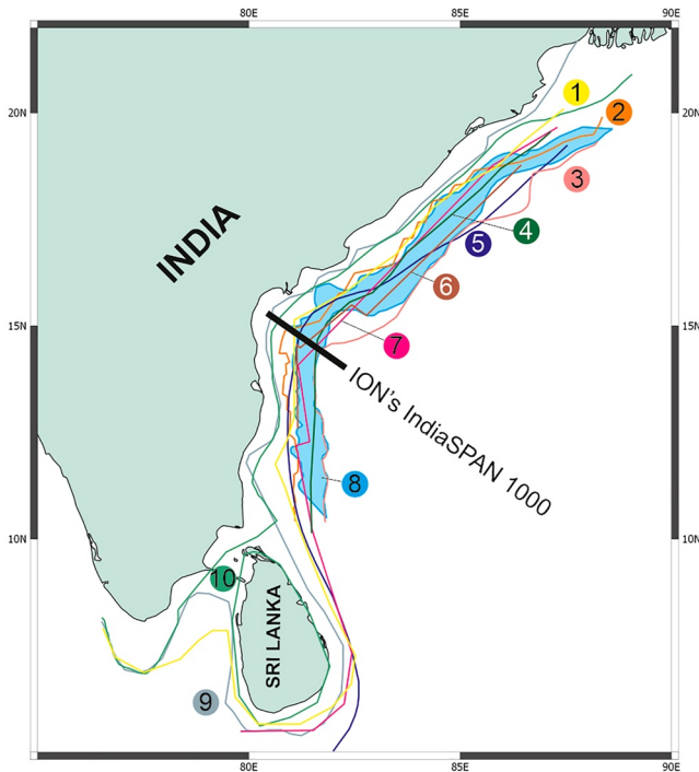
Figure 1. The East Indian margin with the location of the ION's IndiaSPAN 1000 marked, and data showing the location of continent-ocean boundaries and continent-ocean transition interpretations redrawn from Eagles et al. (2015). The numbers indicate the interpretation sources as follow: (1) Bouysse et al. (2009); (2) Bastia et al. (2010); (3) Sinha et al. (2010); (4) Rao et al. (1997); (5) Krishna et al. (2009); (6) Veevers (2009); (7) Powell et al. (1988); (8) Nemčok et al. (2013); (9) Gibbons et al. (2013); (10) Seton et al. (2012). Note that the numbers in this figure do not correspond to the number codes in Eagles et al. (2015).
