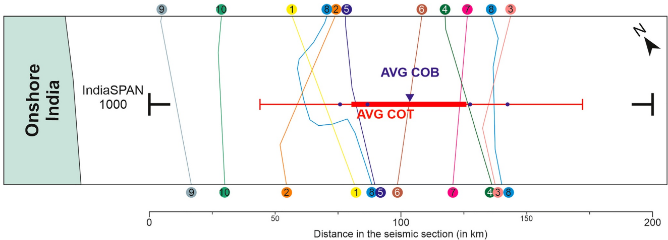
Figure 8. Schematic map view of the placement of abrupt continent-ocean boundaries (COB) and diffuse continent-ocean transition (COT) interpretations across the East Indian Margin from the published studies outlined in Eagles et al. (2015) and summarized in Figure 1. Numbers refer to the different publications (see Figure 1 caption). Analysis of the 17 group interpretations elicited in this study are represented by an average COB mark (blue triangle), the positions of the COB interpretations (blue circles), the average COT range (calculated as the average start and average end of the COT interpretations, thick red line) and the range of COT interpretations (red whiskers).
