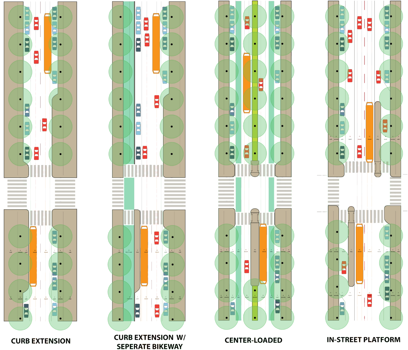
Figure 2.7: Potential Streetcar Loading Options
