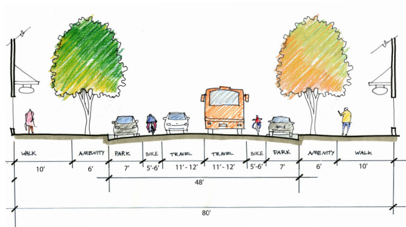
Figure 2.6: Transit Priority Typology, 2- and 3-lane
