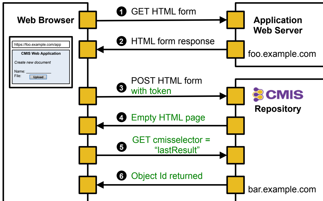
Figure 5.2: Selector "lastResult" returns the last service result from the repository
