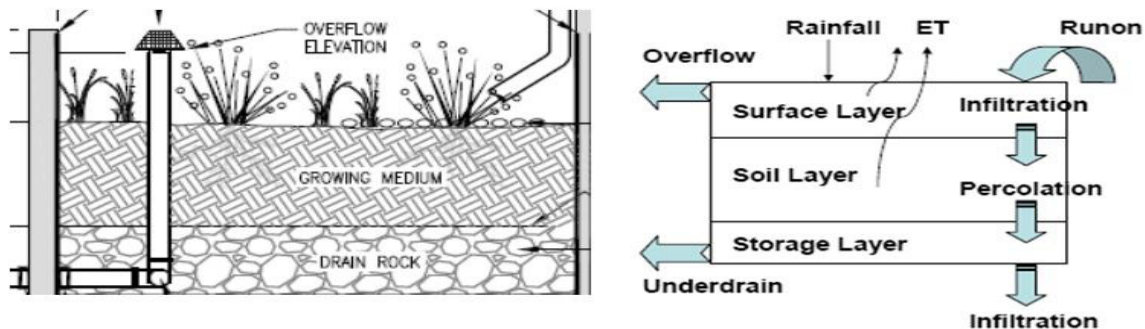
Figure 32. Conceptual representation of a bio-retention cell.
