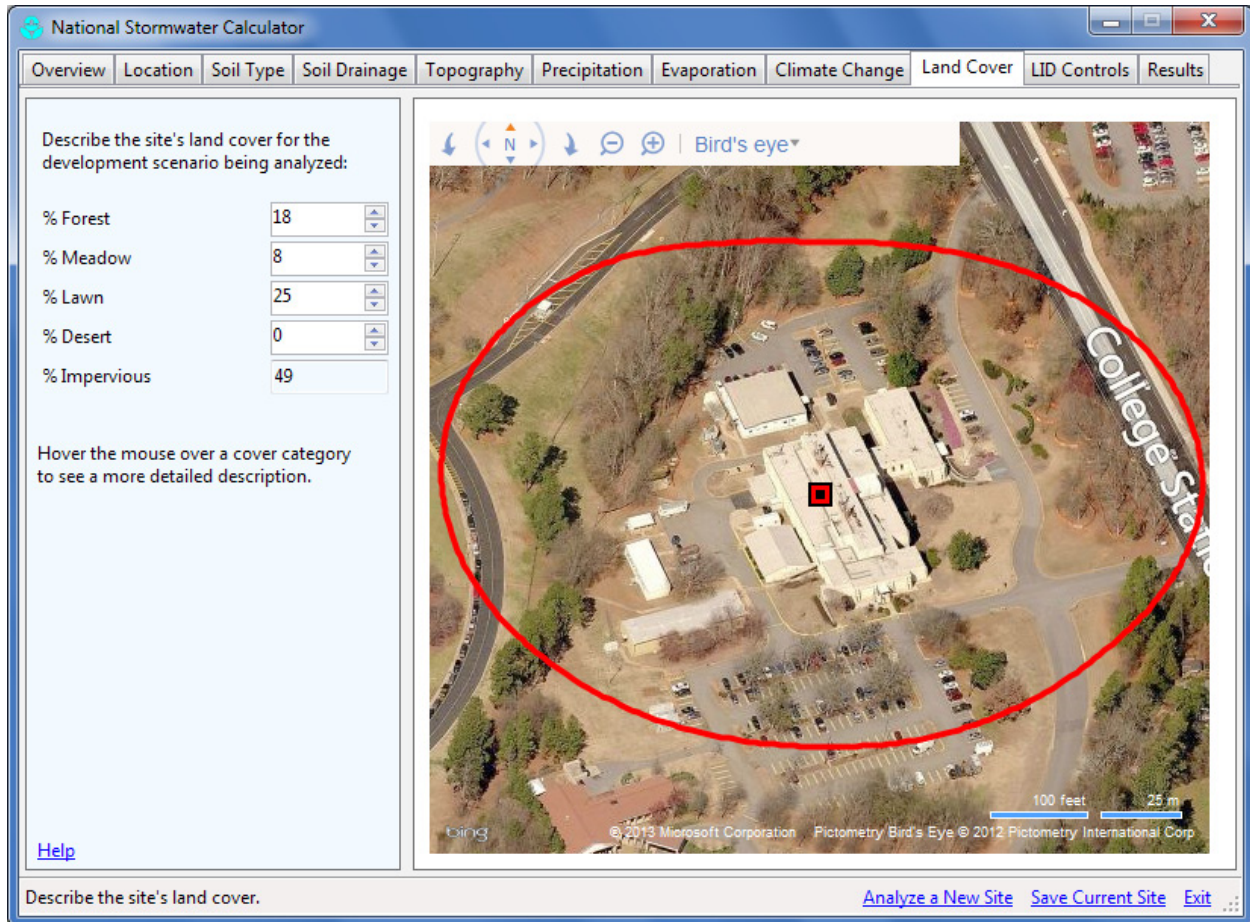
Figure 10. The calculator’s Land Cover page.
