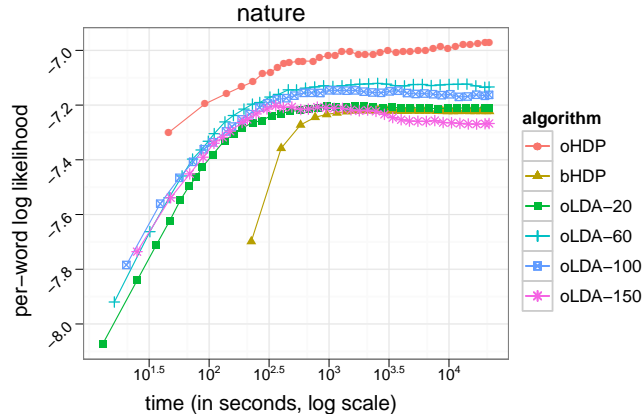
Figure 3: Experimental results on Nature with \kappa = 0.6 and batch size S = 256 (for the online algorithms). Points are sub-sampled for better view. The label “oLDA-20” indicates online LDA with 20 topics. (Not all numbers of topics are shown; see Figure 4 for more details.) Online HDP performs better than online LDA and batch HDP.
