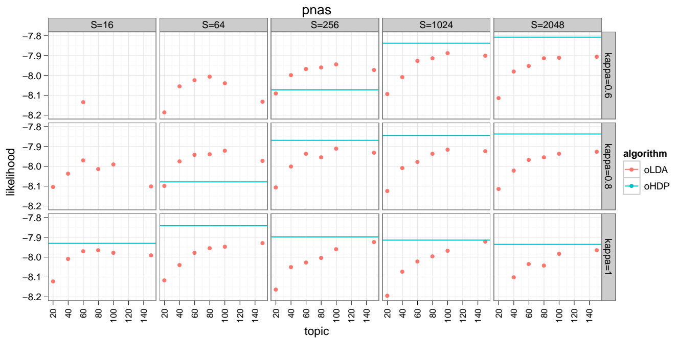
Figure 6: Comparisons of online LDA and online oHDP on the PNAS corpus under various settings of batch size S and parameter \kappa (kappa), run for 6 hours each. (Some lines for online HDP and points for online LDA do not appear due to figure limits.) The best result among all is achieved by online HDP.
