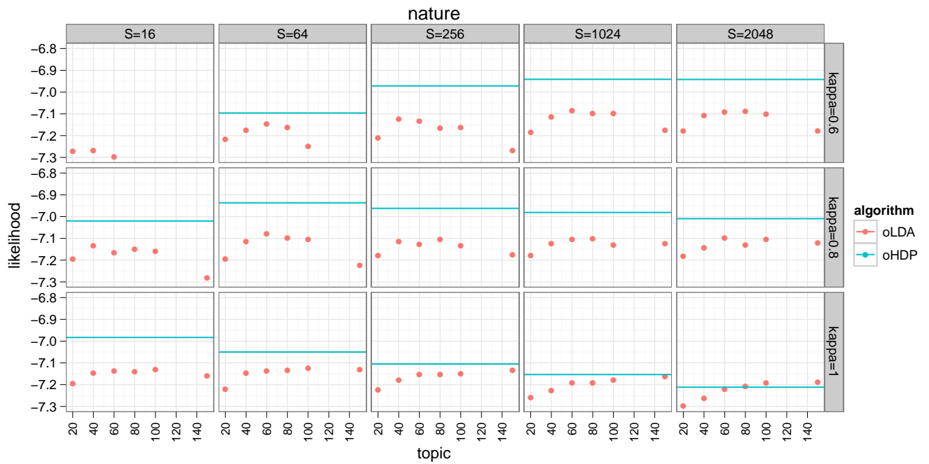
Figure 4: Comparisons of online LDA and online HDP on the Nature corpus under various settings of batch size S and parameter \kappa (kappa), run for 6 hours each. (Some lines for online HDP and points for online LDA do not appear due to figure limits.) The best result among all is achieved by online HDP.
