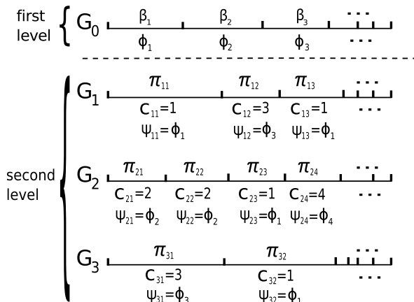
Figure 1: Illustration of the Sethuraman’s stick-breaking construction of the two-level HDP. In the first level, \phi_k \sim H and \beta \sim \text{GEM}(\gamma) ; in the second level, \pi_j \sim \text{GEM}(\alpha_0) , c_{jt} \sim \text{Mult}(\beta) and \psi_{jt} = \phi_{c_{jt}} .
