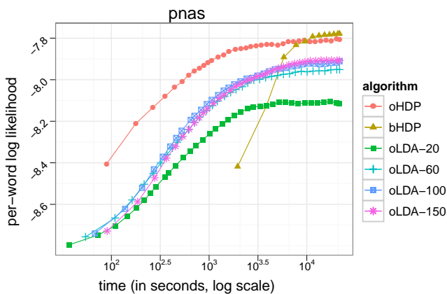
Figure 5: Experimental results on PNAS \kappa = 0.6 and batch size S = 2048 (for the online algorithms). Points are subsampled for better view. (Not all numbers of topics are shown, please see Figure 6 for more details.) Online HDP performs better than online LDA, and slightly worse than batch HDP. Unlike in the Nature experiment, batch HDP is trained on the whole training set.
