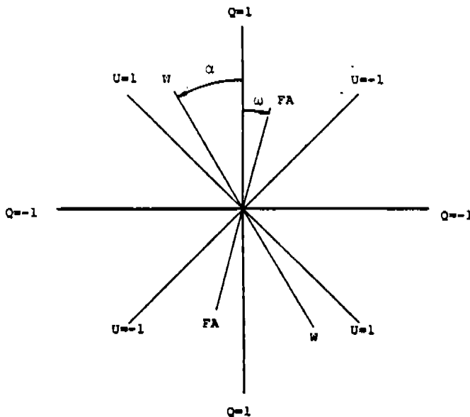
Figure 1. Coordinate system used in the polarization analysis. The view is toward the source. The line W-W is the pass direction of the Wollaston; while FA-FA is the fast axis of the waveplate.
