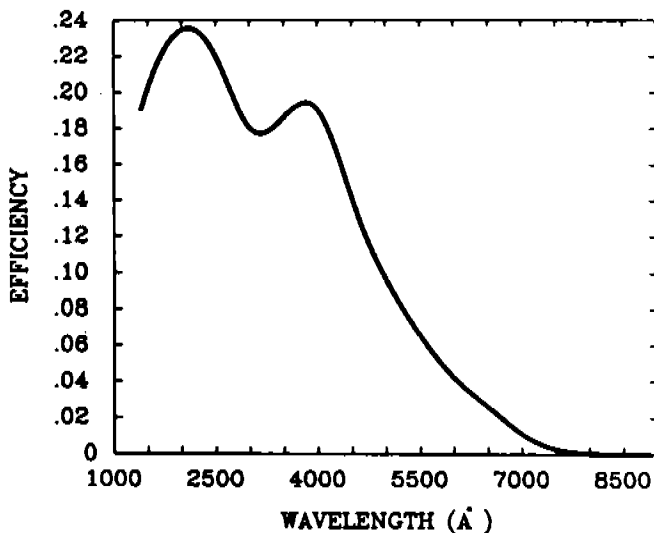
RED DIGICON (F8) QUANTUM EFFICIENCY
