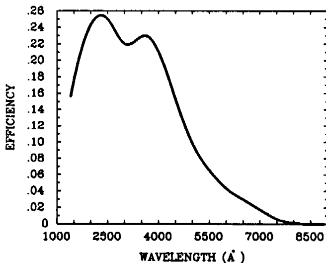
Figure 2.2.4-1 Digicon quantum efficiencies as a function of wavelength (courtesy of Ed Beaver and George Hartig).
