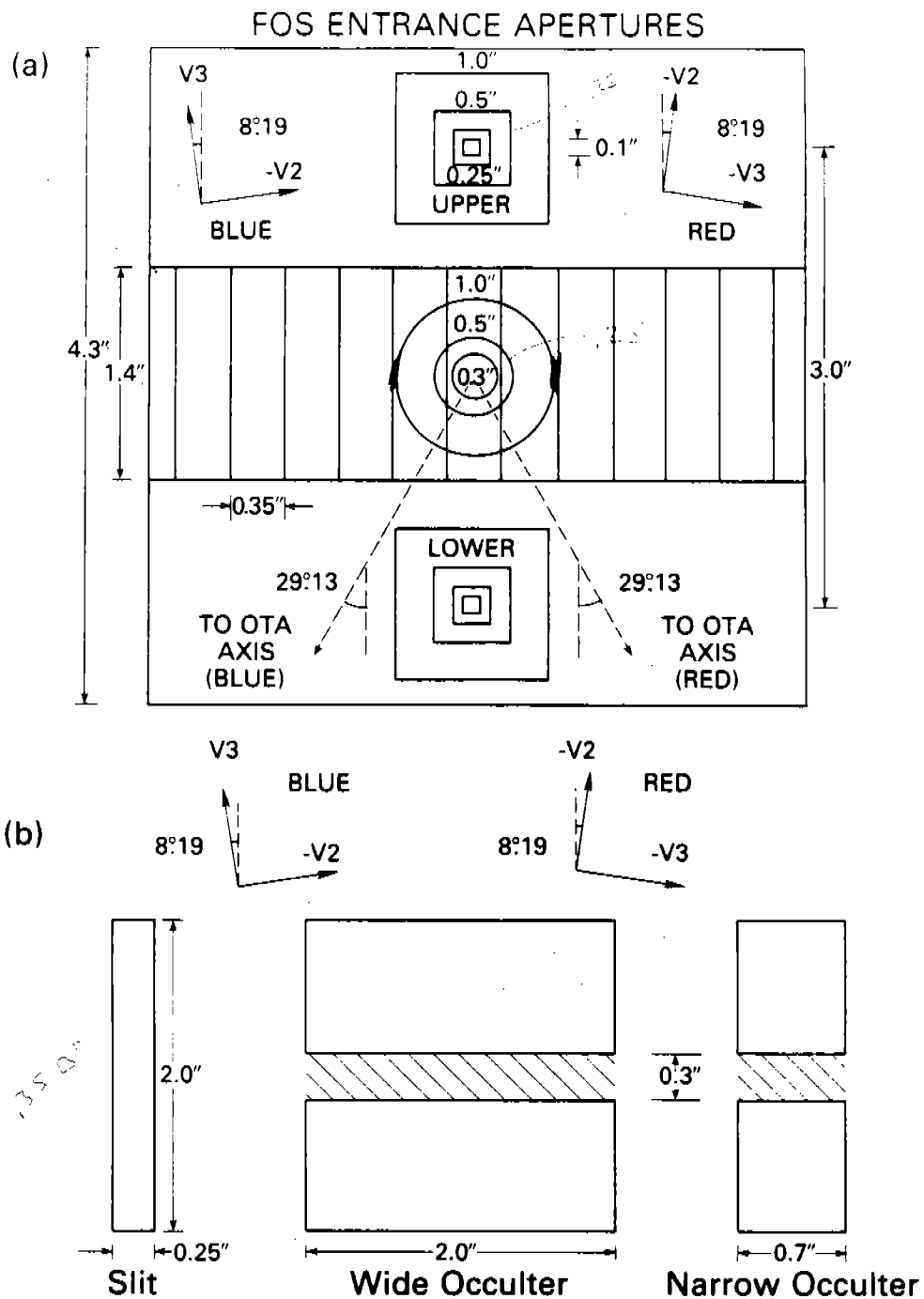
Figure 2.2.1-1 A Schematic of the FOS Apertures projected onto the sky. The upper panel shows the array of 0.35'' \times 1.4'' diodes projected across the center of the 4.3'' \times 4.3'' target acquisition aperture. The target acquisition aperture and the single circular apertures position to a common center. The pairs of square apertures position to common centers with respect to the target acquisition aperture as shown in the figure. Either the upper aperture (the "A" aperture, which is furthest from the HST optical axis) or the lower aperture (the "B" aperture, which is closest to the HST optical axis) in a pair can be selected by an appropriate y-deflection in the Digicon detectors. The lower panel shows the three rectangular slits; two of the slits are bisected by an 0.3'' opaque occulting bar. The centers of the three slits position to the center of the target acquisition aperture. The figure shows the orientation of the direction perpendicular to the dispersion in the HST V2, V3 focal plane on the blue and red sides. The FOS x-axis is parallel to the diode array and positive to the right; the y-axis is perpendicular to the diode array and positive toward the upper aperture.
