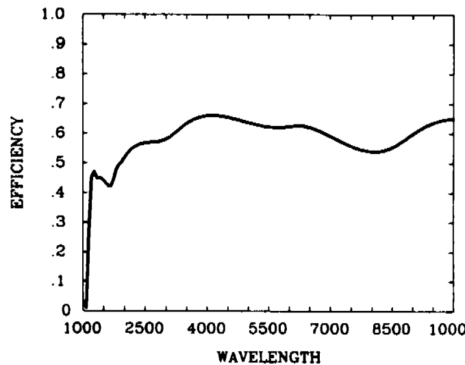
ASSUMED SPACE TELESCOPE EFFICIENCY
