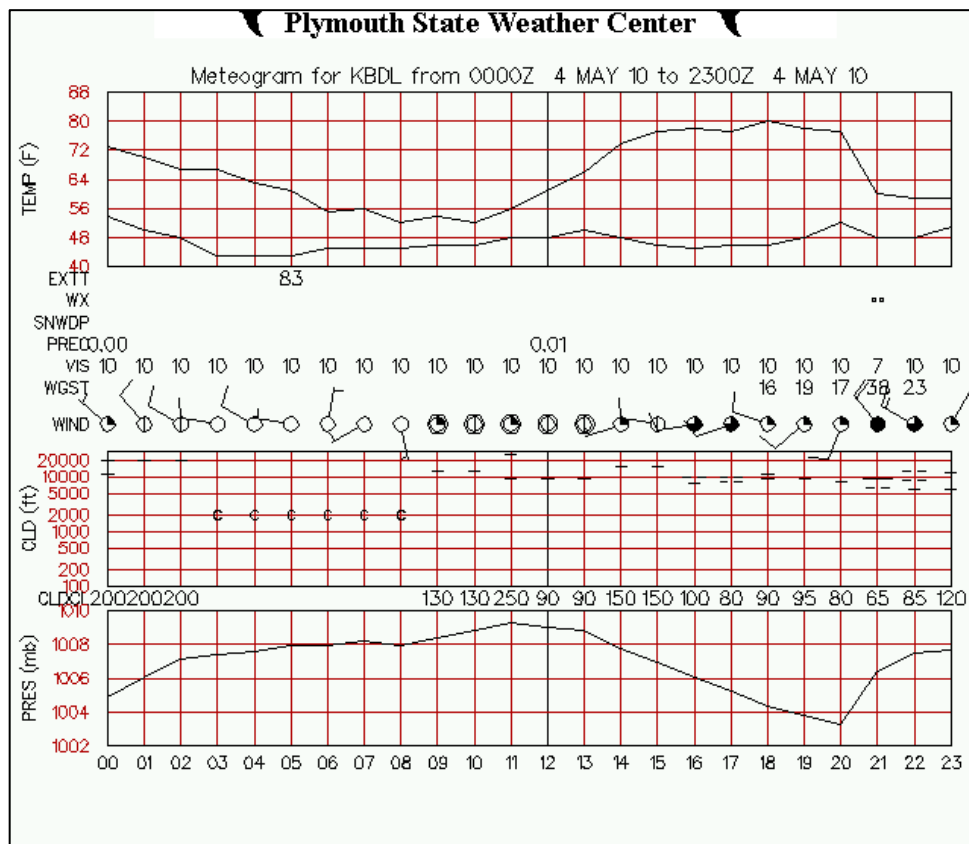
Figure 3.51. Meteogram for BDL valid from 0000 UTC 4 May 2010 to 2300 UTC 4 May 2010. Wind speeds are in knots (source: Plymouth State College).
