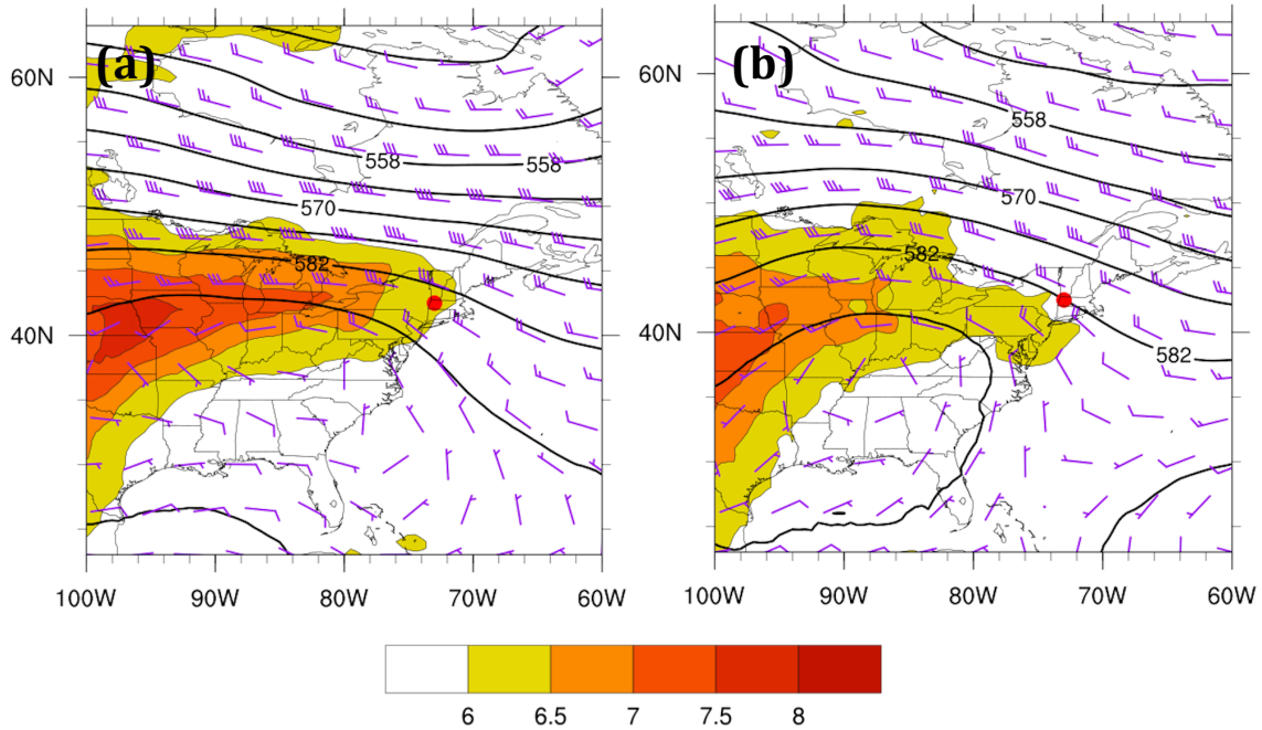
Figure 3.20. Northwesterly flow category composite 500-hPa geopotential height (black contours, dam), wind barbs (kt), and 700–500-hPa lapse rate (fills, K km -1 ), for good (a) events (N = 20) and type 1 (b) events (N = 29). Heavy red dot represents composite center at point of maximum report density.
