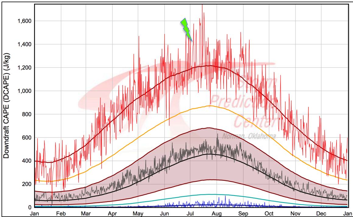
Figure 3.67. As in Fig. 3.39 but for PIT. Green bolt represents observed value at 1200 UTC 4 July 2012 (source: SPC).
