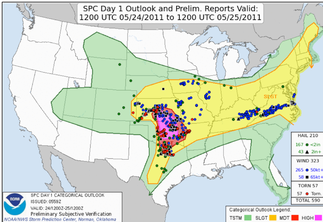
Figure 3.73. SPC 0600 UTC 24 May 2011 severe wind convective outlook valid 1200 UTC 24 May 2011 to 1200 UTC 25 May 2011.
