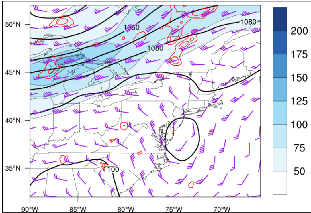
Figure 3.34. 250-hPa geopotential height (black contours, dam), divergence (red contours every 5 \times 10^{-5} \text{ s}^{-1} starting at 10 \times 10^{-5} \text{ s}^{-1} ), wind speed (fills, kt), and wind barbs (kt) at 1600 UTC 18 August 2009 using RUC model analysis data.
