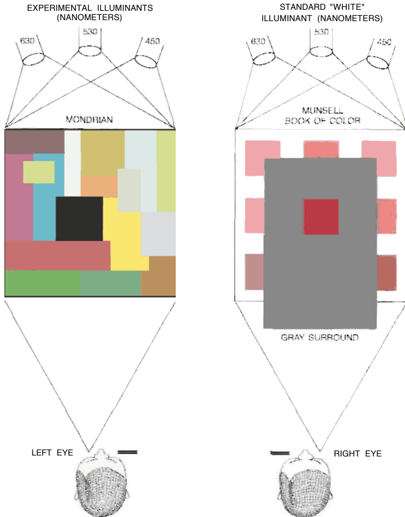
COLOR-MATCHING EXPERIMENT uses a simplified Mondrian of 17 color areas (left) and a standard color reference, The Munsell Book of Color , which contains 1150 color "chips" (right). The Mondrian is illuminated with three narrow-band light sources: one at 630 nanometers (long-wave light), one at 530 nanometers (middle-wave light) and one at 450 nanometers (short-wave light). The ratio of the three illuminants can be adjusted so that the triplet of energies reflected to the eye from any chosen area will exactly equal the triplet that previously reached the eye from some other area. In this experiment five areas, gray, red, yellow, blue and green, were selected in sequence to send the same triplet of energies to the eye. In each of the five consecutive parts of this experiment the observer selected from the Munsell book the chips that came closest to matching the 17 areas of the Mondrian. The Munsell book was illuminated throughout the experiment with a constant spectral mixture of three narrow-band lights adjusted at the outset so that the white Munsell chip appeared the "best white." The experiment was set up so that the observers used one eye for viewing the Mondrian and the other eye for viewing chips. Gray paper with an opening was used to provide chips with a constant surround.
