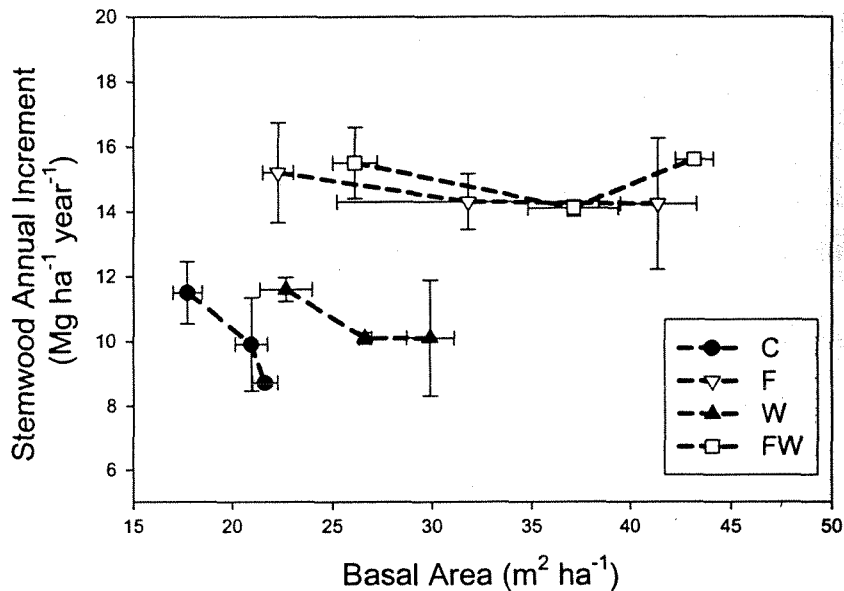
Fig. 12. Relationship between stemwood annual increment and basal area at the beginning of the growing season for loblolly pine stands on the lower coastal plain of Georgia. C: stands receiving mechanical site preparation only, W: stands receiving complete control of interspecific vegetation in addition to mechanical site preparation, F: stands receiving annual fertilization in addition to mechanical site preparation, and FW: stands receiving both competition control and annual fertilization in addition to mechanical site preparation. Vertical bars represent standard errors.
