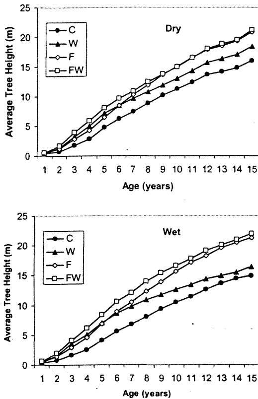
Fig. 2. Average height through 15 growing seasons for loblolly pine stands on the lower coastal plain. C: stands receiving mechanical site preparation only, W: stands receiving complete control of interspecific vegetation in addition to mechanical site preparation, F: stands receiving annual fertilization in addition to mechanical site preparation, and FW: stands receiving both competition control and annual fertilization in addition to mechanical site preparation.
