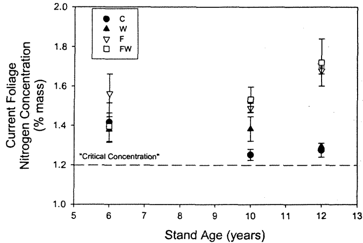
Fig. 9. Dormant season foliar nitrogen concentration of different aged loblolly pine stands growing on the lower coastal plain of Georgia. C: stands receiving mechanical site preparation only, W: stands receiving complete control of interspecific vegetation in addition to mechanical site preparation, F: stands receiving annual fertilization in addition to mechanical site preparation, and FW: stands receiving both competition control and annual fertilization in addition to mechanical site preparation vertical bars represent standard errors.
