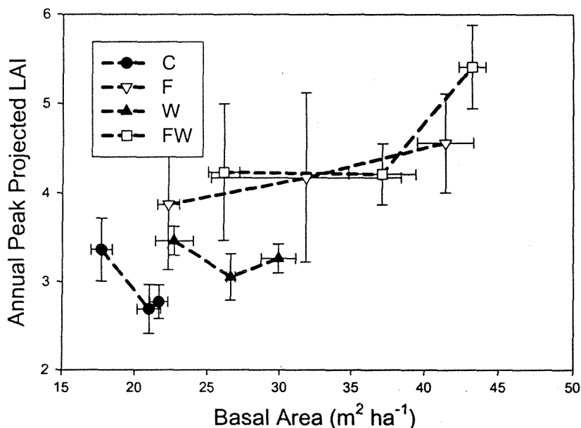
Fig. 11. Relationship between peak leaf area index (LAI) and basal area at the beginning of the growing season for loblolly pine stands on the lower coastal plain of Georgia. C: stands receiving mechanical site preparation only, W: stands receiving complete control of interspecific vegetation in addition to mechanical site preparation, F: stands receiving annual fertilization in addition to mechanical site preparation, and FW: stands receiving both competition control and annual fertilization in addition to mechanical site preparation. Vertical bars represent standard errors.
