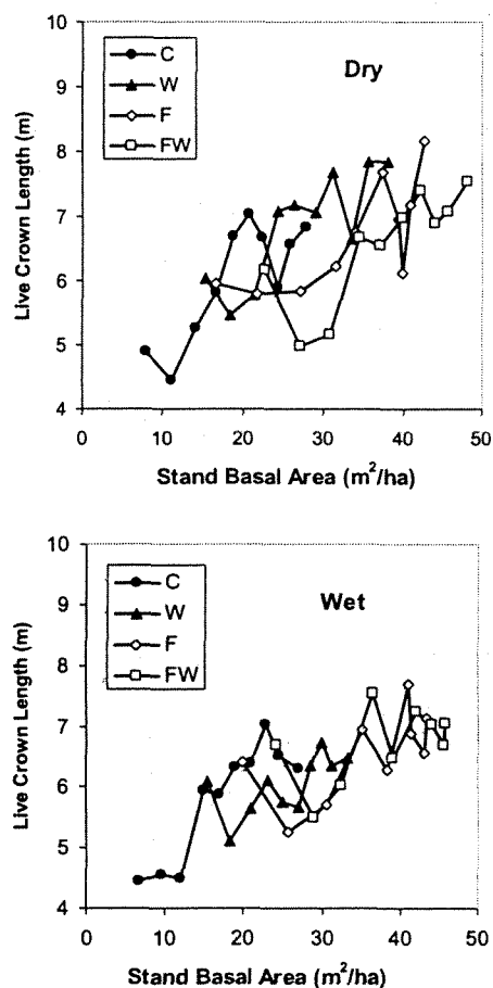
Fig. 5. Average live crown length vs. stand basal area for loblolly pine on the lower coastal plain. C: stands receiving mechanical site preparation only, W: stands receiving complete control of interspecific vegetation in addition to mechanical site preparation, F: stands receiving annual fertilization in addition to mechanical site preparation, and FW: stands receiving both competition control and annual fertilization in addition to mechanical site preparation.
