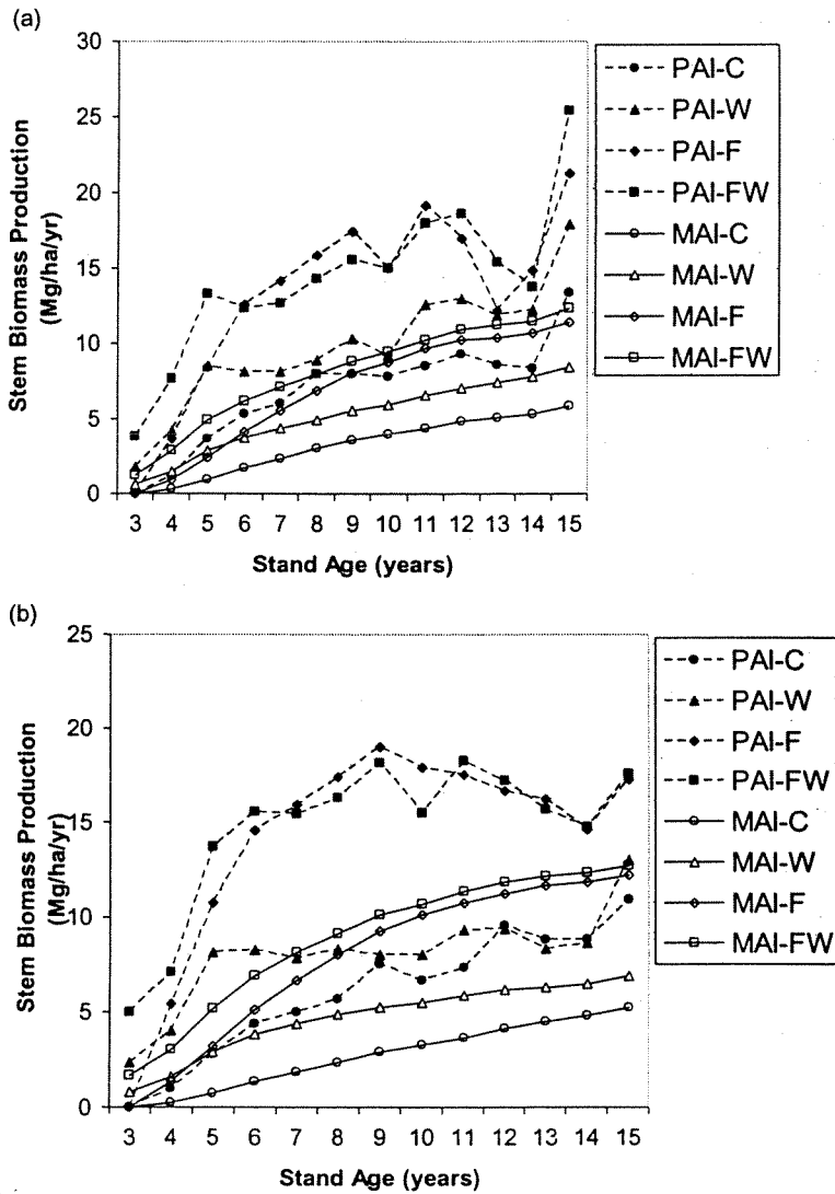
Fig. 7. (a) Mean and periodic (1 year) annual increment of stem biomass for plantations for loblolly pine on the lower coastal plain of Georgia for the dry site. C: stands receiving mechanical site preparation only, W: stands receiving complete control of interspecific vegetation in addition to mechanical site preparation, F: stands receiving annual fertilization in addition to mechanical site preparation, and FW: stands receiving both competition control and annual fertilization in addition to mechanical site preparation. (b) Mean and periodic (1 year) annual increment of stem biomass for plantations for loblolly pine on the lower coastal plain of Georgia for the wet site. C: stands receiving mechanical site preparation only, W: stands receiving complete control of interspecific vegetation in addition to mechanical site preparation, F: stands receiving annual fertilization in addition to mechanical site preparation, and FW: stands receiving both competition control and annual fertilization in addition to mechanical site preparation.
