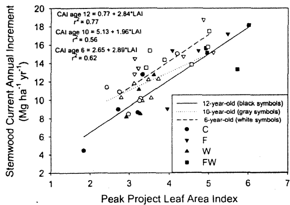
Fig. 13. Relationship between peak leaf area index and stemwood current annual increment for loblolly pine stands growing on the lower coastal plain of Georgia. C: stands receiving mechanical site preparation only, W: stands receiving complete control of interspecific vegetation in addition to mechanical site preparation, F: stands receiving annual fertilization in addition to mechanical site preparation, and FW: stands receiving both competition control and annual fertilization in addition to mechanical site preparation.
