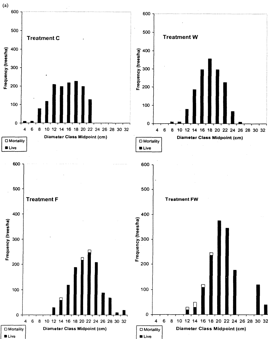
Fig. 4. (a) Diameter distribution bar graphs by treatment for loblolly pine on the lower coastal plain dry site. C: stands receiving mechanical site preparation only, W: stands receiving complete control of interspecific vegetation in addition to mechanical site preparation, F: stands receiving annual fertilization in addition to mechanical site preparation, and FW: stands receiving both competition control and annual fertilization in addition to mechanical site preparation. (b) Diameter distribution bar graphs by treatment for loblolly pine on the lower coastal plain dry site. C: stands receiving mechanical site preparation only, W: stands receiving complete control of interspecific vegetation in addition to mechanical site preparation, F: stands receiving annual fertilization in addition to mechanical site preparation, and FW: stands receiving both competition control and annual fertilization in addition to mechanical site preparation.
