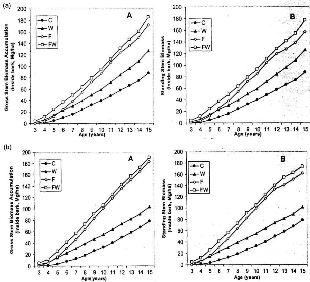
Fig. 6. (a) Gross (A) and standing (B) stem wood biomass (dry mass, inside bark, no branches) vs. stand age for the loblolly pine on the lower coastal plain of Georgia for the dry site. C: stands receiving mechanical site preparation only, W: stands receiving complete control of interspecific vegetation in addition to mechanical site preparation, F: stands receiving annual fertilization in addition to mechanical site preparation, and FW: stands receiving both competition control and annual fertilization in addition to mechanical site preparation. (b) Gross (A) and standing (B) stem wood biomass (dry mass, inside bark, no branches) vs. stand age for loblolly pine on the lower coastal plain of Georgia for the wet site. C: stands receiving mechanical site preparation only, W: stands receiving complete control of interspecific vegetation in addition to mechanical site preparation, F: stands receiving annual fertilization in addition to mechanical site preparation, and FW: stands receiving both competition control and annual fertilization in addition to mechanical site preparation.
