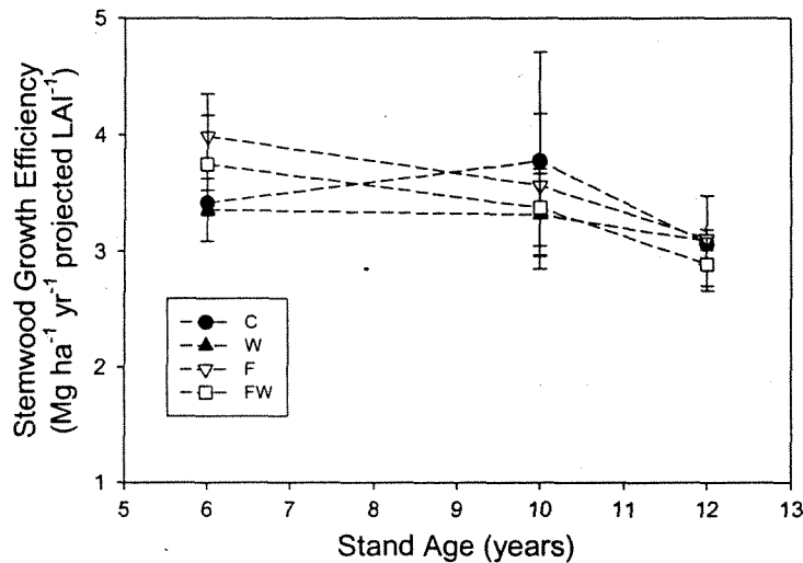
Fig. 14. Growth efficiency for different aged loblolly pine stands growing on the lower coastal plain of Georgia. C: stands receiving mechanical site preparation only, W: stands receiving complete control of interspecific vegetation in addition to mechanical site preparation, F: stands receiving annual fertilization in addition to mechanical site preparation, and FW: stands receiving both competition control and annual fertilization in addition to mechanical site preparation estimates based on peak leaf area. Vertical bars represent standard errors.
