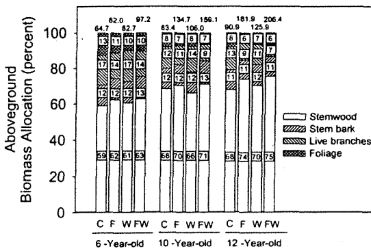
Fig. 10. Partitioning of standing aboveground biomass of different aged loblolly pine stands growing on the lower coastal plain of Georgia. C: stands receiving mechanical site preparation only, W: stands receiving complete control of interspecific vegetation in addition to mechanical site preparation, F: stands receiving annual fertilization in addition to mechanical site preparation, and FW: stands receiving both competition control and annual fertilization in addition to mechanical site preparation estimates based on peak leaf biomass. Numbers above the bars represent total biomass (Mg ha -1 ). Numbers within the boxes are percentage of total biomass in each component.
