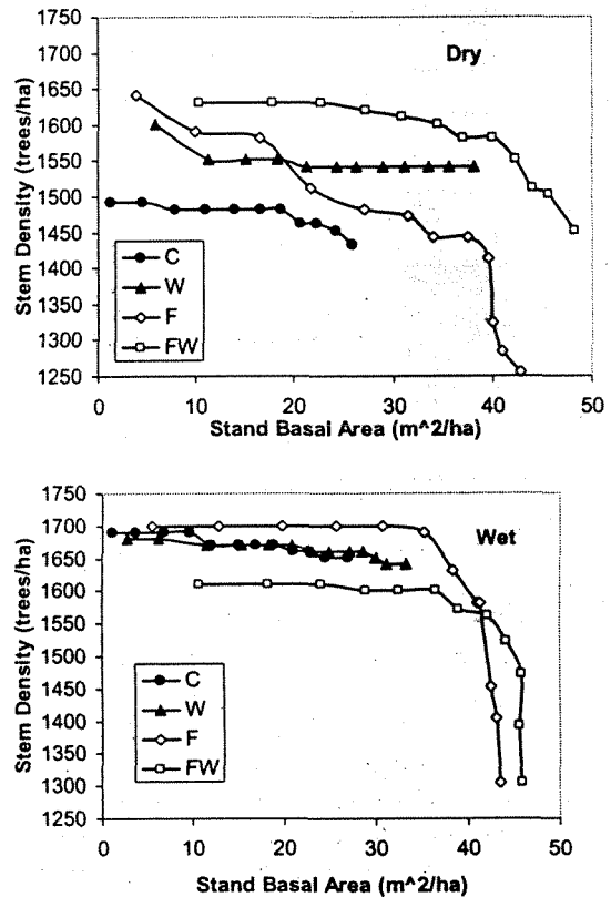
Fig. 3. Stem density vs. stand basal area for loblolly pine stands on the lower coastal plain. C: stands receiving mechanical site preparation only, W: stands receiving complete control of interspecific vegetation in addition to mechanical site preparation, F: stands receiving annual fertilization in addition to mechanical site preparation, and FW: stands receiving both competition control and annual fertilization in addition to mechanical site preparation.
