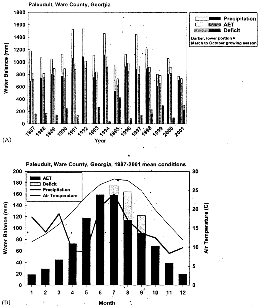
Fig. 1. Water balance estimates for plots within the consortium for accelerated pine productivity studies (CAPPS) located in the Dixon State Forest, Waycross, GA. Climatological data for 1987–2001 are from Alma, GA approximately 18 miles north of Waycross (Georgia Automated Environmental Monitoring Network, 2001). Potential evapotranspiration was estimated using the approach of Thornthwaite and Mather (1957) and soil moisture storage was taken as 100 mm for the upper 1 m of soil. Annual precipitation, actual evapotranspiration (AET), and water deficit for all years of plantation growth are in (A) and mean monthly values over the course of the experiment are in (B).
