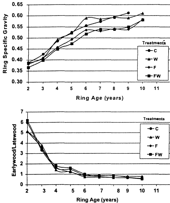
Fig. 8. Specific gravity and earlywood/latewood ratio by ring age for loblolly pine on the lower coastal plain. C: stands receiving mechanical site preparation only, W: stands receiving complete control of interspecific vegetation in addition to mechanical site preparation, F: stands receiving annual fertilization in addition to mechanical site preparation, and FW: stands receiving both competition control and annual fertilization in addition to mechanical site preparation.
