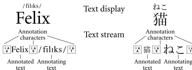
Figure 16-4. Annotation Characters
