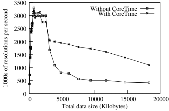
(a) File system results for uniform directory popularity.
