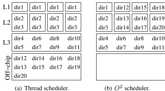
Figure 2: Possible cache contents for the directory lookup workload when using a thread scheduler and an O^2 scheduler. Directories in the “off-chip” box must be loaded from DRAM.
