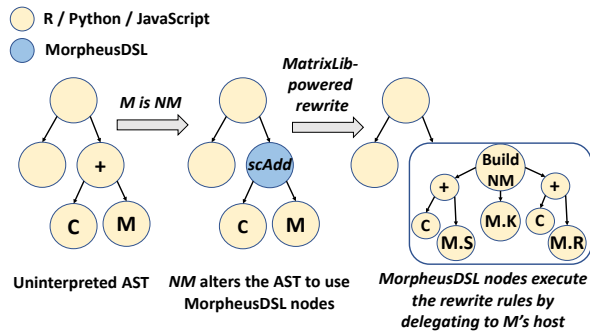
Figure 5: MorpheusDSL dynamically factorizes ML algorithms. C refers to some numeric constant, M refers to some matrix datatype and NM refers to the adapted Normalized Matrix. The rewrite occurs by using the host language’s own LA operator implementations
