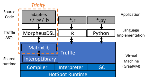
Figure 2: Trinity in and for GraalVM (Section 3 explains more). GraalVM supports many host PLs, they execute on a shared runtime Truffle, which provides services such as dynamic compilation and memory management. Truffle also provides interoperability services across PLs. We build two such services in Trinity to achieve our goals: MatrixLib (Section 4) and MorpheusDSL (Section 5).
