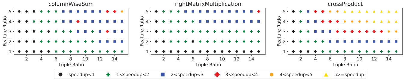
Figure 7: Discretized speedups of Trinity over Materialized in FastR .
