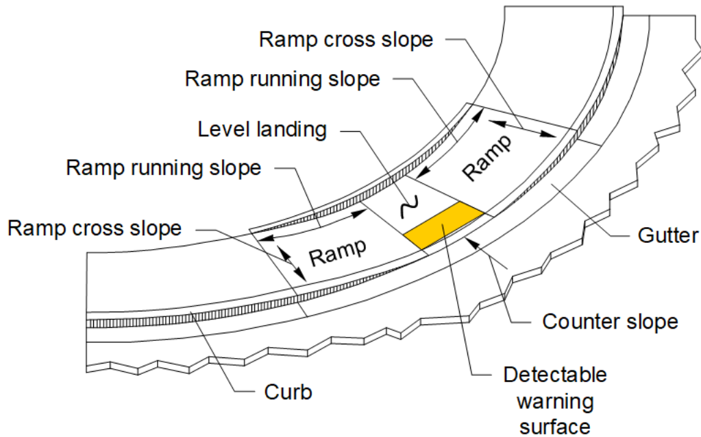
Exhibit 1510-18 Parallel Curb Ramp Common Elements
