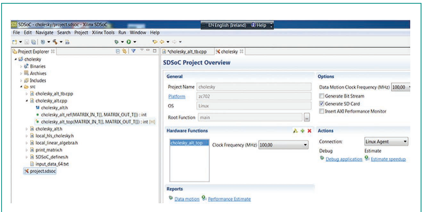
Figure 4 — Setting the hardware accelerator core and its clock frequency from the SDSoC project page
