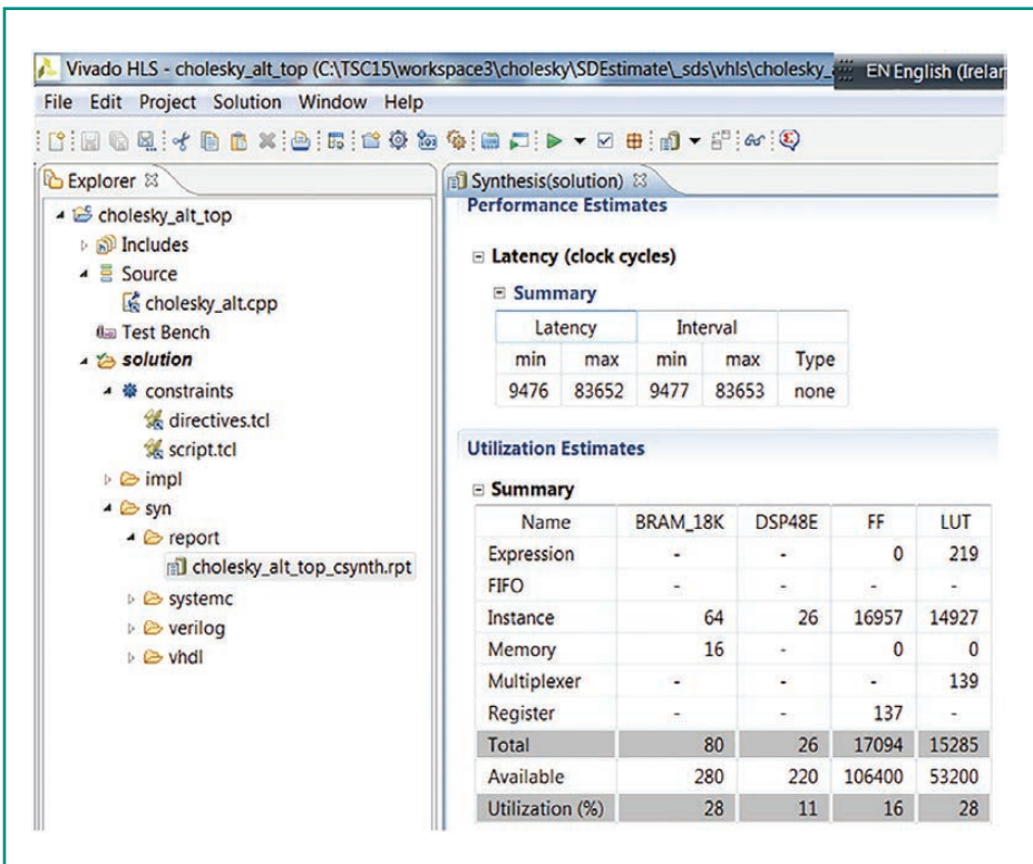
Figure 6: Vivado HLS synthesis estimation report
