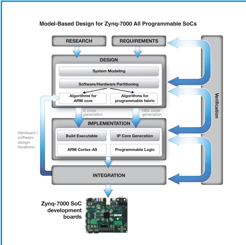
Figure 1 — Designers can create models in Simulink that represent a complete dynamic system and create hardware-software implementations for Zynq SoCs directly from the model.
