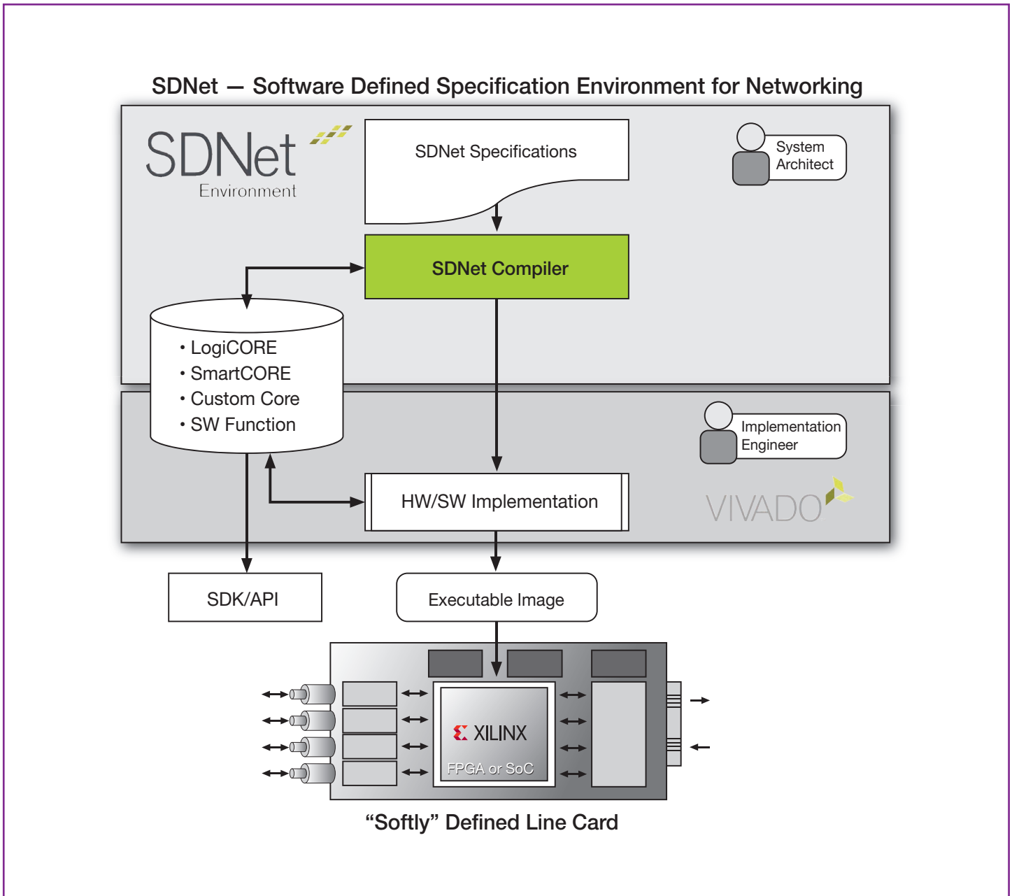
Figure 4 — The SDNet environment enables network architects to create a specification in a C-like language. After a hardware team completes the design, developers can use SDNet to update or add protocols to the card in the field.
