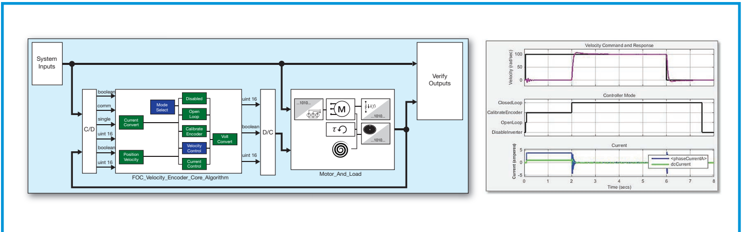
Figure 3 — This control-loop model for a motor control system with simulation results shows the response to a velocity pulse command.
