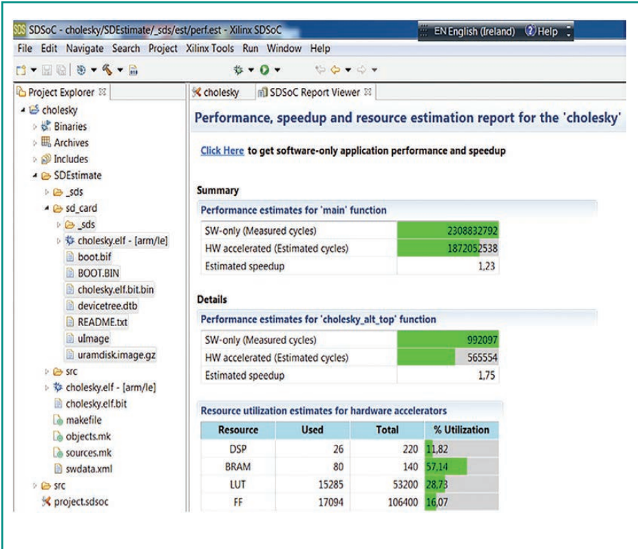
Figure 5 — SDSoC-generated performance, speedup and resources estimation report
