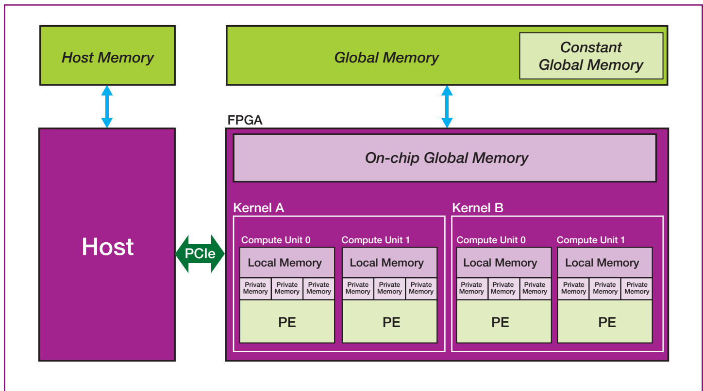
Figure 2 — The OpenCL memory model defines a single memory hierarchy for application development.
