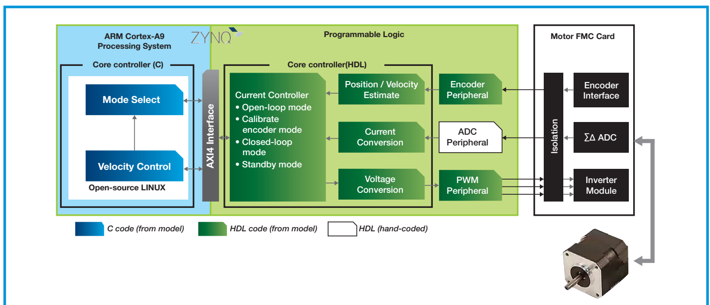
Figure 2 — The motor control system model includes two primary subsystems.
