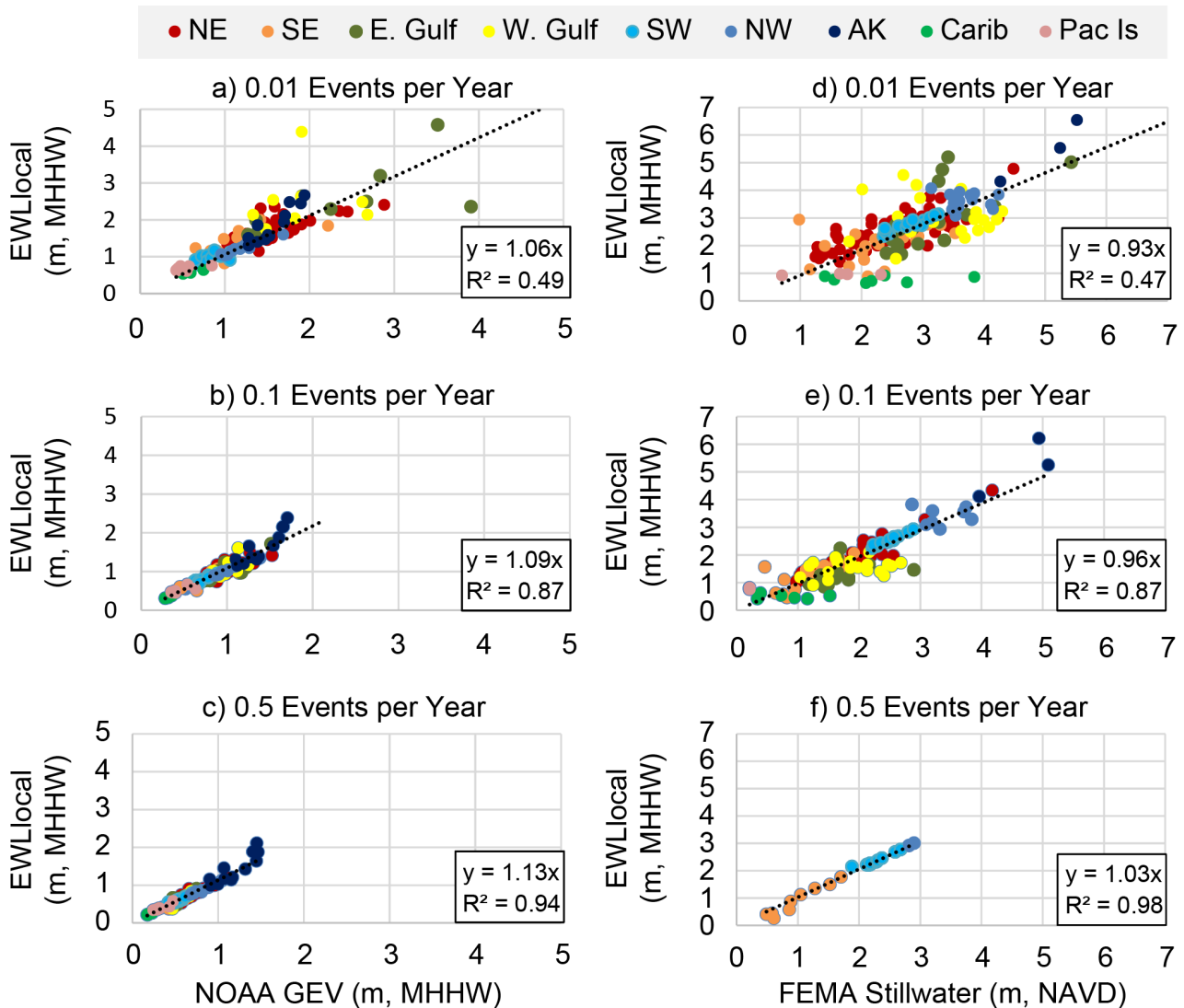
Figure 3.5: Comparison between (a–c) this study’s EWL local to those of NOAA (Zervas, 2013) based on a GEV fit of annual highest water levels and to (d–f) the stillwater (storm surge, tides, and wave set-up) components of FEMA used in their Flood Insurance Study at the 0.01-year, 0.1-year, and 0.5-year average event frequency levels.
