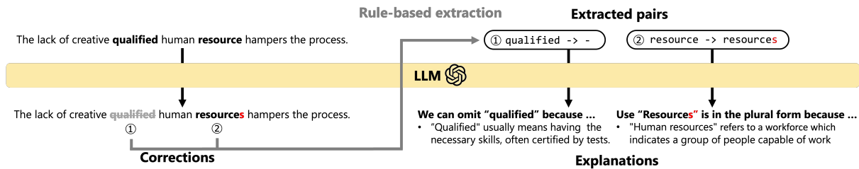
Figure 1: How to generate an explanation of the proposed method PI.
