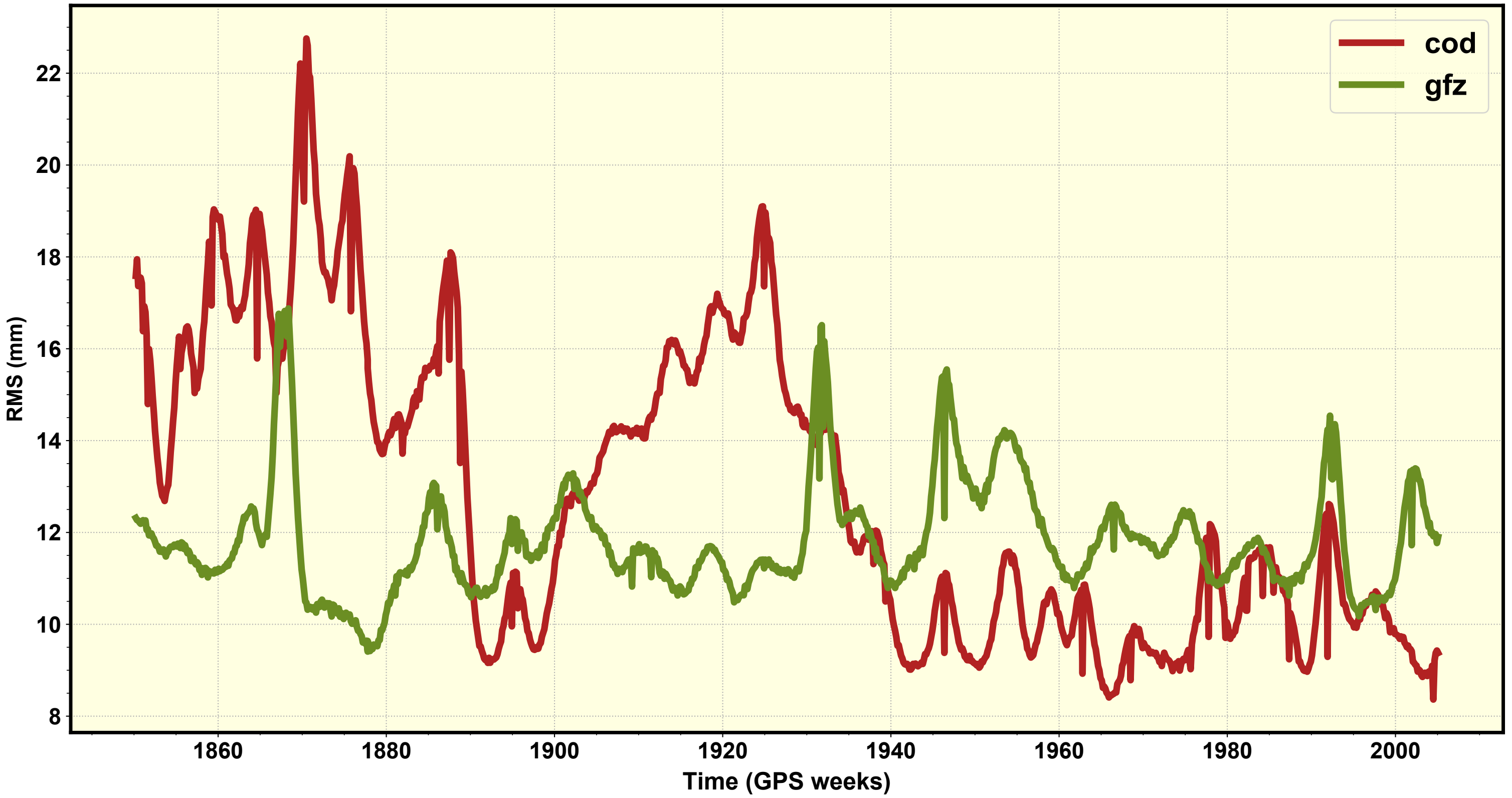
Orbits Rms (ACs MGEX w.r.t. ACs IGS regular) GPS constellation
