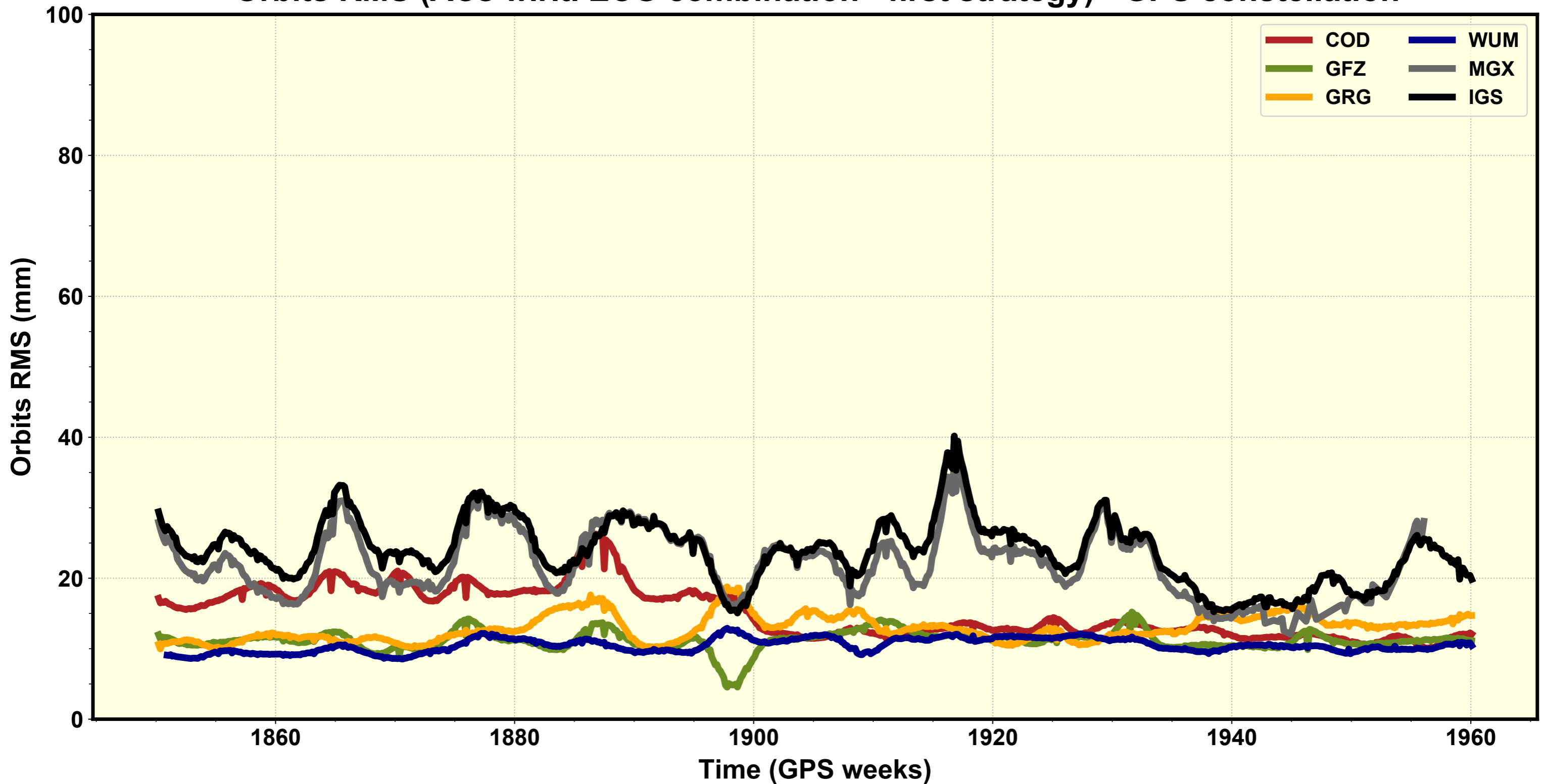
Orbits RMS (ACs w.r.t. ECG combination - first strategy) - GPS constellation
