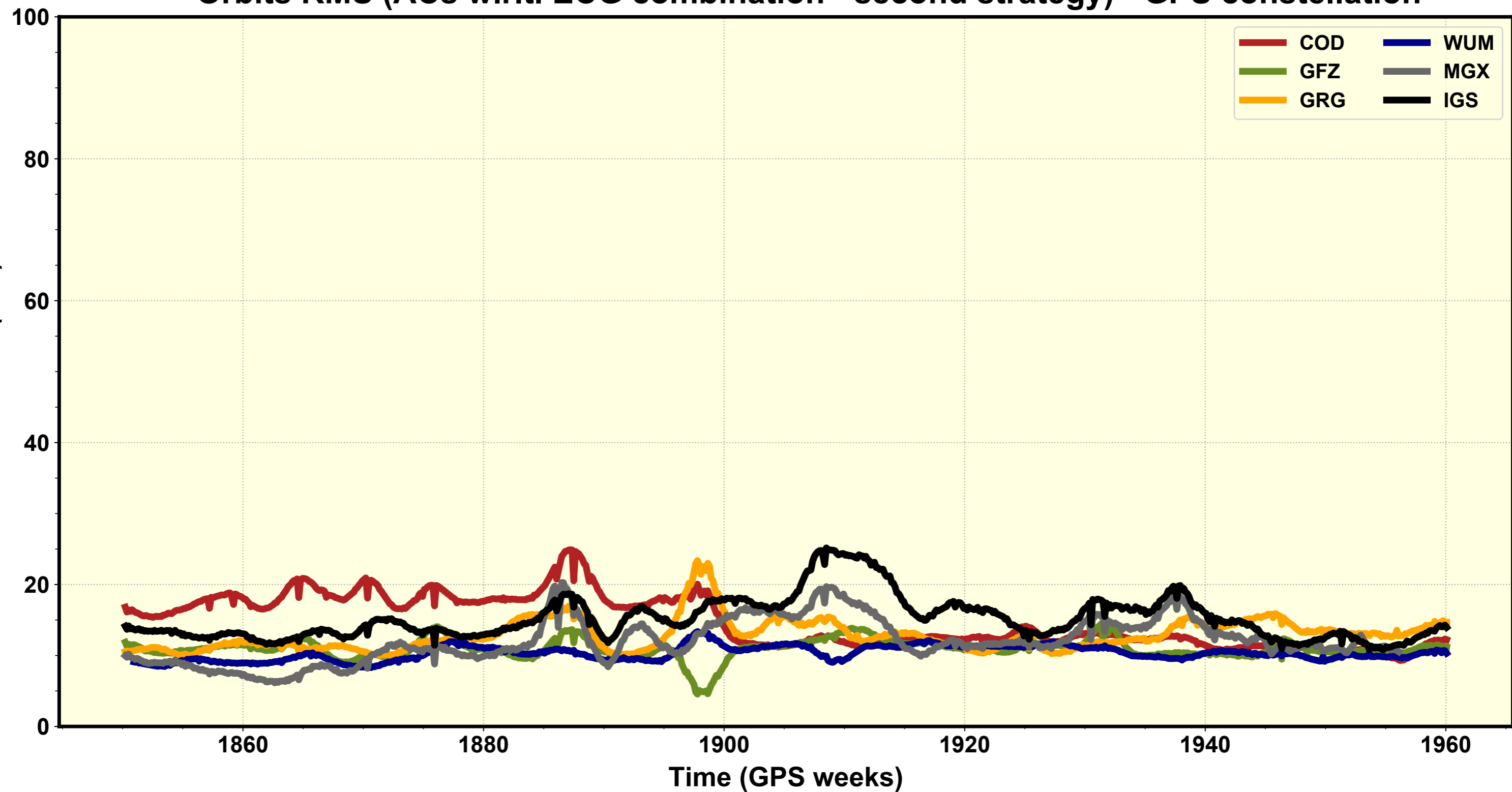
Orbits RMS (ACs w.r.t. ECG combination - second strategy) - GPS constellation
