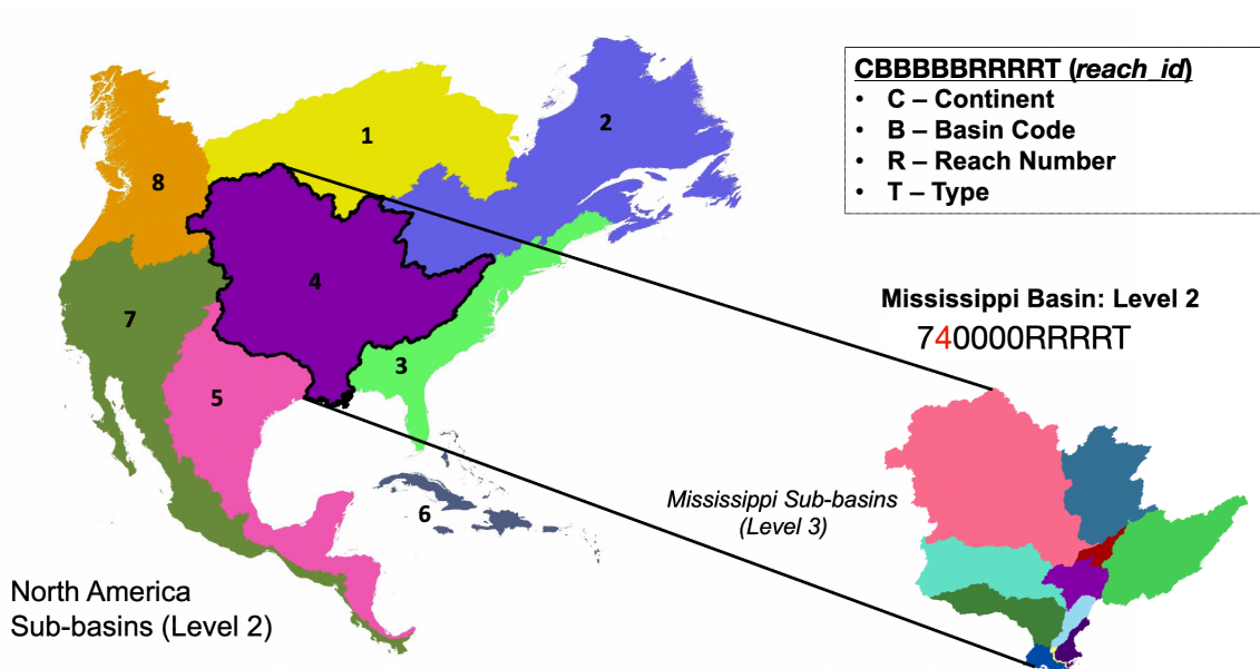
Figure 2. Example of the Pfafstetter basin coding system [7] at Level 2 over North America.
