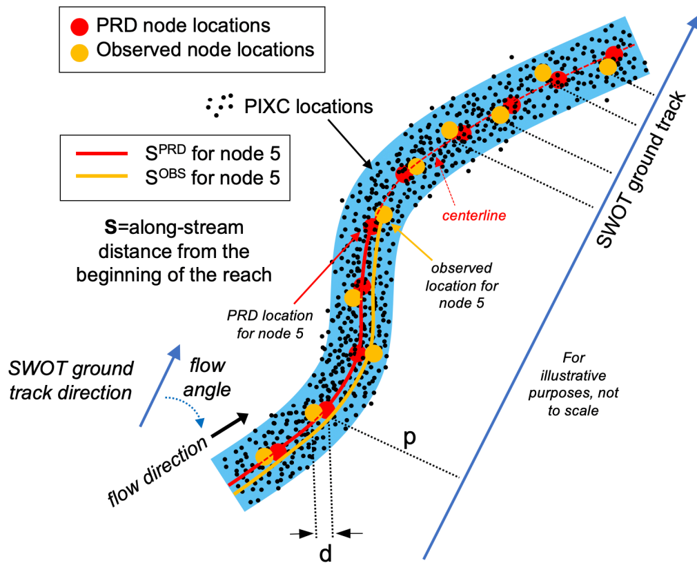
Figure 3. Illustration of quantites used to compute reported node distances for a partial segment of one reach. Definitions of quantities shown are provided in the body text that accompanies this figure.
