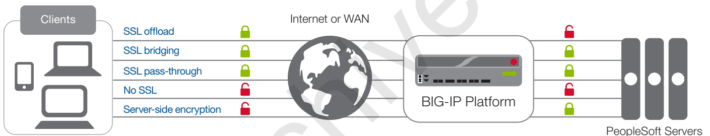
Figure 2: SSL options
