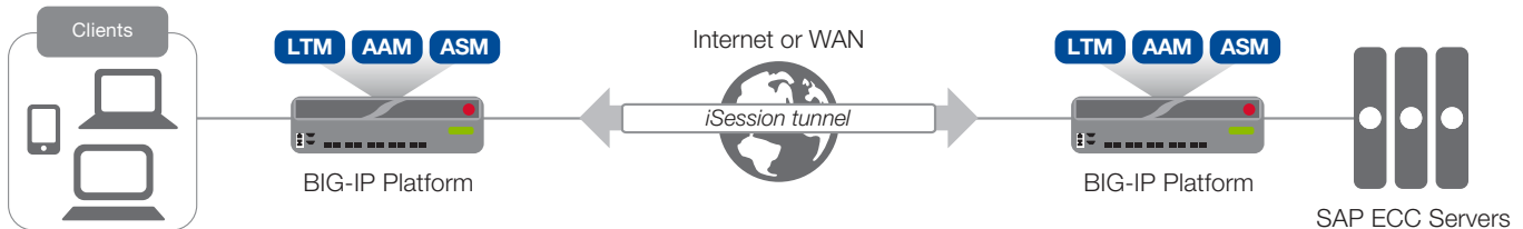
Figure 1: Using an iSession tunnel to secure and optimize traffic between two BIG-IP systems
