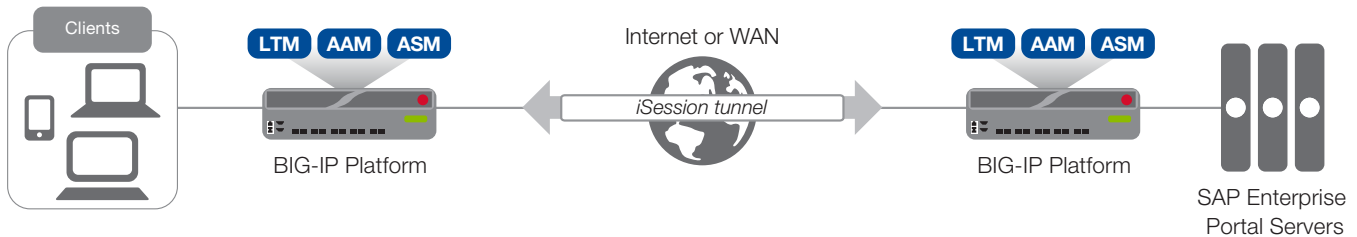
Figure 1: Using an iSession tunnel to secure and optimize traffic between two BIG-IP systems
