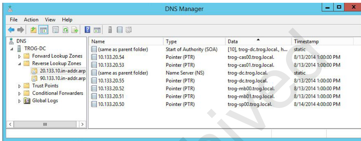
Figure 14: DNS Manager
