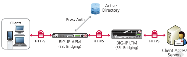
Figure 5: BIG-IP APM with SSL Offload configuration example
