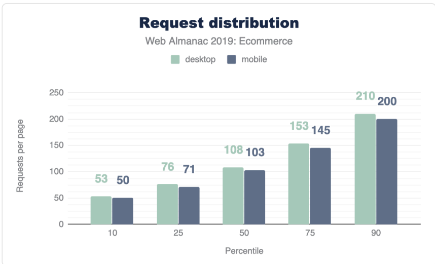
Figure 13.8. Distribution of requests per ecommerce page.
