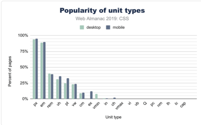
Figure 2.5. Popularity of unit types.
