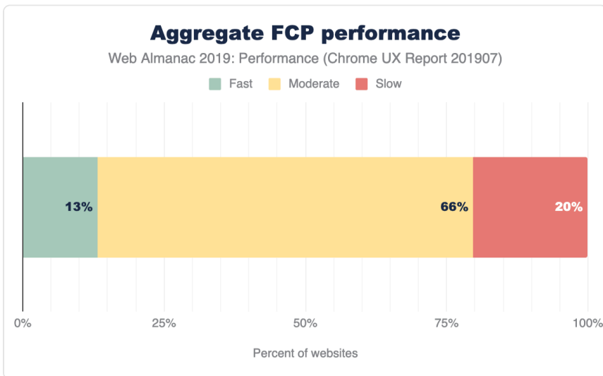
Figure 7.2. Distribution of websites labeled as having fast, moderate, or slow FCP.
