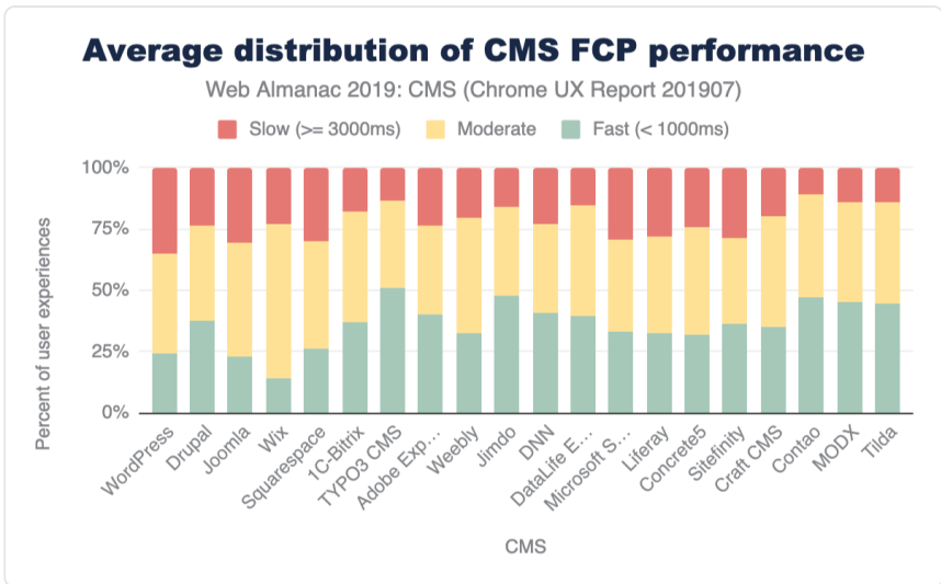
Figure 14.16. Average distribution of FCP experiences across CMSs.
