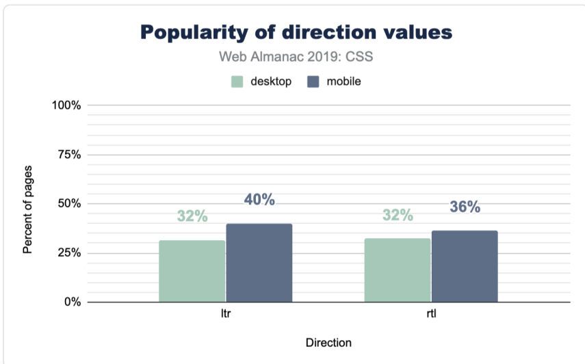
Figure 2.14. Popularity of direction values.
