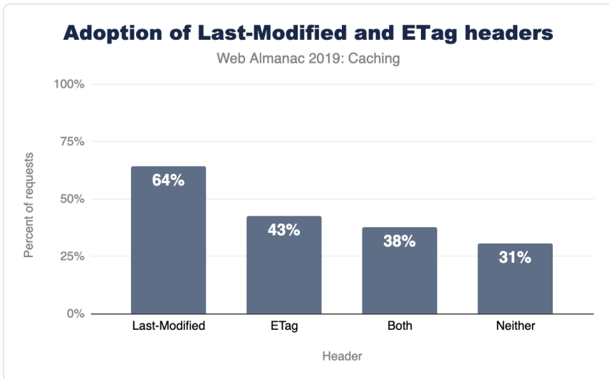
Figure 16.12. Adoption of validating freshness via Last-Modified and ETag headers for desktop websites.
