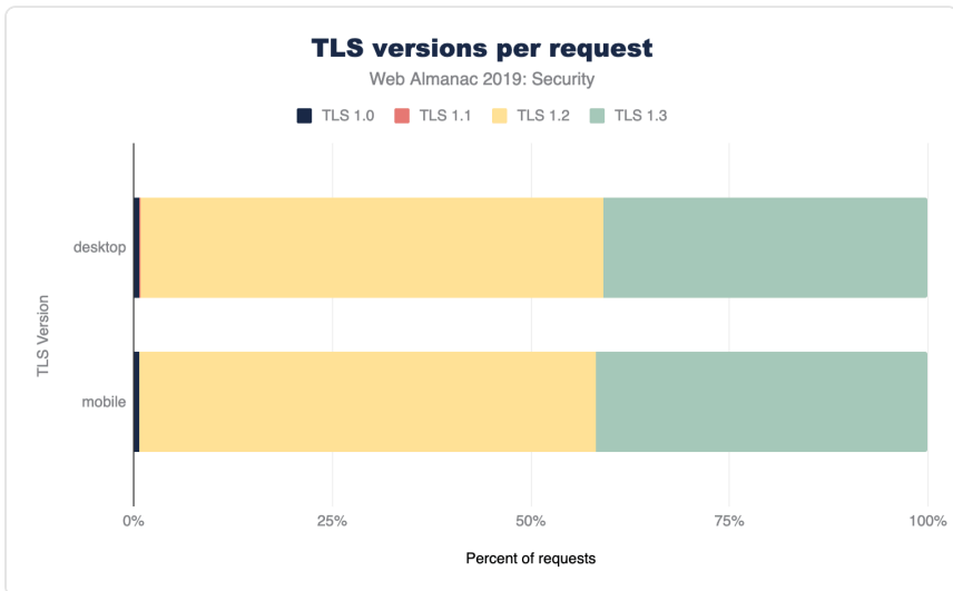
Figure 8.2. Usage of TLS protocol versions.
