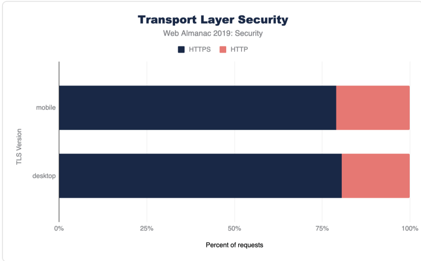
Figure 8.1. Usage of HTTP versus HTTPS.
