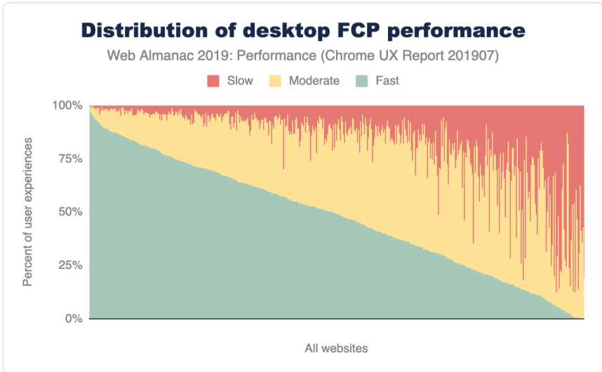
Figure 7.3. Distribution of desktop websites' fast, moderate, and slow FCP performance.
