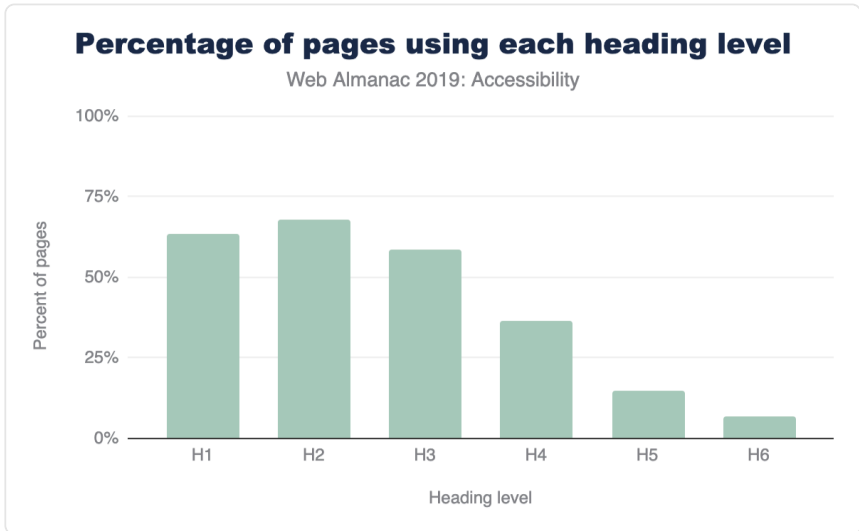
Figure 9.3. Popularity of heading levels.
