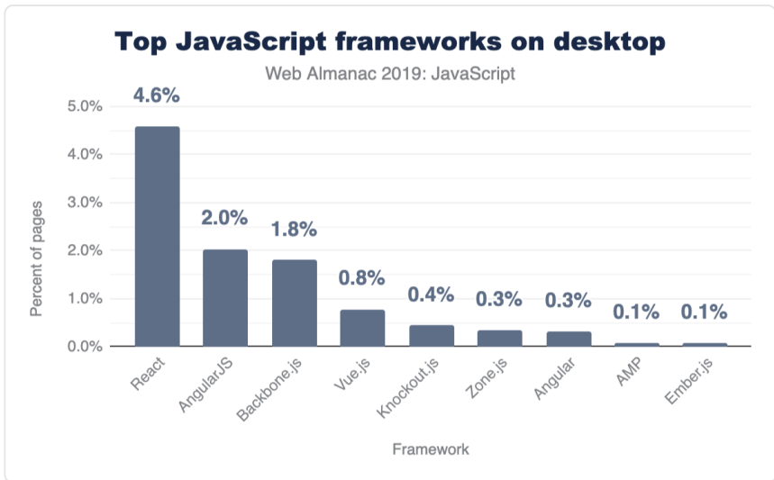
Figure 1.12. Most frequently used frameworks on desktop.
