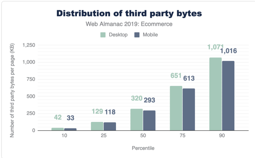
Figure 13.18. Distribution of third-party bytes per ecommerce page.
