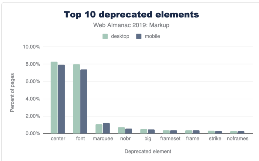
Figure 3.6. Most frequently used deprecated elements.
