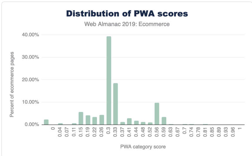
Figure 13.22. Distribution of Lighthouse PWA category scores for mobile ecommerce pages.
