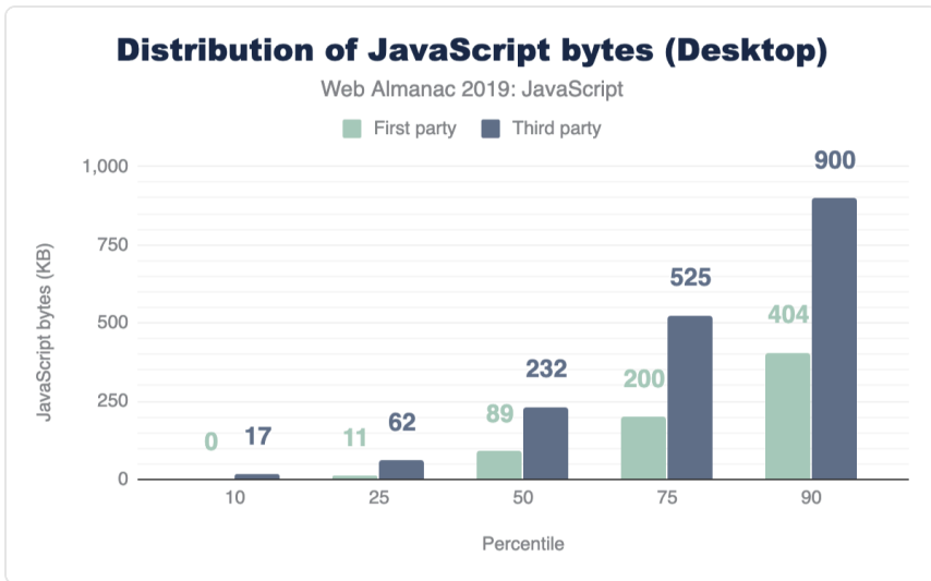
Figure 1.8. Distribution of total JavaScript downloaded on desktop.
