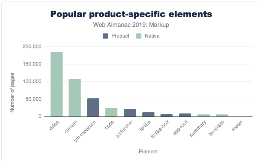
Figure 3.9. Popularity of product-specific and native elements under 5% adoption.
