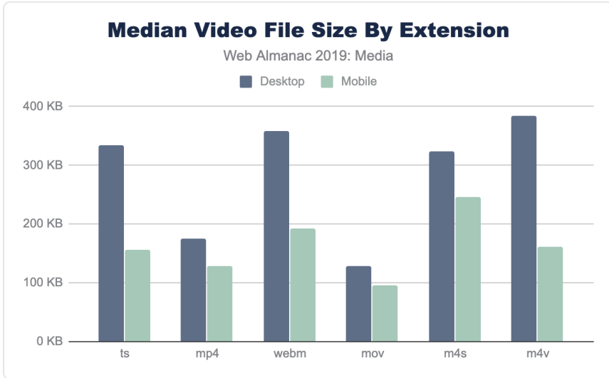
Figure 4.21. Median file size by video extension.
