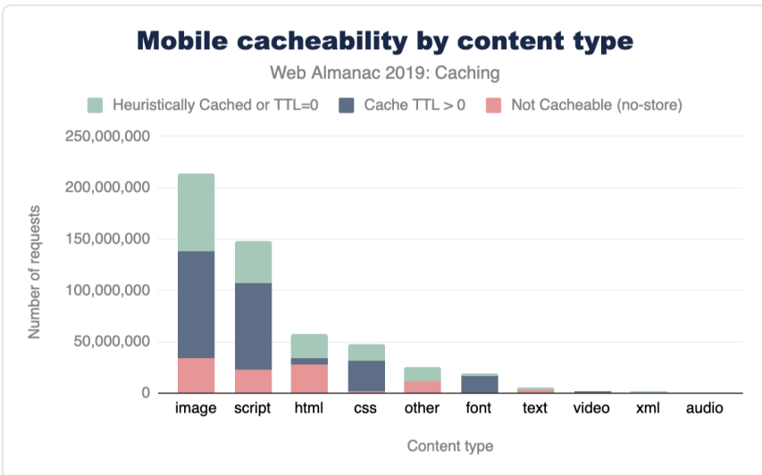
Figure 16.6. Distribution of cacheability by content type for mobile.
