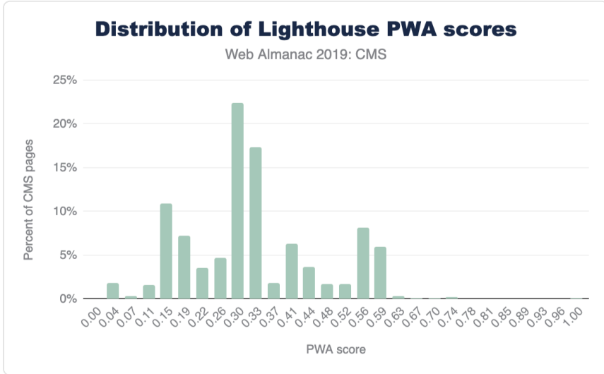
Figure 14.20. Distribution of Lighthouse PWA category scores for CMS pages.
