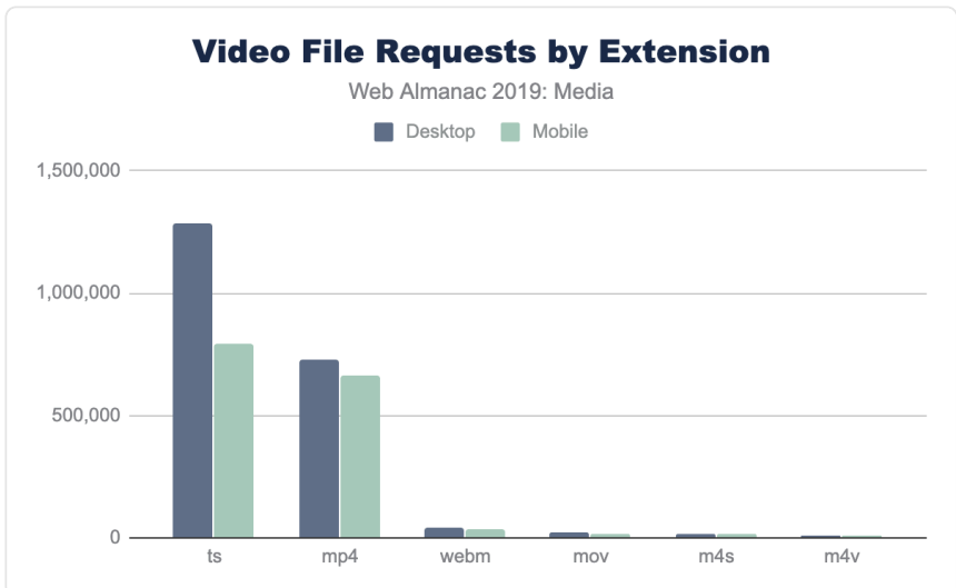
Figure 4.20. Count of video files by extension.
