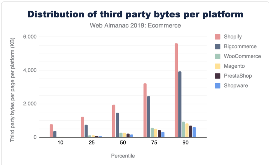
Figure 13.20. Distribution of third-party bytes (KB) per mobile page for each ecommerce platform.
