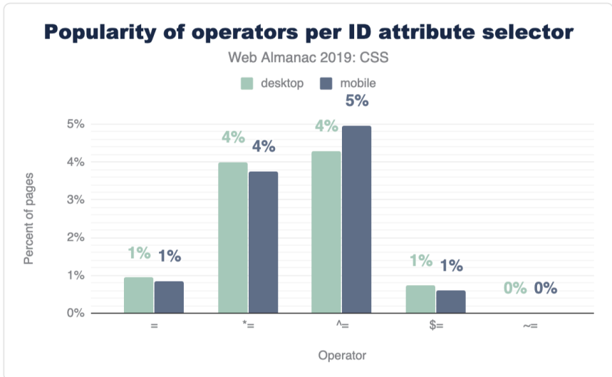
Figure 2.9. Popularity of operators per ID attribute selector.
