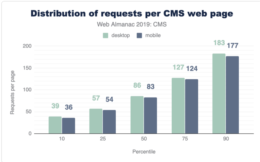
Figure 14.7. Distribution of CMS requests per page.
