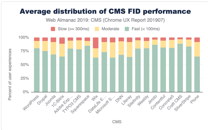
Figure 14.18. Average distribution of FID experiences across CMSs.
