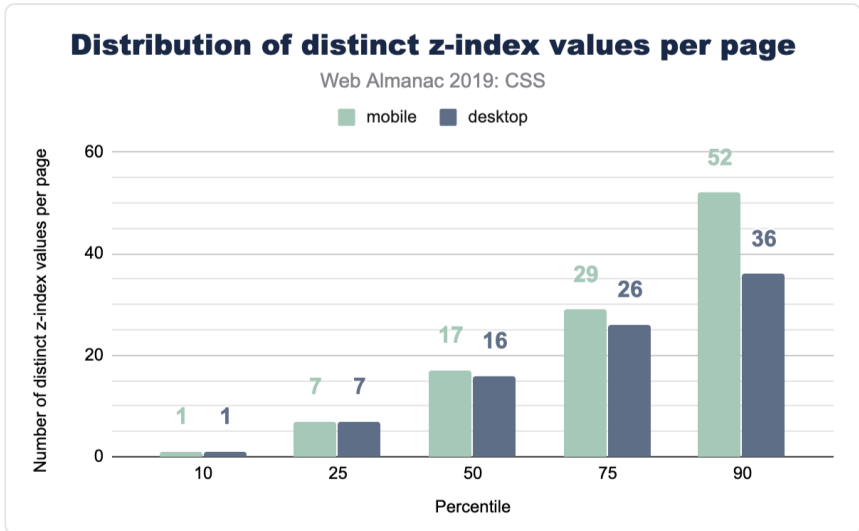
Figure 2.20. Distribution of the number of distinct z-index values per page.
