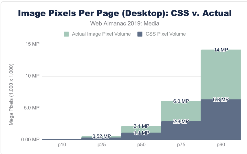
Figure 4.4. Image pixels per page (desktop): CSS versus actual.
