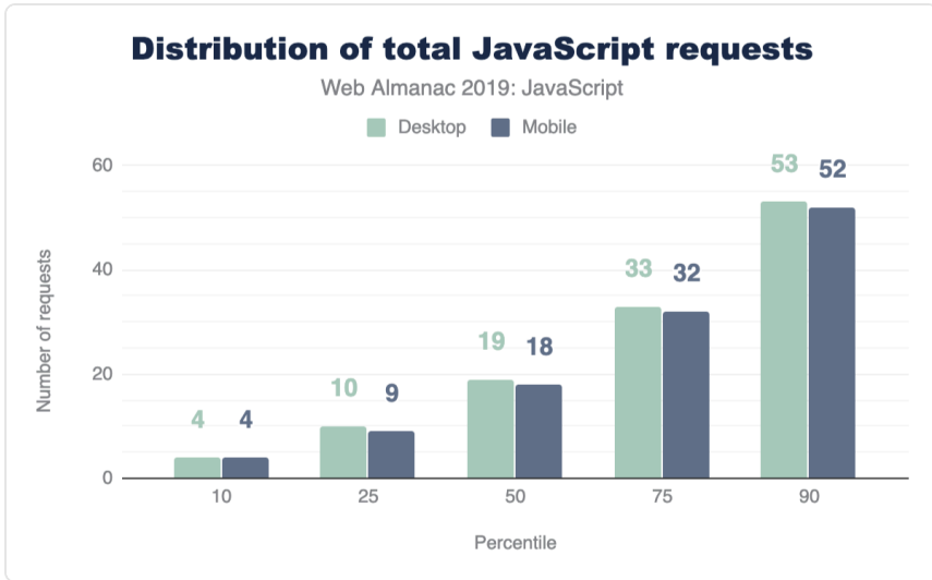
Figure 1.5. Distribution of total JavaScript requests.
