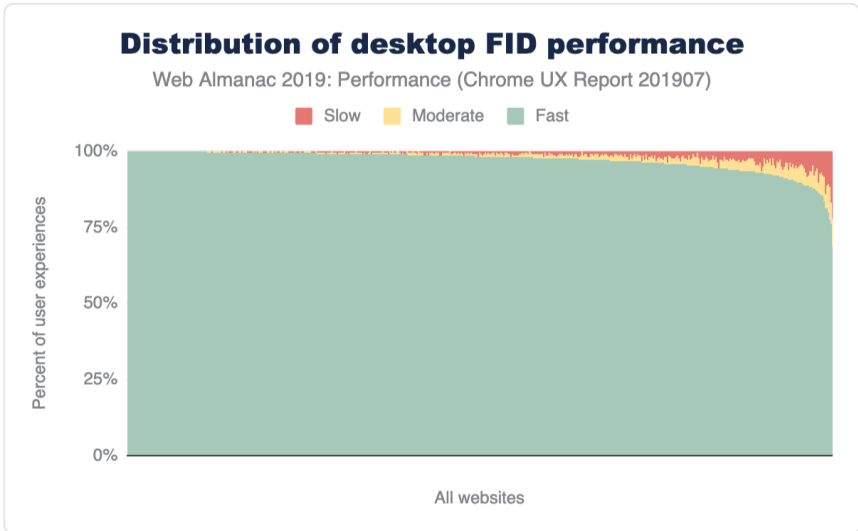
Figure 7.14. Distribution of desktop websites' fast, moderate, and slow FID performance.
