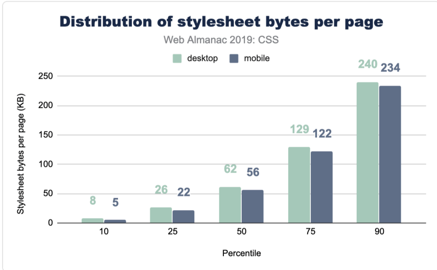
Figure 2.35. Distribution of the number of stylesheet bytes (KB) loaded per page.
