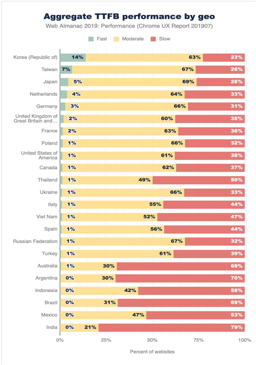
Figure 7.11. Distribution of websites labeled as having fast, moderate, or slow TTFB, broken down by geo.
