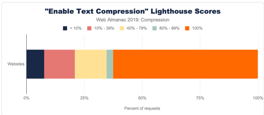
Figure 15.11. Lighthouse "enable text compression" audit scores.
