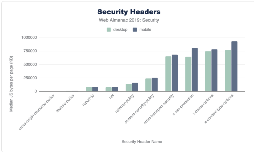
Figure 8.8. Usage of Security Headers
