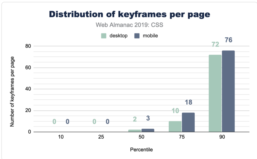
Figure 2.26. Distribution of the number of keyframes per page.
