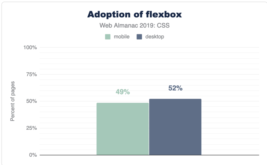
Figure 2.12. Adoption of flexbox.
