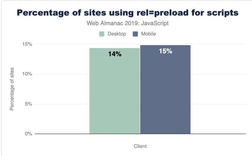
Figure 1.15. Percentage of sites using rel=preload for scripts.
