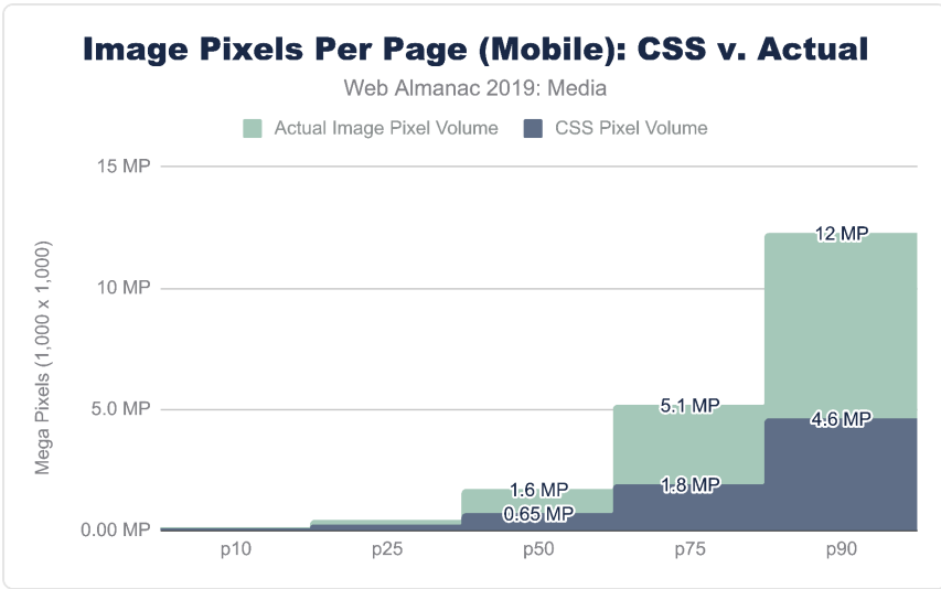
Figure 4.3. Image pixels per page (mobile): CSS versus actual.
