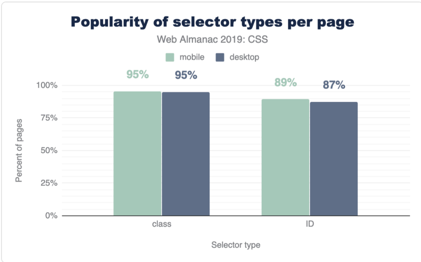
Figure 2.7. Popularity of selector types per page.
