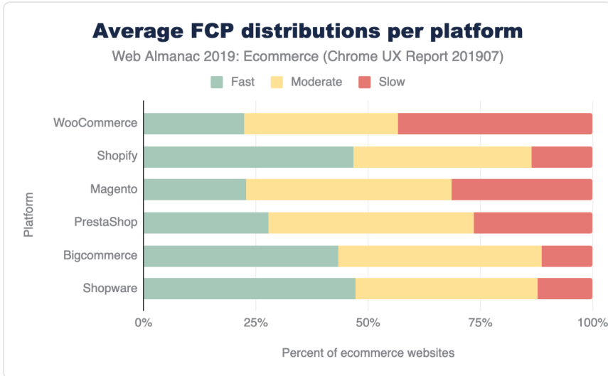
Figure 13.21. Average distribution of FCP experiences per ecommerce platform.
