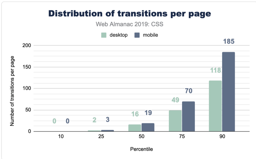
Figure 2.25. Distribution of the number of transitions per page.
