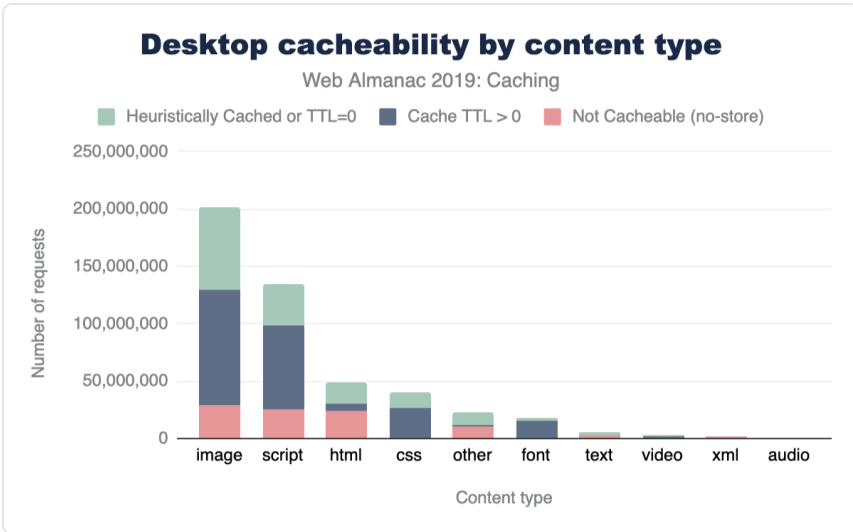
Figure 16.5. Distribution of cacheability by content type for desktop.
