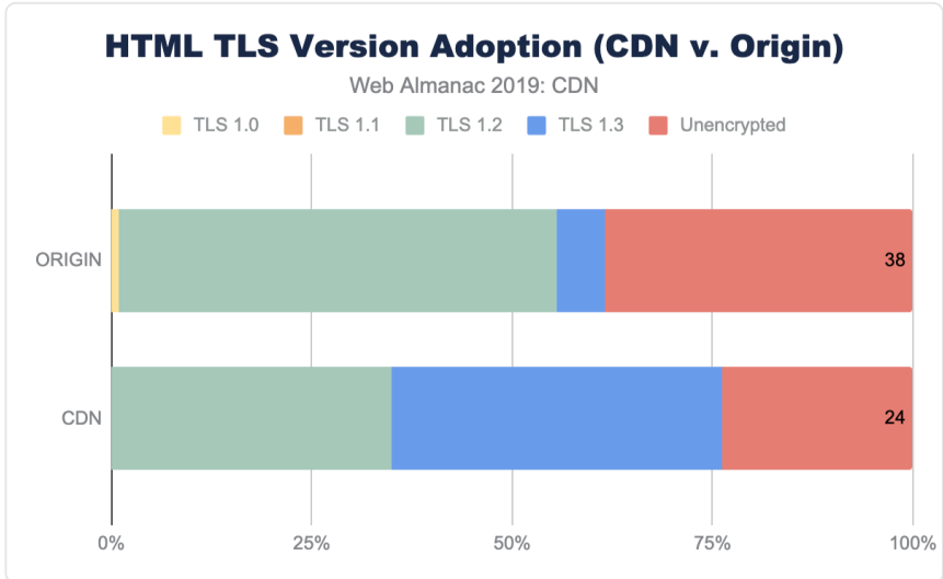
Figure 17.15. HTML TLS version adoption (CDN vs. origin).
