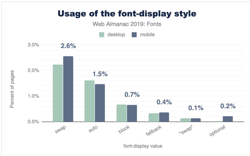
Figure 6.11. Usage of font-display values.
