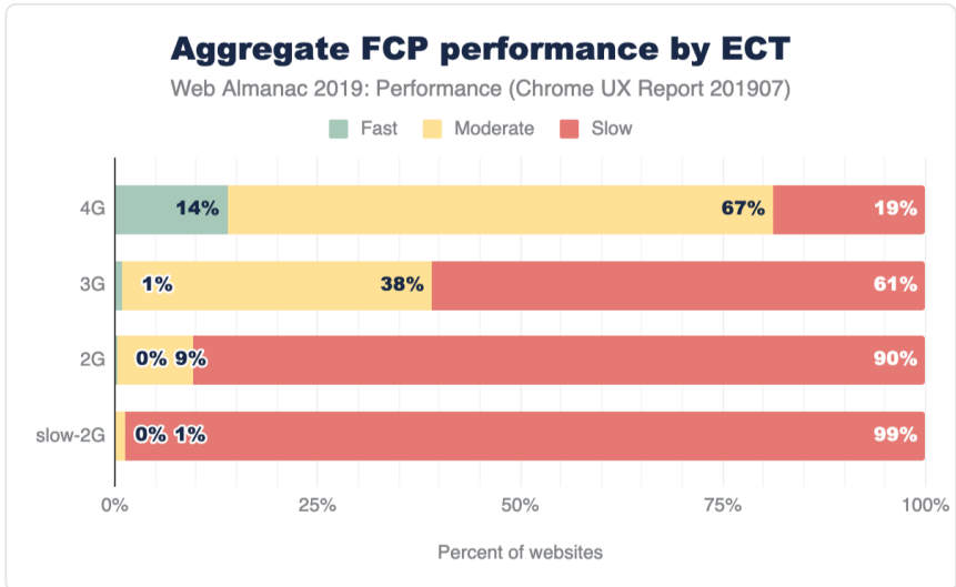
Figure 7.6. Distribution of websites labeled as having fast, moderate, or slow FCP, broken down by ECT .
