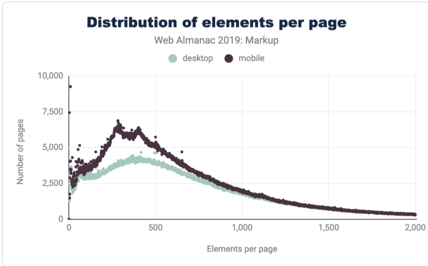
Figure 3.3. Element frequencies as of 2019.
