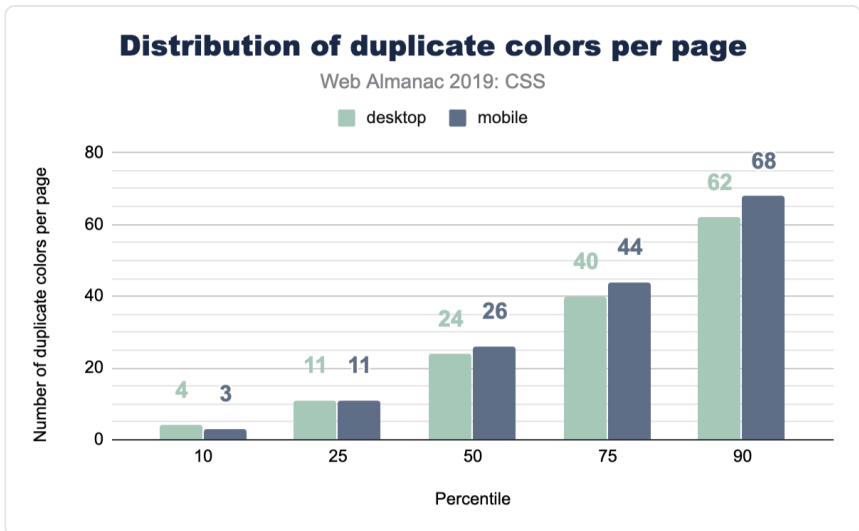
Figure 2.4. Distribution of duplicate colors per page.
