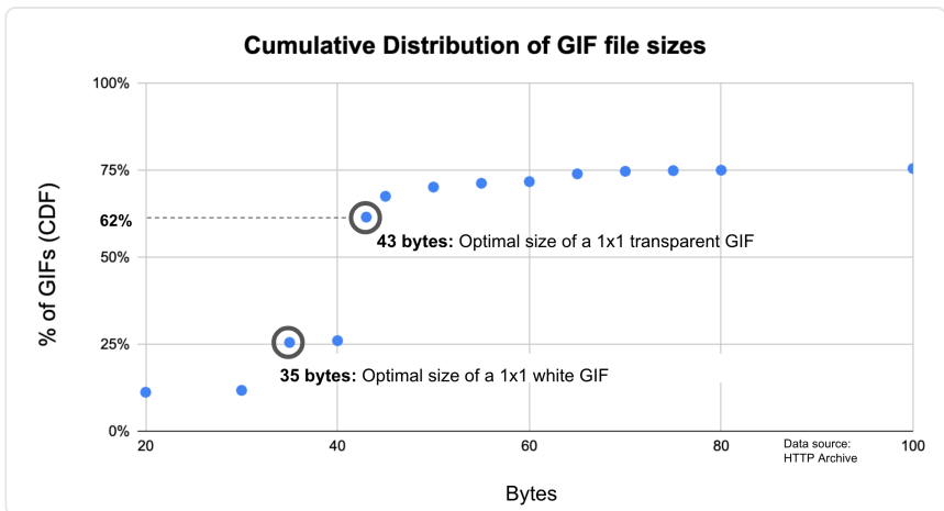
Figure 18.10. Cumulative distribution function of GIF file sizes.
