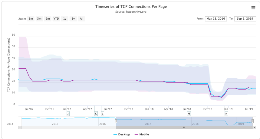
Figure 20.9. TCP connections per page. (Source: HTTP Archive 431 )
