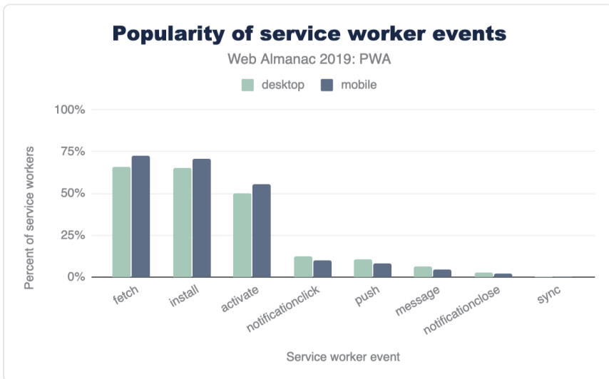
Figure 11.4. Popularity of service worker events.
