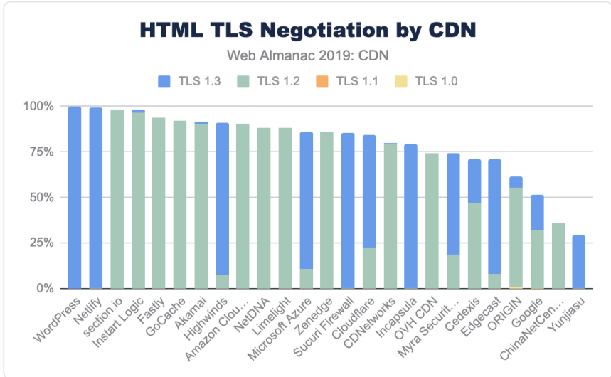
Figure 17.18. HTML TLS version by CDN.
