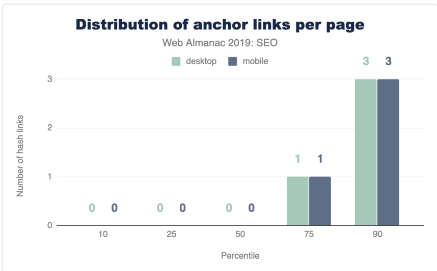
Figure 10.9. Distribution of anchor links per page.
