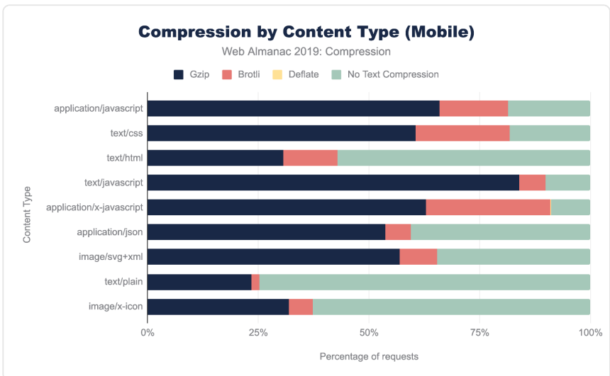
Figure 15.8. Compression by content type as a percent for mobile.
