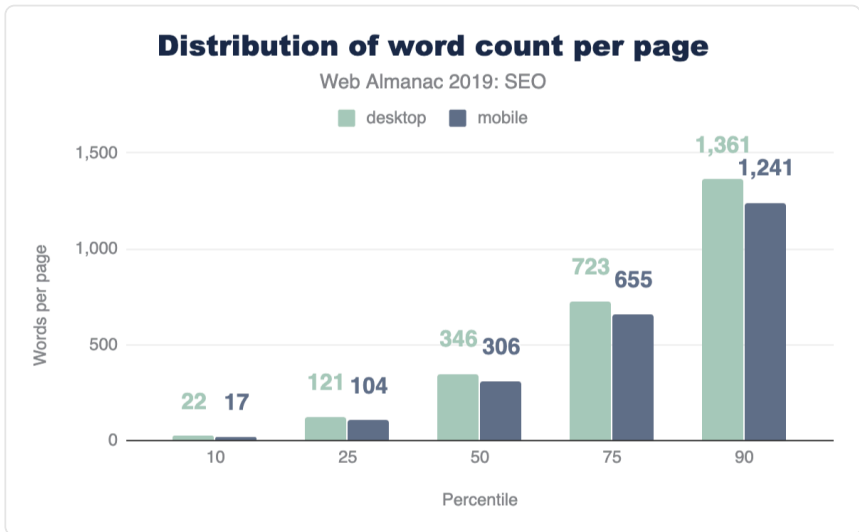
Figure 10.1. Distribution of the number of words per page.
