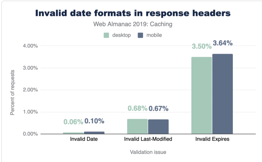
Figure 16.13. Invalid date formats in response headers.
