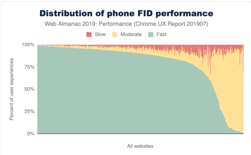
Figure 7.15. Distribution of phone websites' fast, moderate, and slow FID performance.
