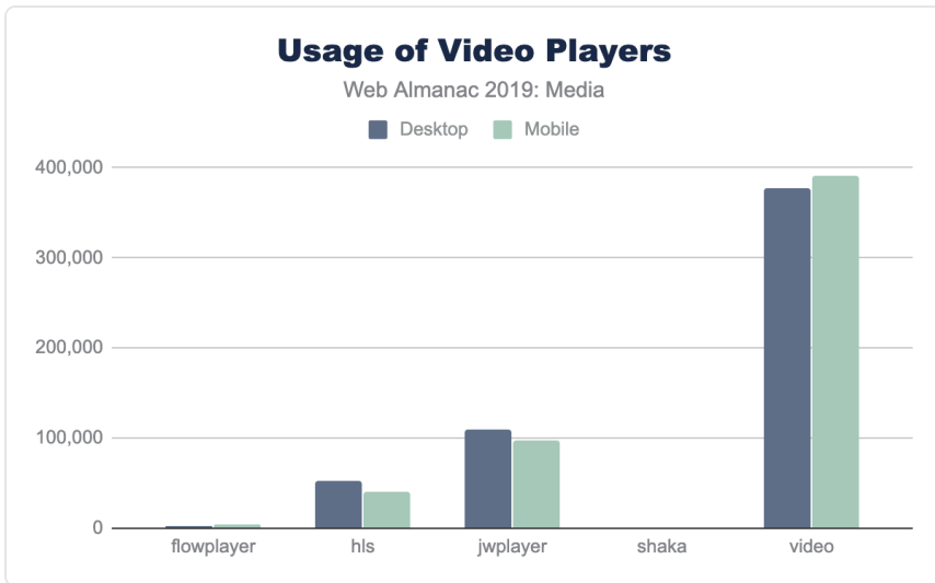
Figure 4.23. Top JavaScript video players.
