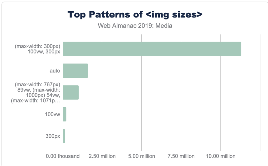
Figure 4.16. Top patterns of <img sizes> .
