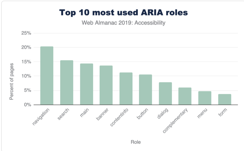
Figure 9.9. Top 10 ARIA roles.
