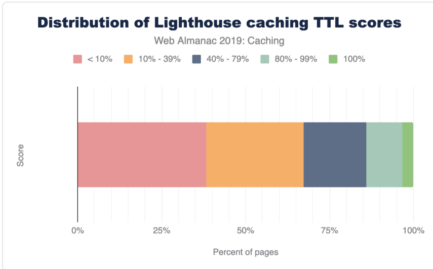
Figure 16.21. Distribution of Lighthouse scores for the “Uses Long Cache TTL” audit for mobile web pages.
