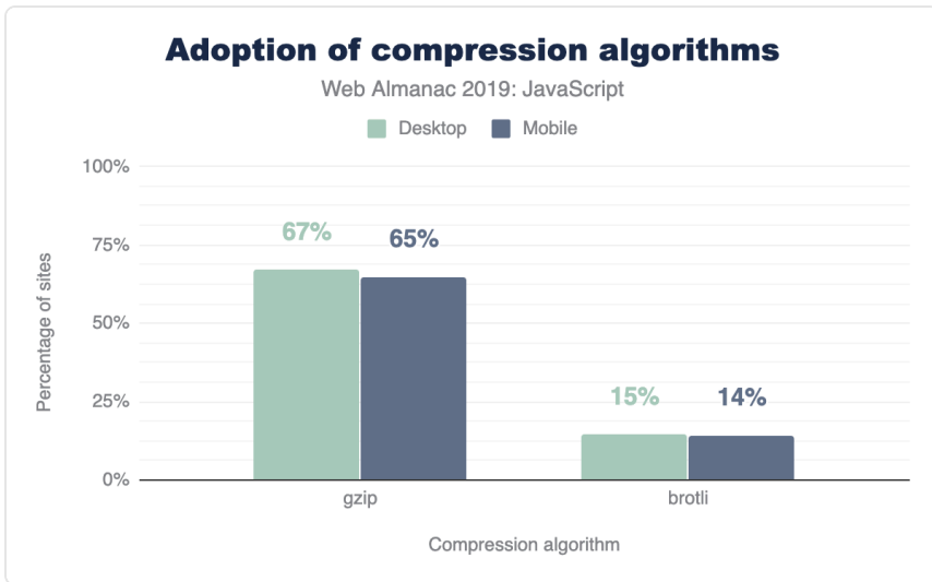
Figure 1.10. Percentage of sites compressing JavaScript resources with Gzip or Brotli.
