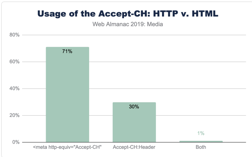
Figure 4.17. Usage of the Accept-CH header versus the equivalent <meta> tag.
