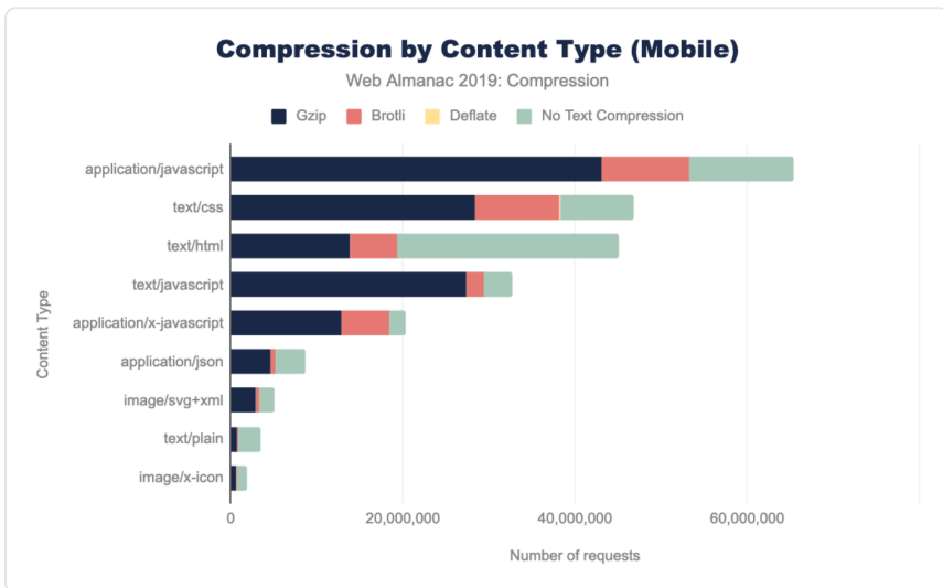
Figure 15.6. Compression by content type for mobile.
