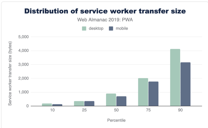
Figure 11.5. Distribution of service worker transfer size.
