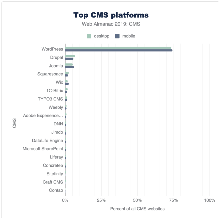
Figure 14.5. Top CMS platforms as a percent of all CMS websites.
