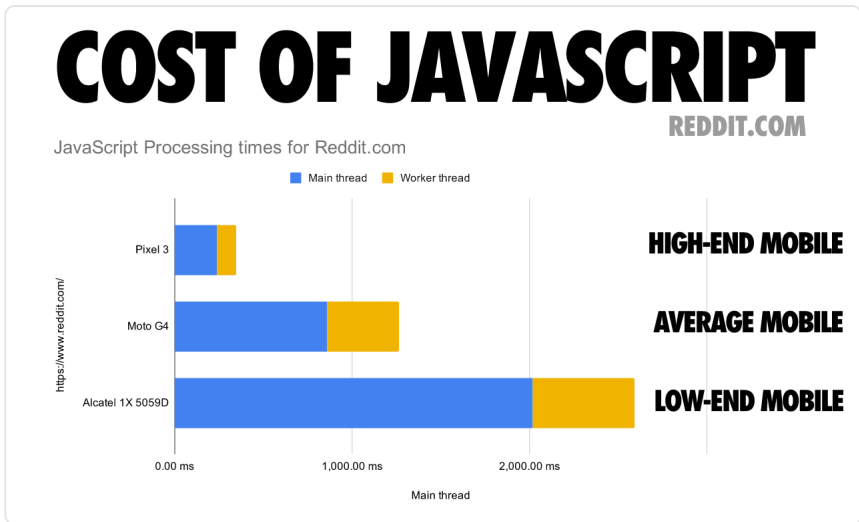
Figure 1.4. JavaScript processing times for reddit.com. From The cost of JavaScript in 2019 5 .
