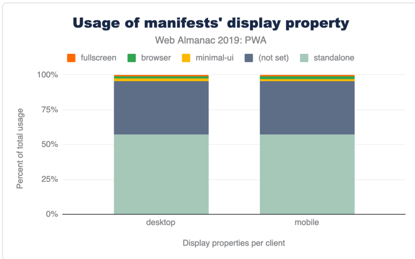
Figure 11.7. Usage of web app manifest display properties.
