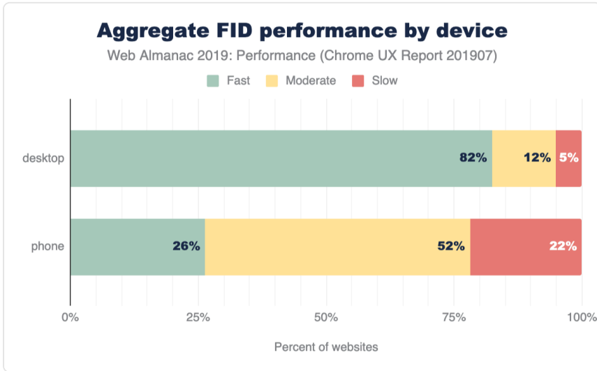
Figure 7.16. Distribution of websites labeled as having fast, moderate, or slow FID, broken down by device type.
