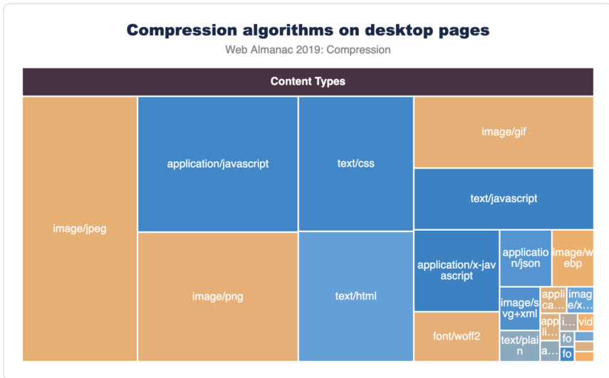
Figure 15.3. Top 25 compressed content types.
