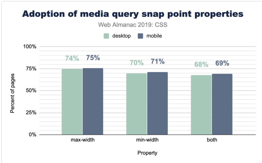
Figure 2.31. Adoption of properties used in media query snap points.
