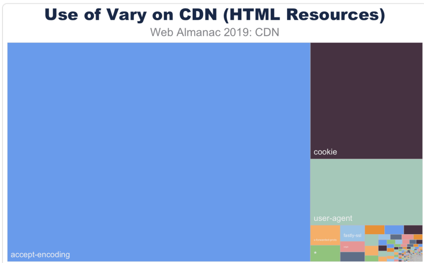
Figure 17.24. Usage of Vary for HTML served from CDNs.
