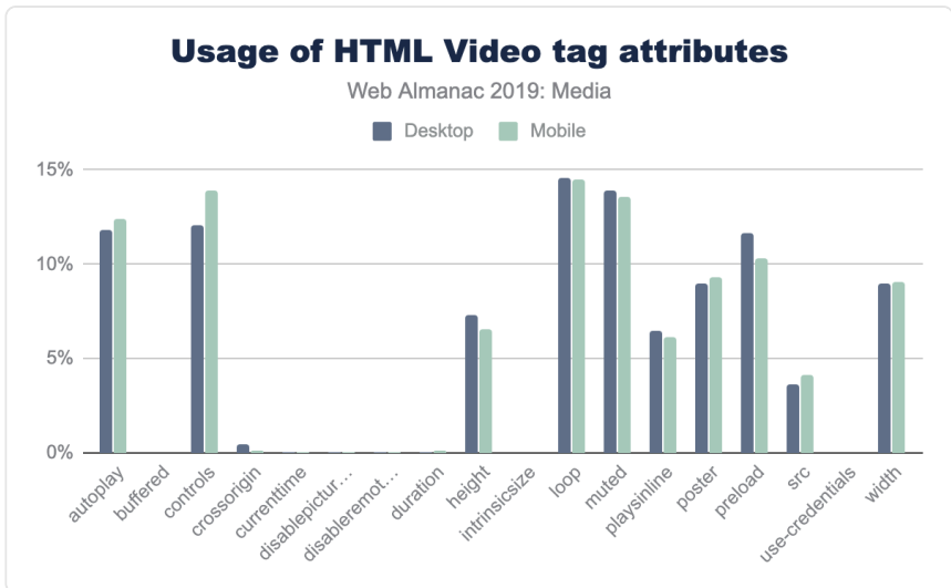
Figure 4.22. Usage of HTML video tag attributes.
