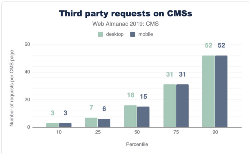
Figure 14.11. Distribution of the number of third-party requests on CMS pages.
