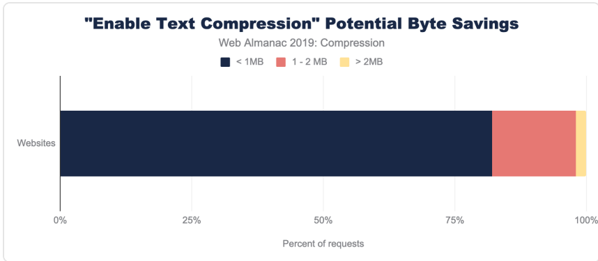
Figure 15.12. Lighthouse “enable text compression” audit potential byte savings.
