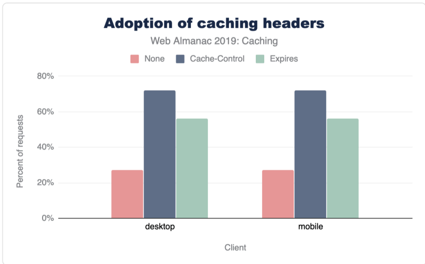
Figure 16.2. Presence of HTTP Cache-Control and Expires headers.
