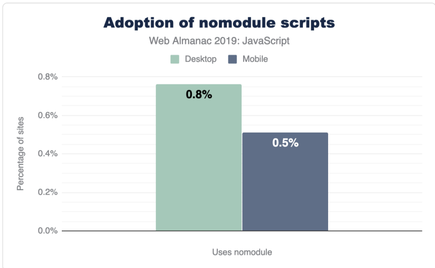
Figure 1.14. Percentage of sites using nomodule .
