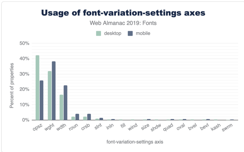
Figure 6.19. Usage of font-variation-settings axes.
