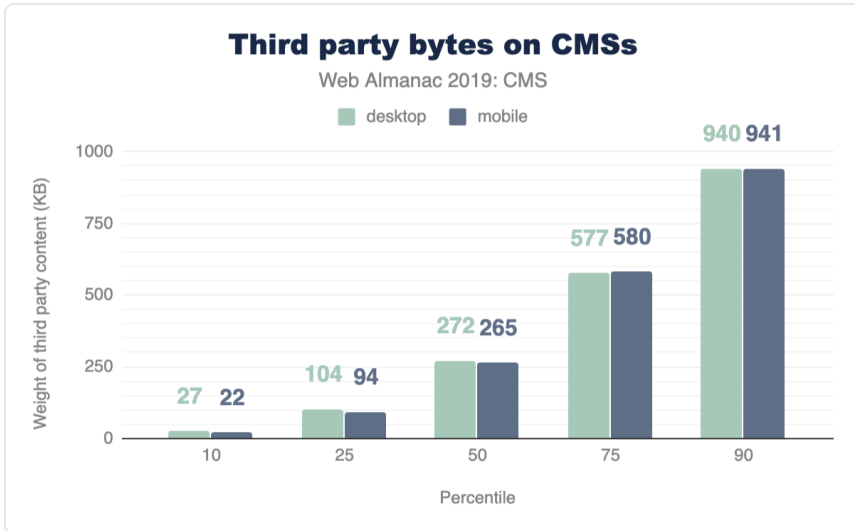
Figure 14.10. Distribution of third-party weight (KB) on CMS pages.
