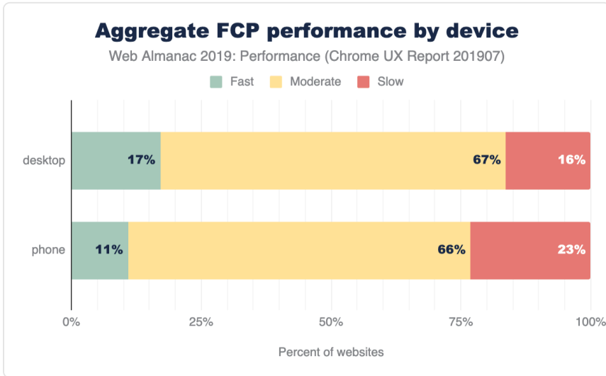
Figure 7.5. Distribution of websites labeled as having fast, moderate, or slow FCP, broken down by device type.
