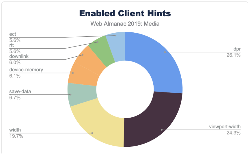
Figure 4.18. Enabled Client Hints.
