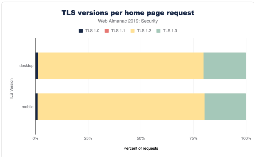
Figure 8.3. Usage of TLS protocol versions for home page requests only.
