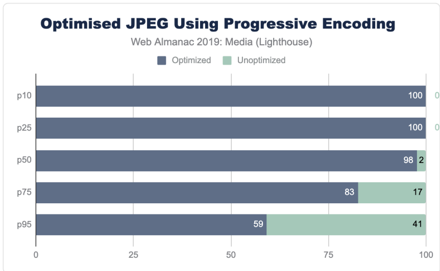
Figure 4.12. Percent “optimized” images.
