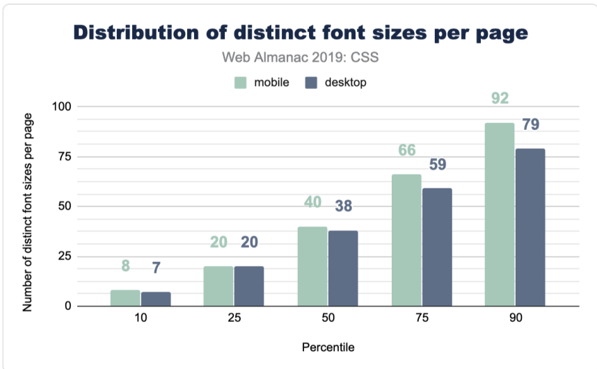
Figure 2.17. Distribution of the number of distinct font sizes per page.
