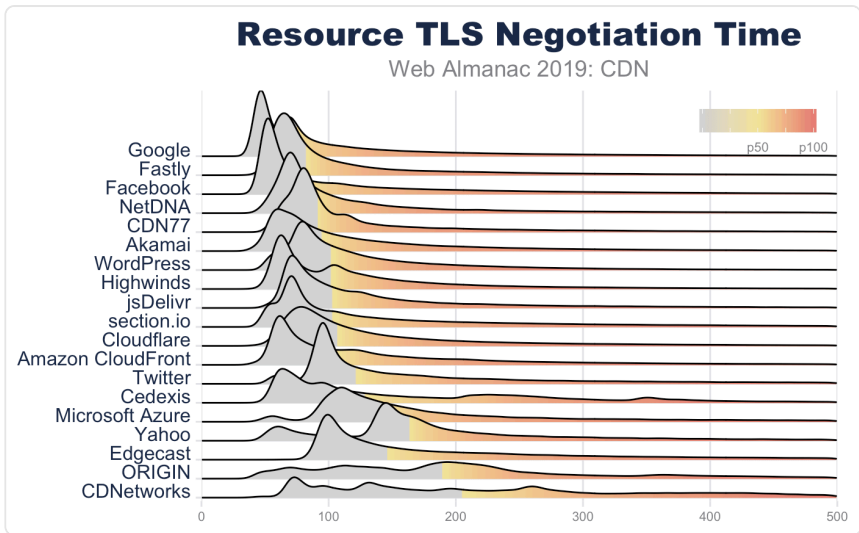
Figure 17.10. Resource TLS negotiation time.
