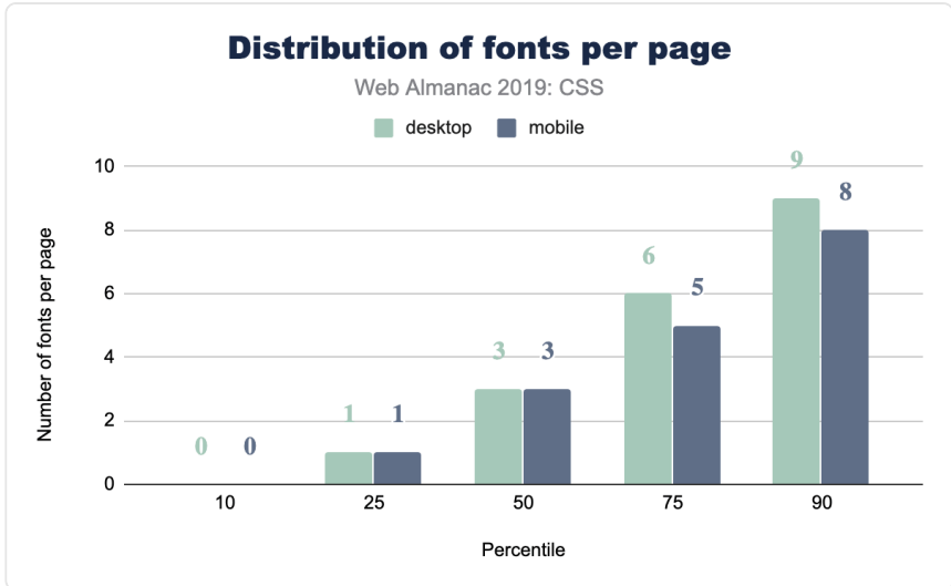
Figure 2.15. Distribution of the number of web fonts loaded per page.
