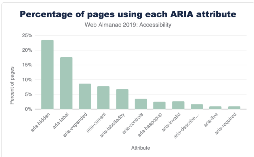
Figure 9.8. Percent of total pages vs ARIA attribute.
