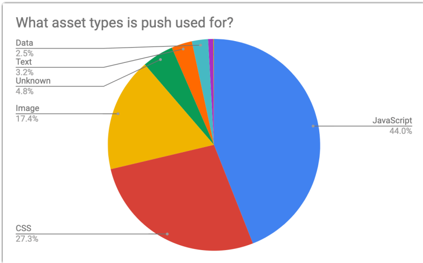
Figure 20.13. What asset types is push used for?
