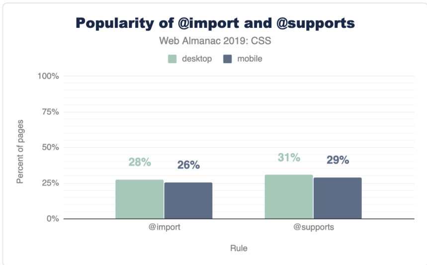
Figure 2.38. Popularity of CSS “at” rules.
