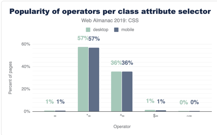
Figure 2.10. Popularity of operators per class attribute selector.
