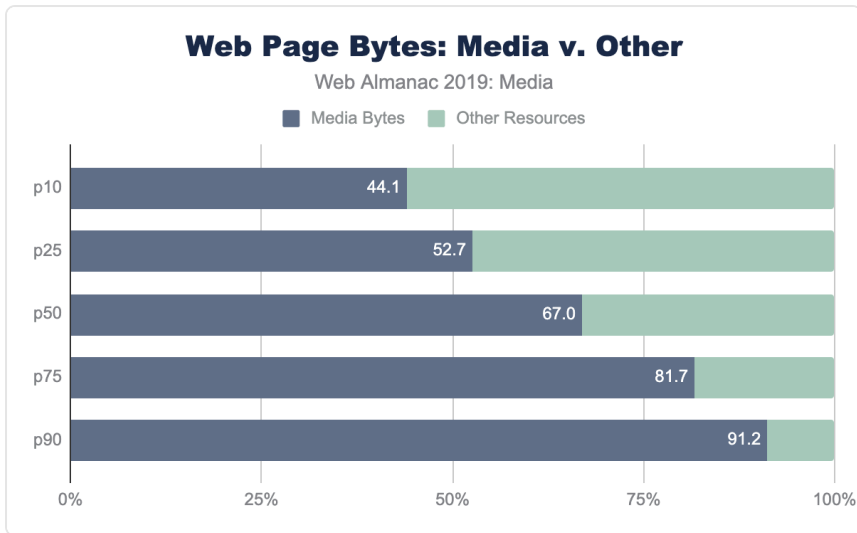
Figure 4.1. Web page bytes: image and video versus other.
