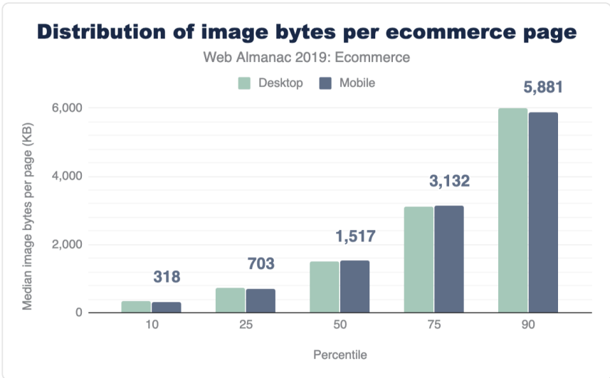
Figure 13.12. Distribution of image bytes (in KB) per ecommerce page.
