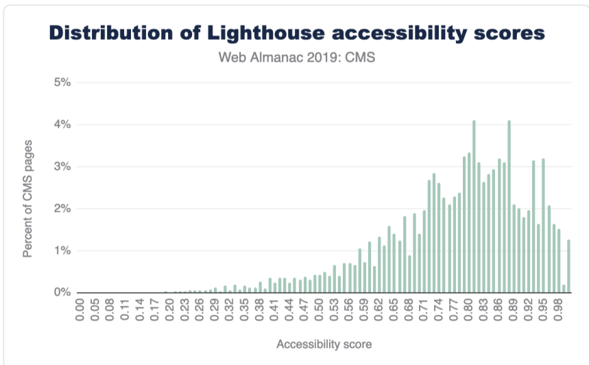
Figure 14.22. Distribution of Lighthouse accessibility category scores for CMS pages.
