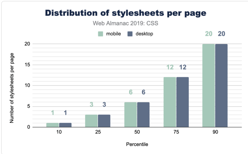
Figure 2.33. Distribution of the number of stylesheets loaded per page.
