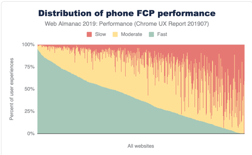
Figure 7.4. Distribution of phone websites' fast, moderate, and slow FCP performance.
