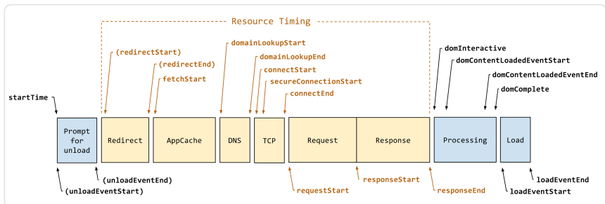
Figure 7.8. Navigation Timing API diagram of the events in a page navigation.
