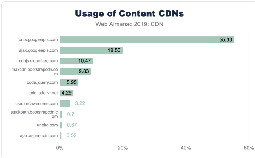
Figure 17.27. Usage of public content CDNs.
