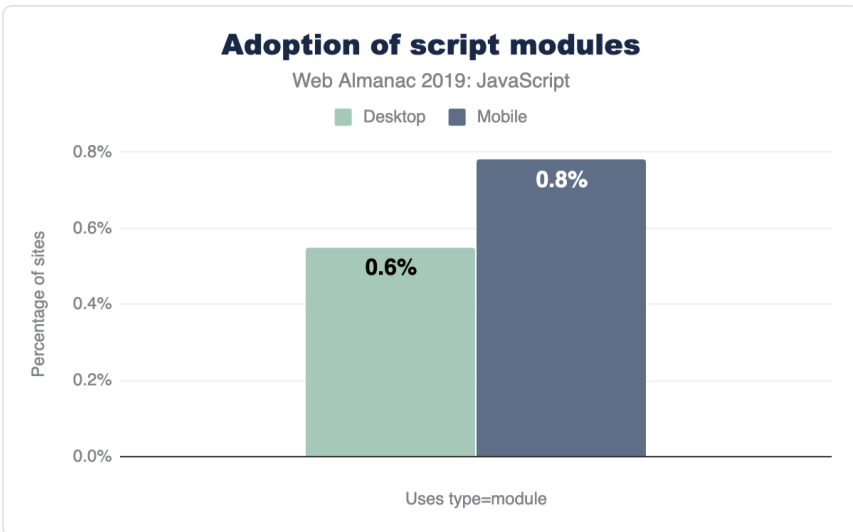
Figure 1.13. Percentage of sites utilizing type=module .
