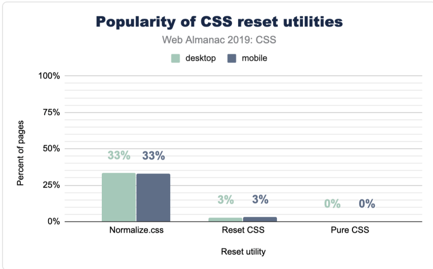
Figure 2.37. Adoption of CSS reset utilities.
