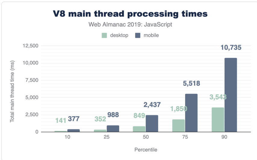
Figure 1.3. V8 Main thread processing times by device.
