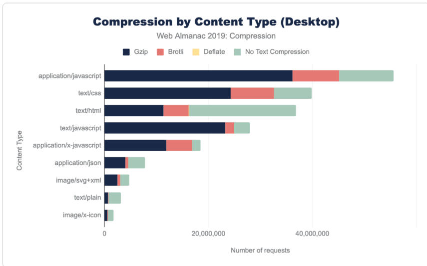
Figure 15.5. Compression by content type for desktop.
