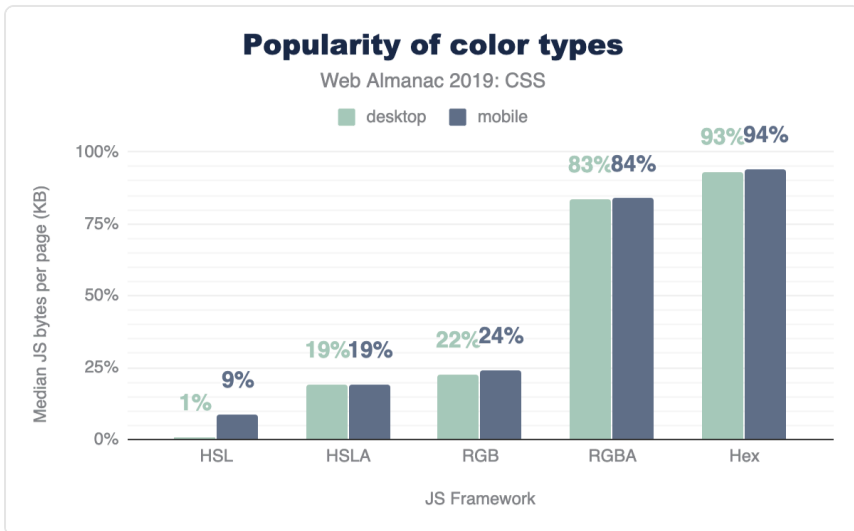
Figure 2.1. Popularity of color formats.
