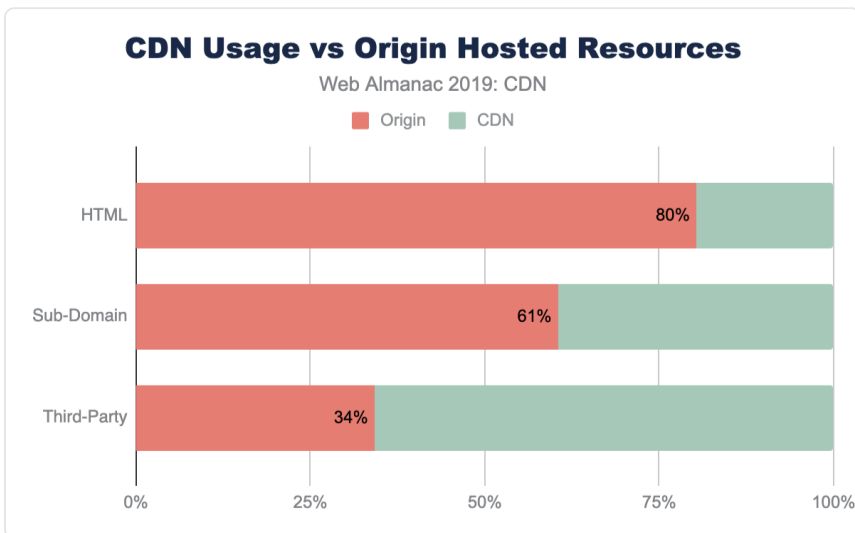
Figure 17.1. CDN usage vs. origin-hosted resources.
