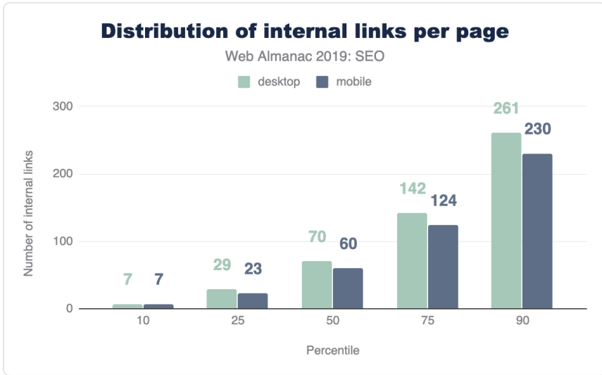
Figure 10.7. Distribution of internal links per page.
