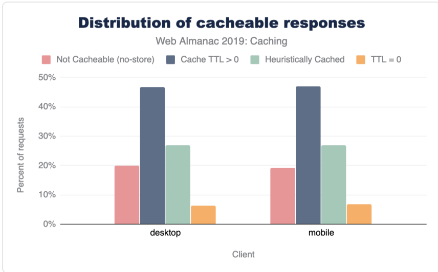
Figure 16.3. Distribution of cacheable responses.
