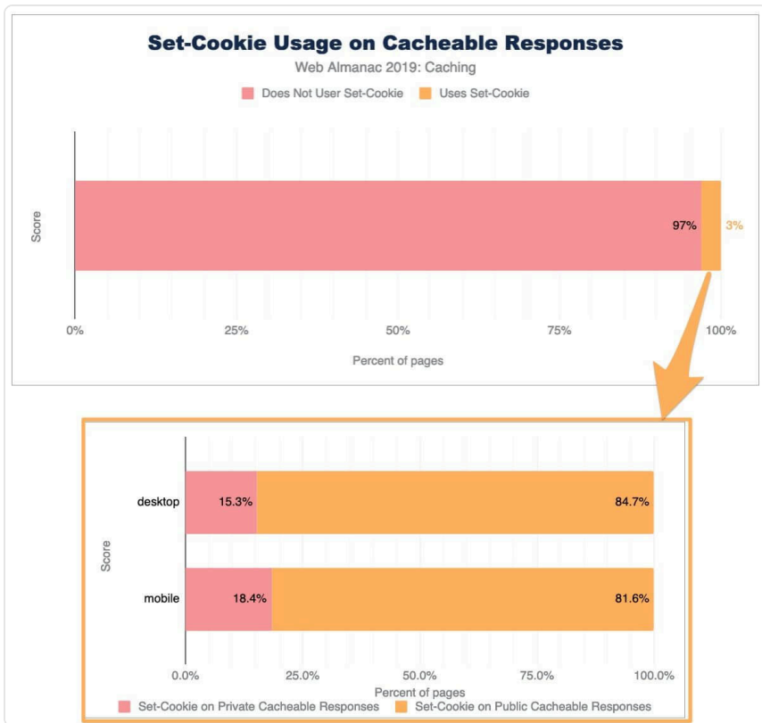
Figure 16.16. Cacheable responses of Set-Cookie responses.
