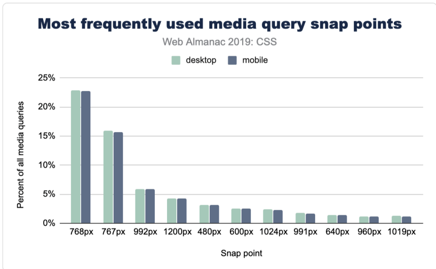
Figure 2.28. Most frequently used snap points used in media queries.
