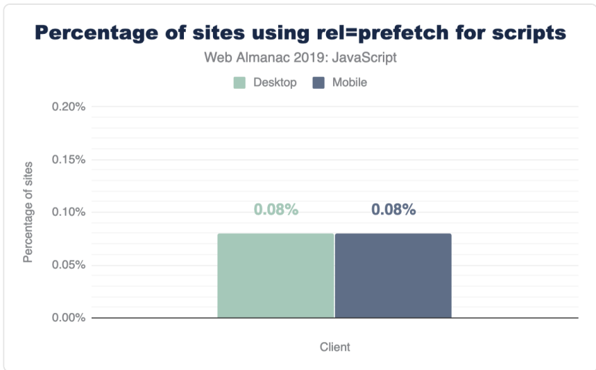
Figure 1.16. Percentage of sites using rel=prefetch for scripts.
