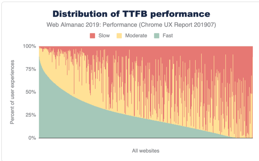
Figure 7.9. Distribution of websites' fast, moderate, and slow TTFB performance.
