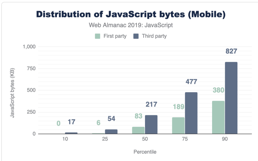
Figure 1.9. Distribution of total JavaScript downloaded on mobile.
