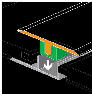
Insert the top profile into the base
