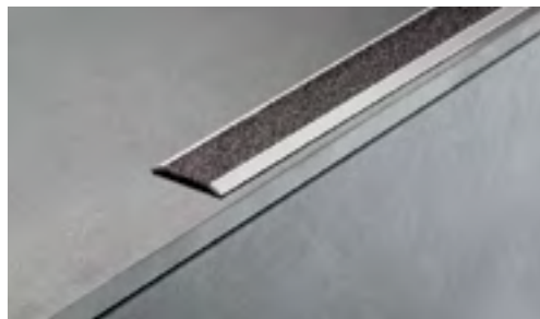
110/F silver anodized aluminum + black slip-resistant insert
