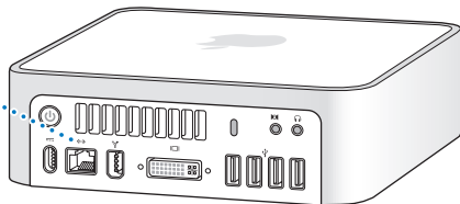
Ethernet-port (10/100/1000Base-T)
