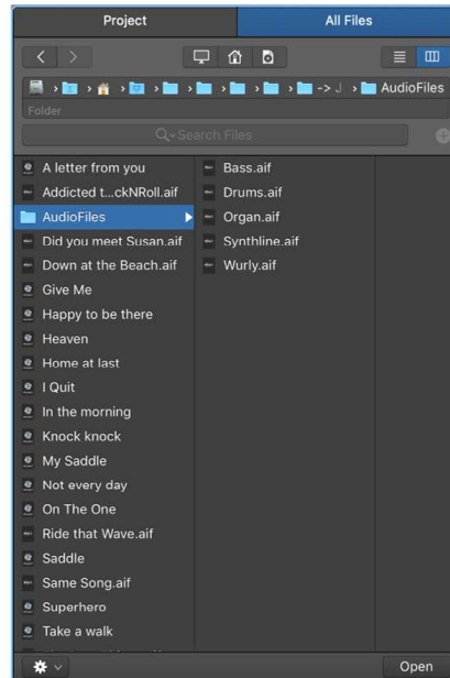
Column View
