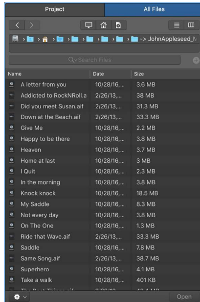
List View
