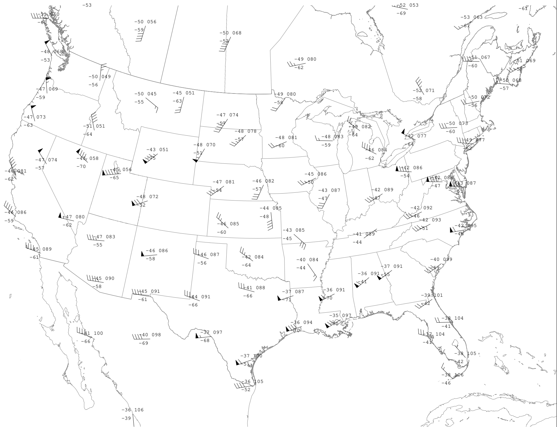
250 mb Observations Valid 240913/0000 UTC College of DuPage NEXLAB
