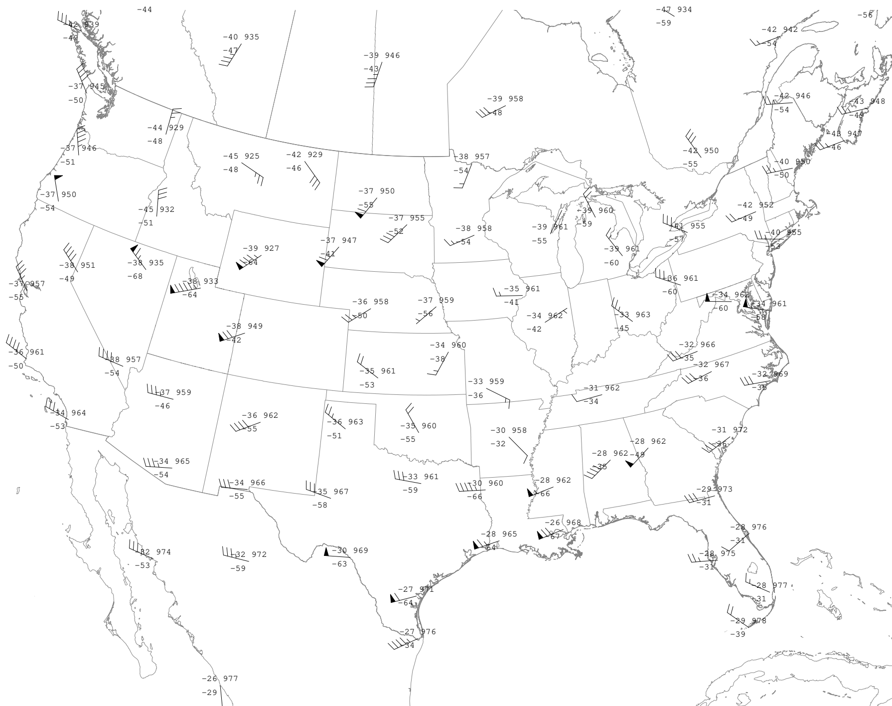
300 mb Observations Valid 240913/0000 UTC College of DuPage NEXLAB
