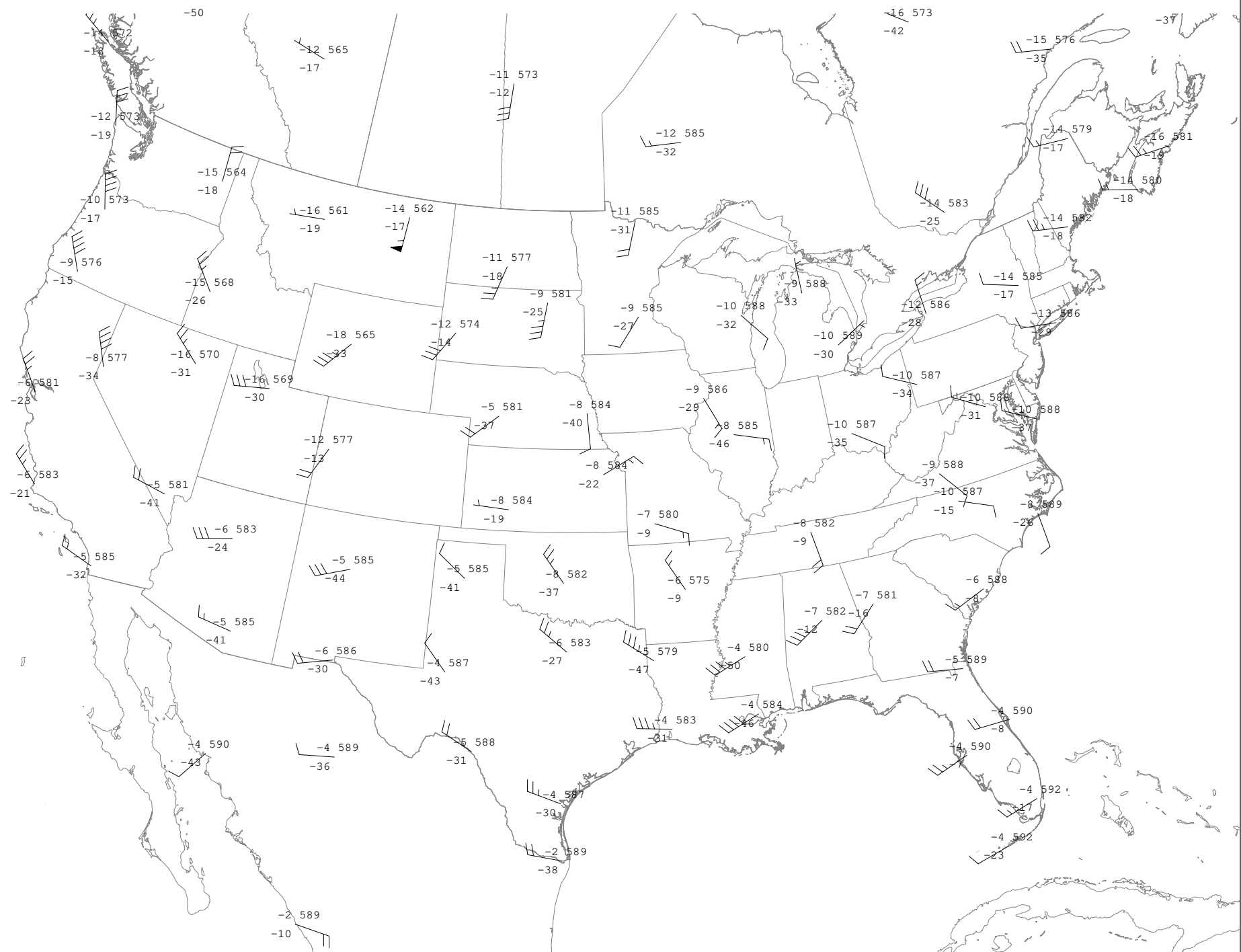
500 mb Observations Valid 240913/0000 UTC College of DuPage NEXLAB
