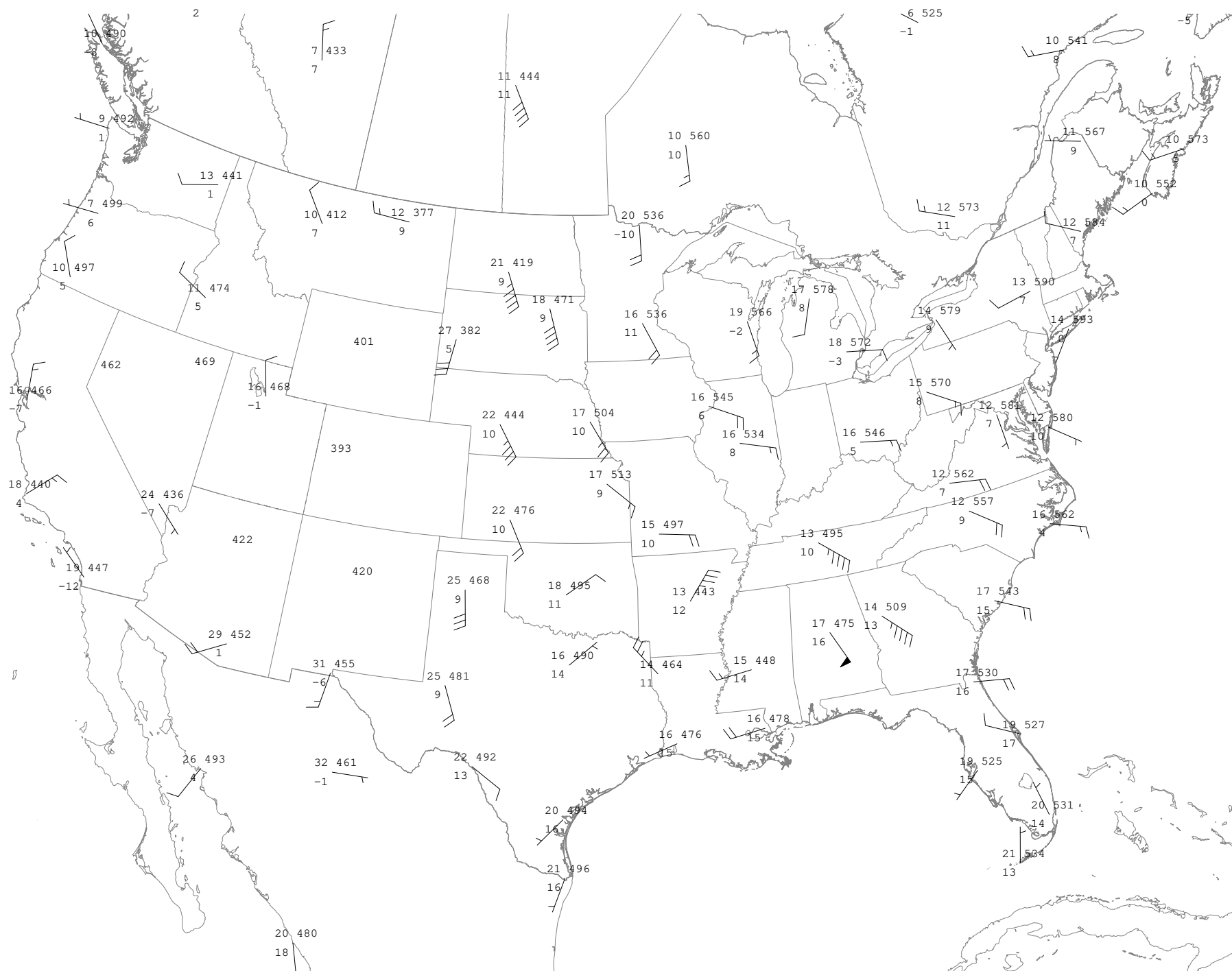
850 mb Observations Valid 240913/0000 UTC College of DuPage NEXLAB
