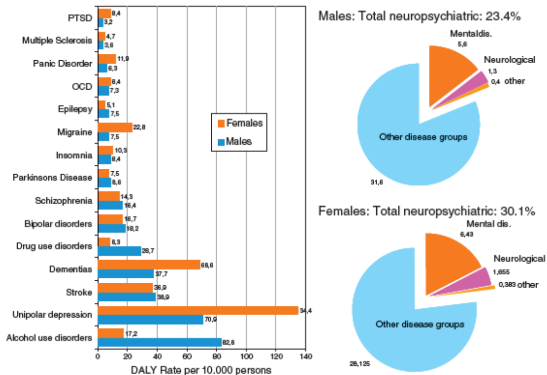
Fig. 2 Summary of DALY estimates.
