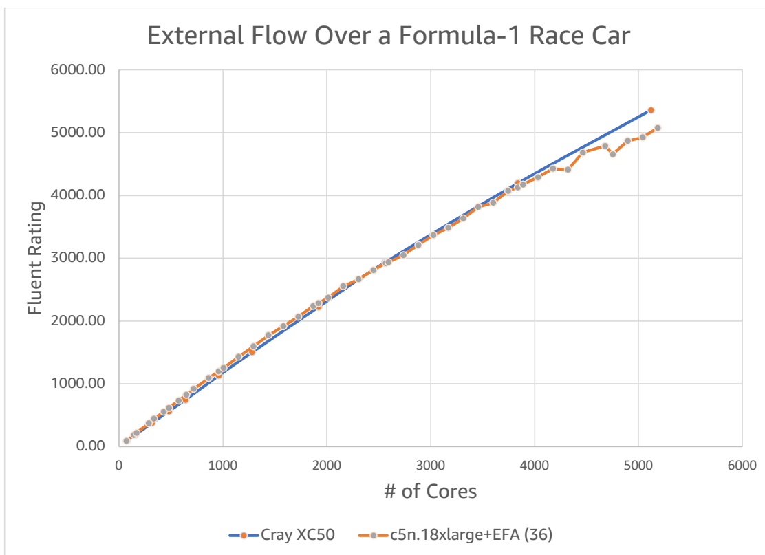
The plot shows C5n.18xlarge with EFA got a higher rating up to 2,400 cores and is essentially on par up to about 3,800 cores.
