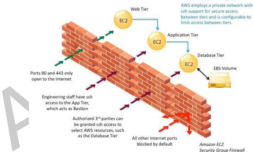
Figure 3: Amazon EC2 security group firewall
