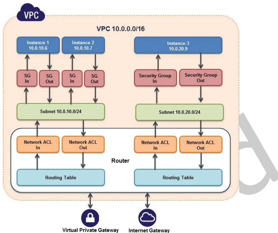
Figure 5: Flexible network topologies
