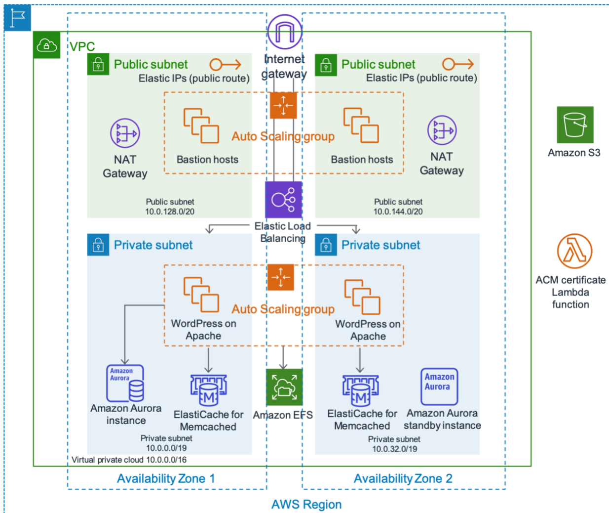
WordPress high availability architecture by Bitnami
